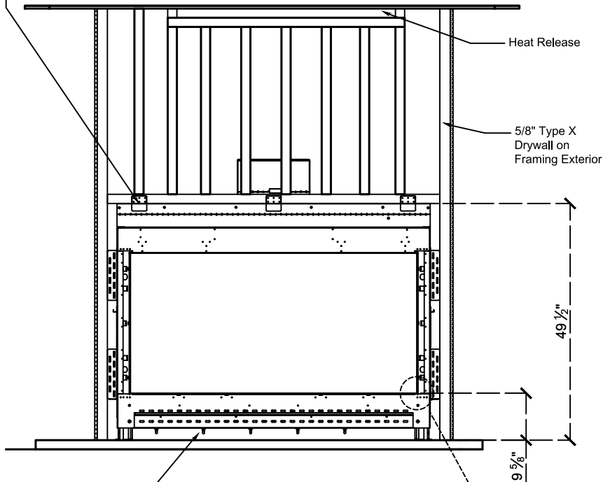
Elevation View
