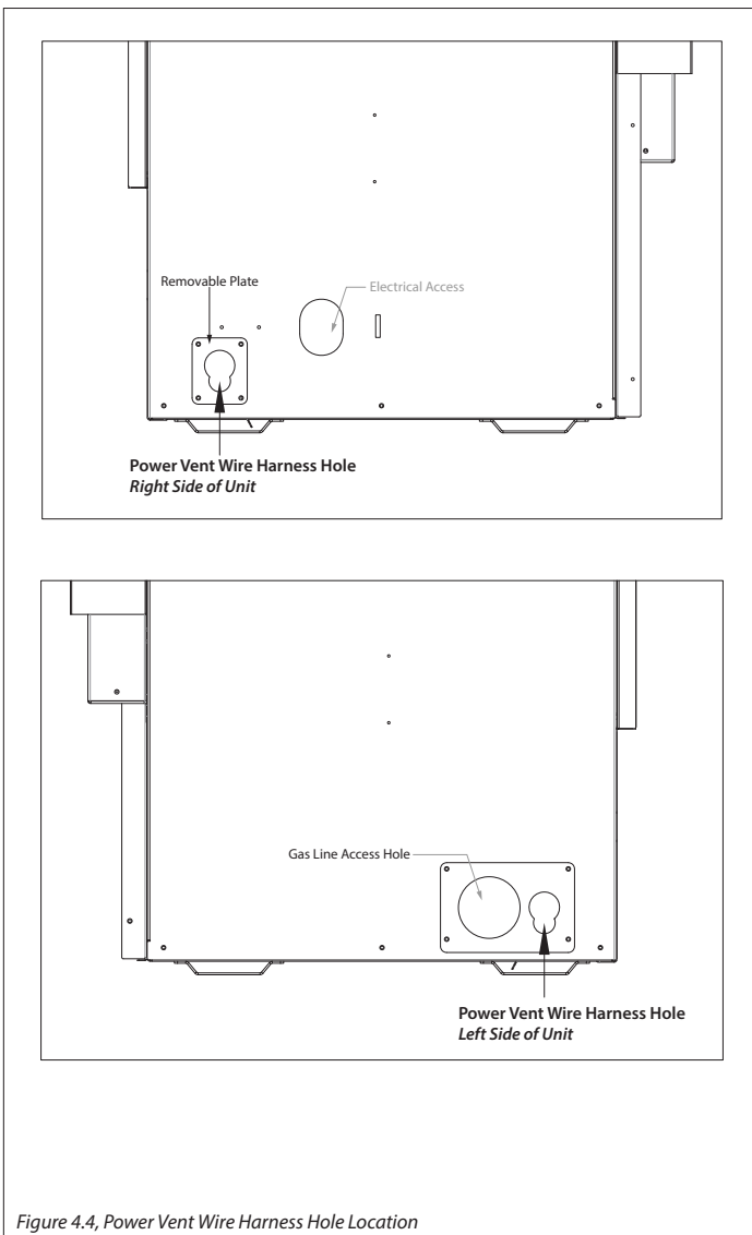
Figure 4.4, Power Vent Wire Harness Hole Location
