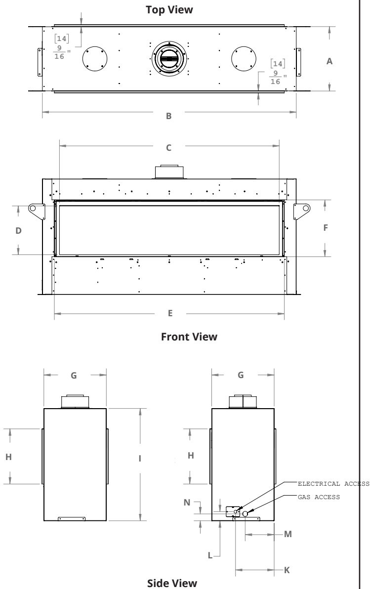
Figure 2.b DL6315ST, D6315ST Fireplace dimensions (Tolerance \pm 1/8" ).
