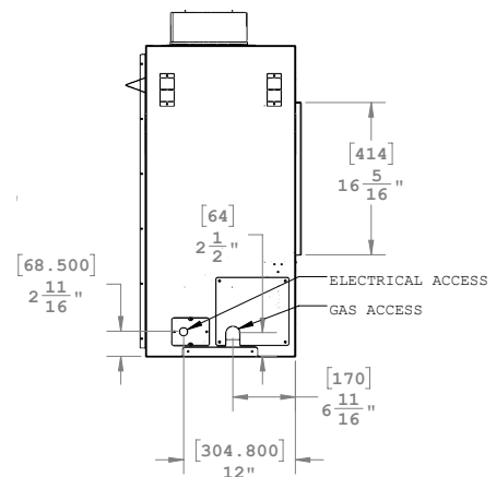
Figure 18. Gas Inlet Supply location
