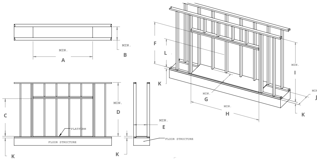
Figure 5. Back framing the Single Sided Fireplace
