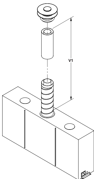
Figure 8. Vertical Termination
