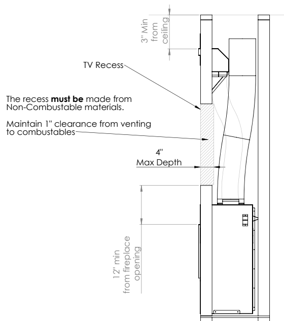
Figure 8.b.d Cool Wall Advantage TV recess dimensions
