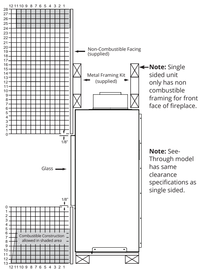
Figure 19. Combustible mantles and facings. (Not to scale)
