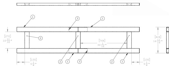
Figure 8. Assembly of Non Combustible Framing
