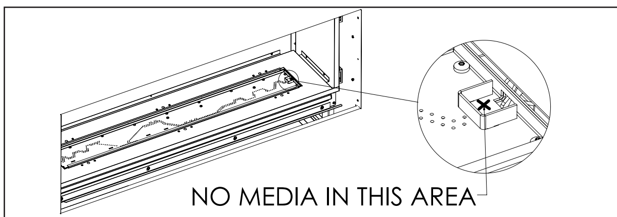
Figure 48: Protected Pilot Area
