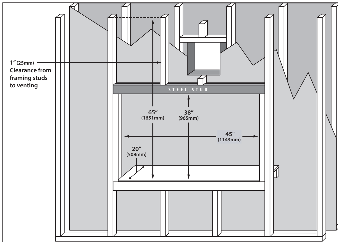
Figure 18: Framing Dimensions
