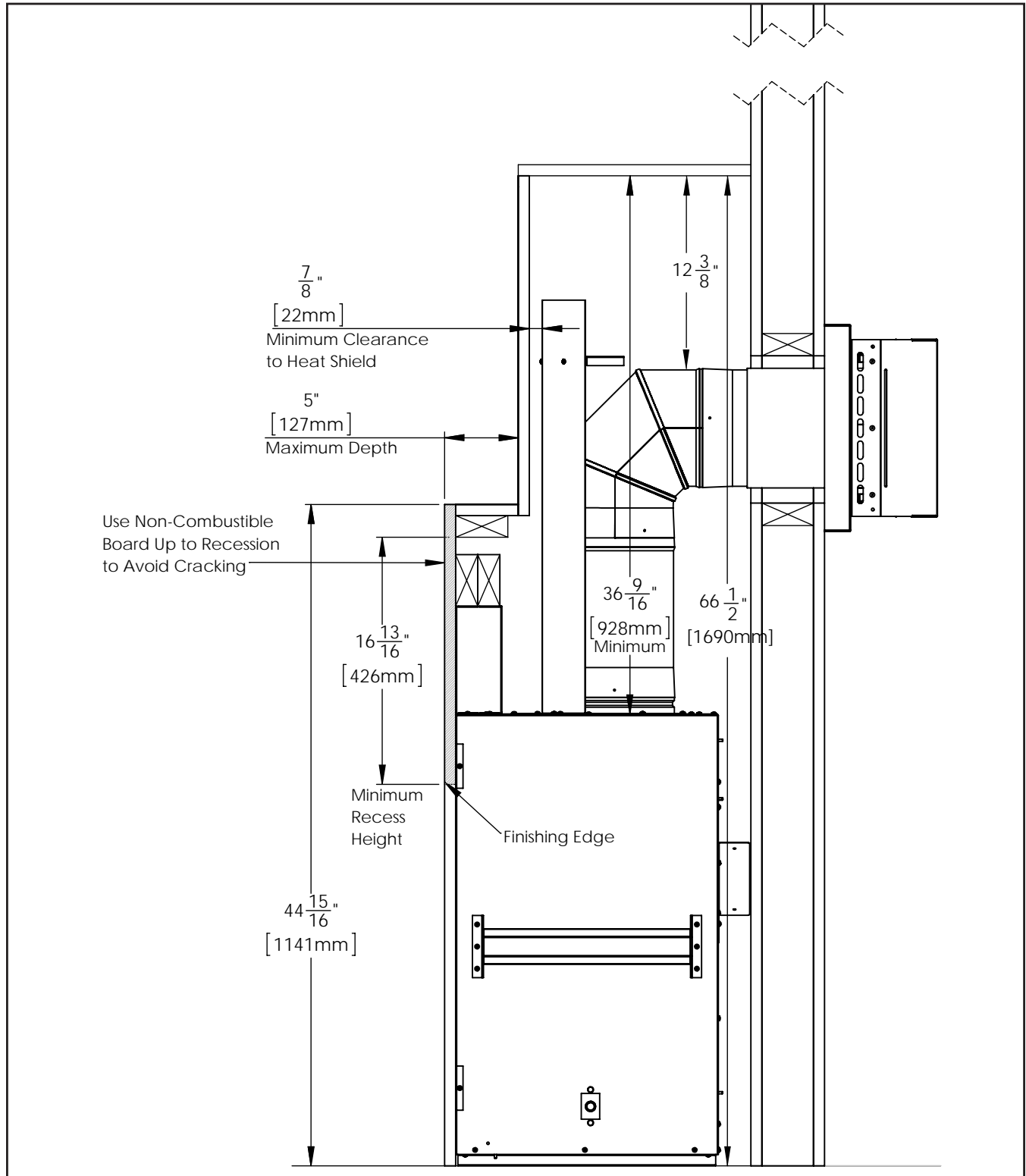
Figure 22: Install Dimensions with Recess
