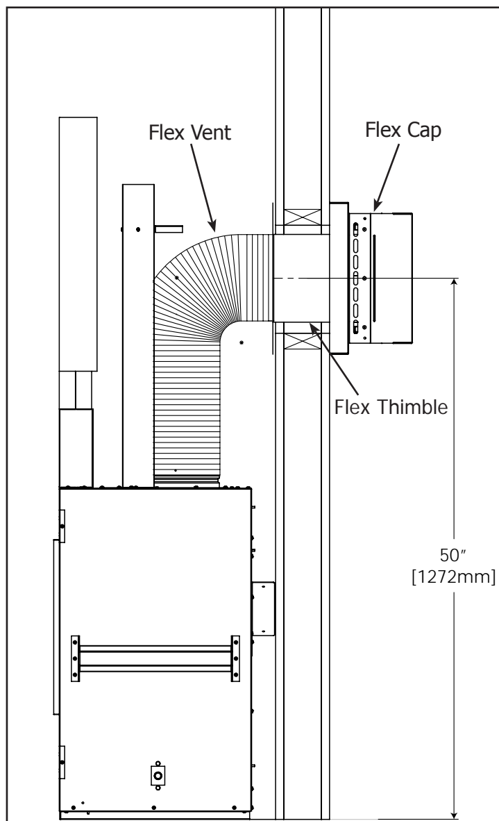
Figure 26. Flex Vent Minimum Install
