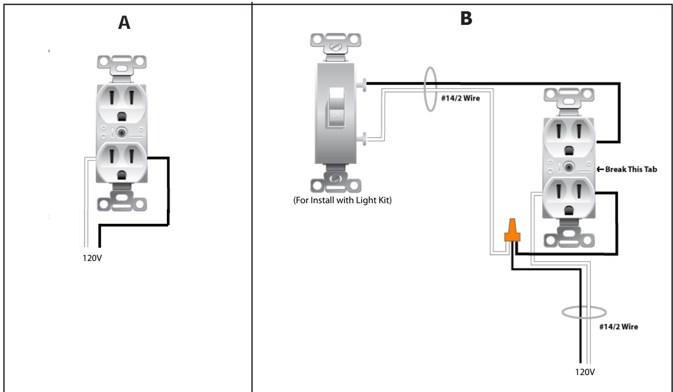
Figure 44: C34 Receptacle Wiring
