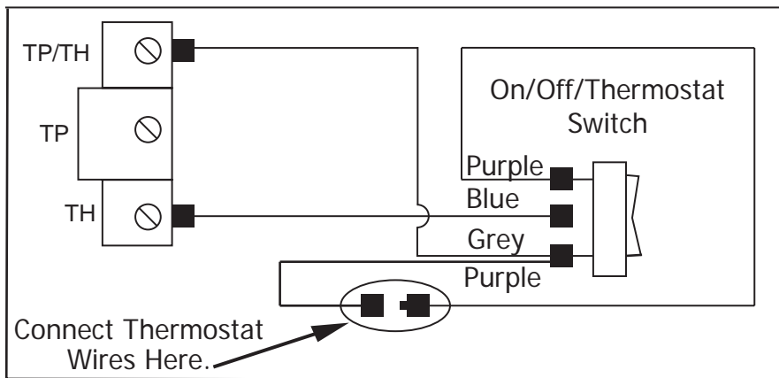
Figure 42: C34 Wiring Diagram
