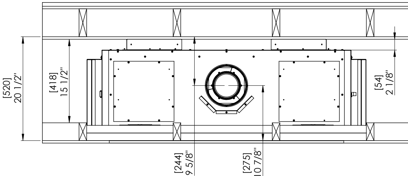
Figure 25(b). Dimensions for a Vertical Installation
