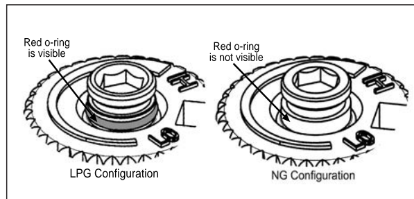
Figure 16: O-ring on valve screw.
