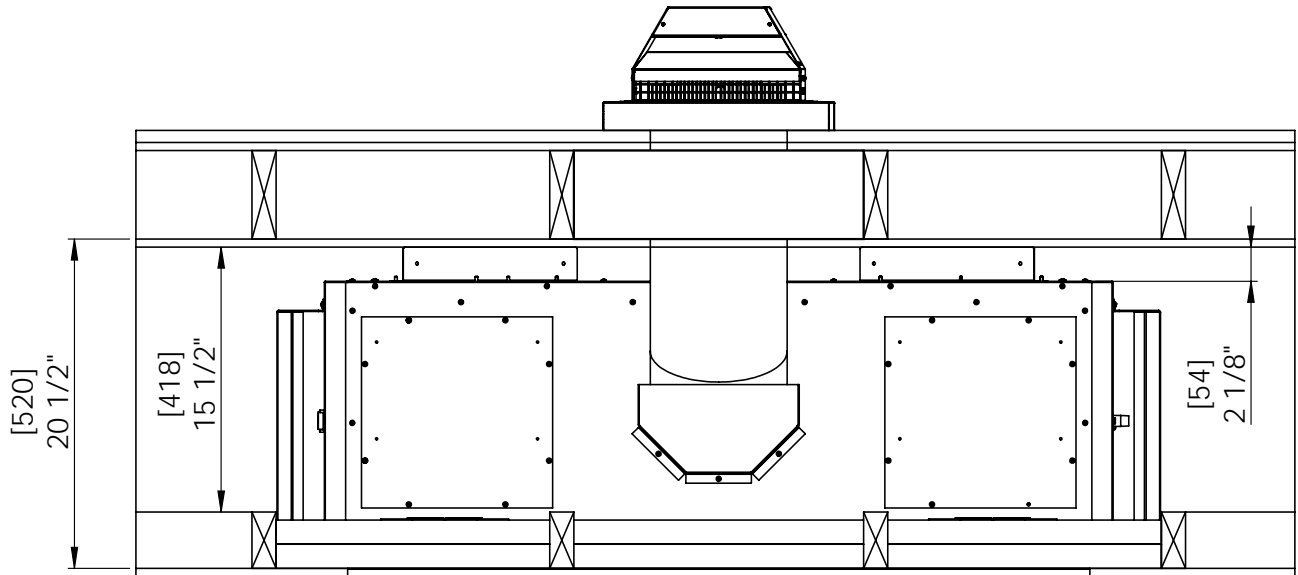
Figure 25(a). Dimensions for a Horizontal Installation
