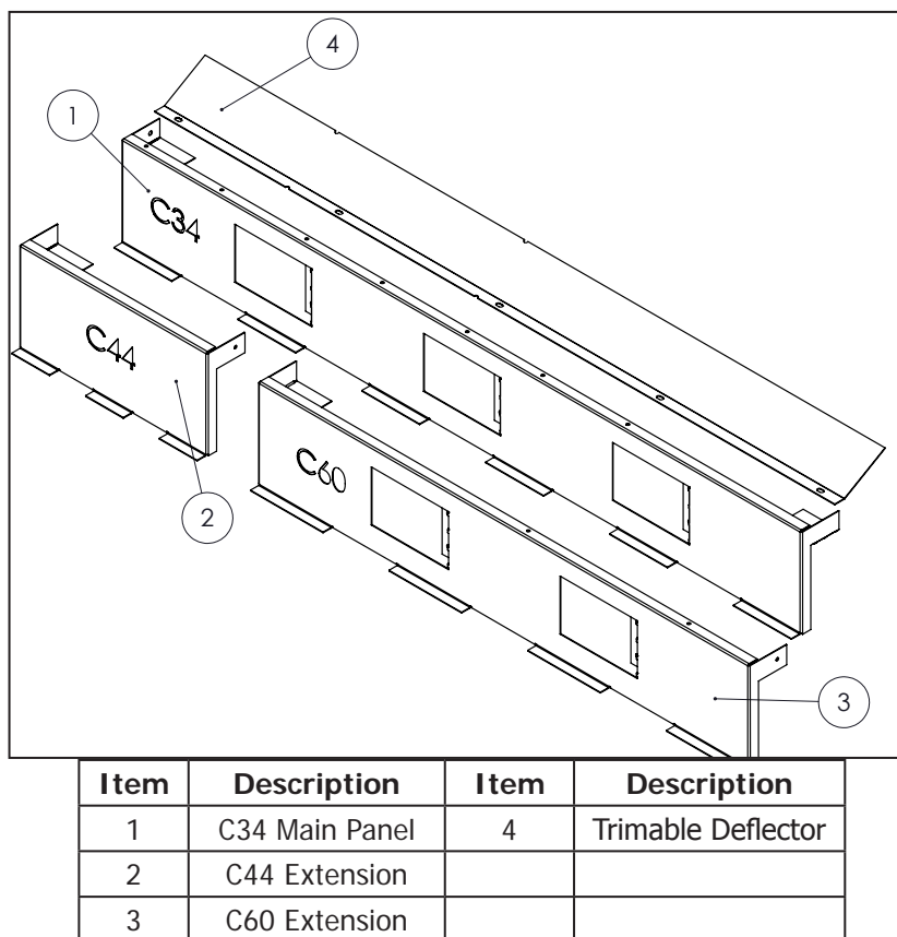
Figure 2. Cool Surface System Combustible Facing Kit - Parts Diagram
