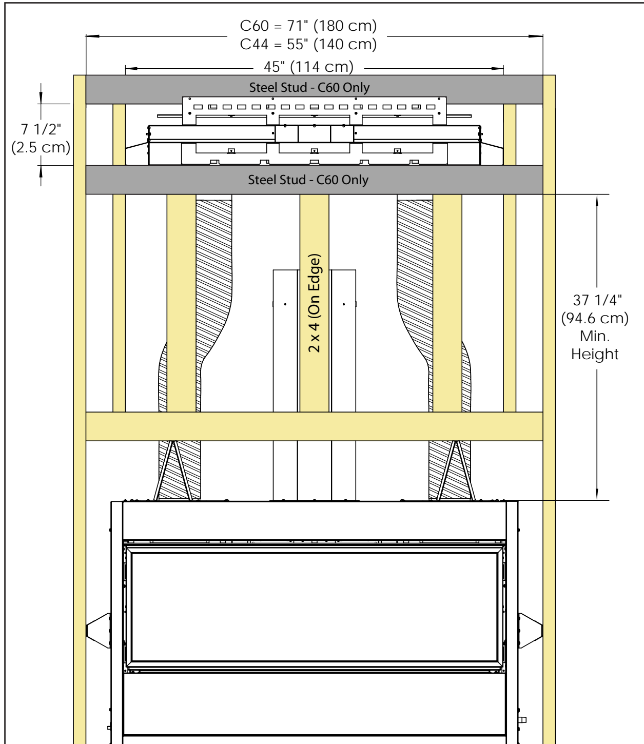
Figure 6. C44/60 - CSS Framing & Rough Opening
