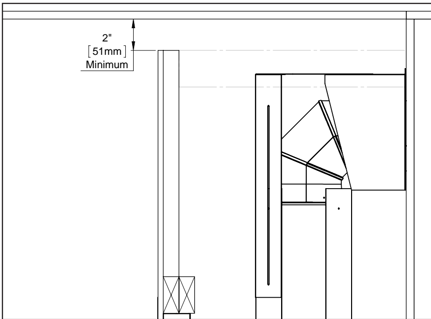
Figure 28: Open Chase
