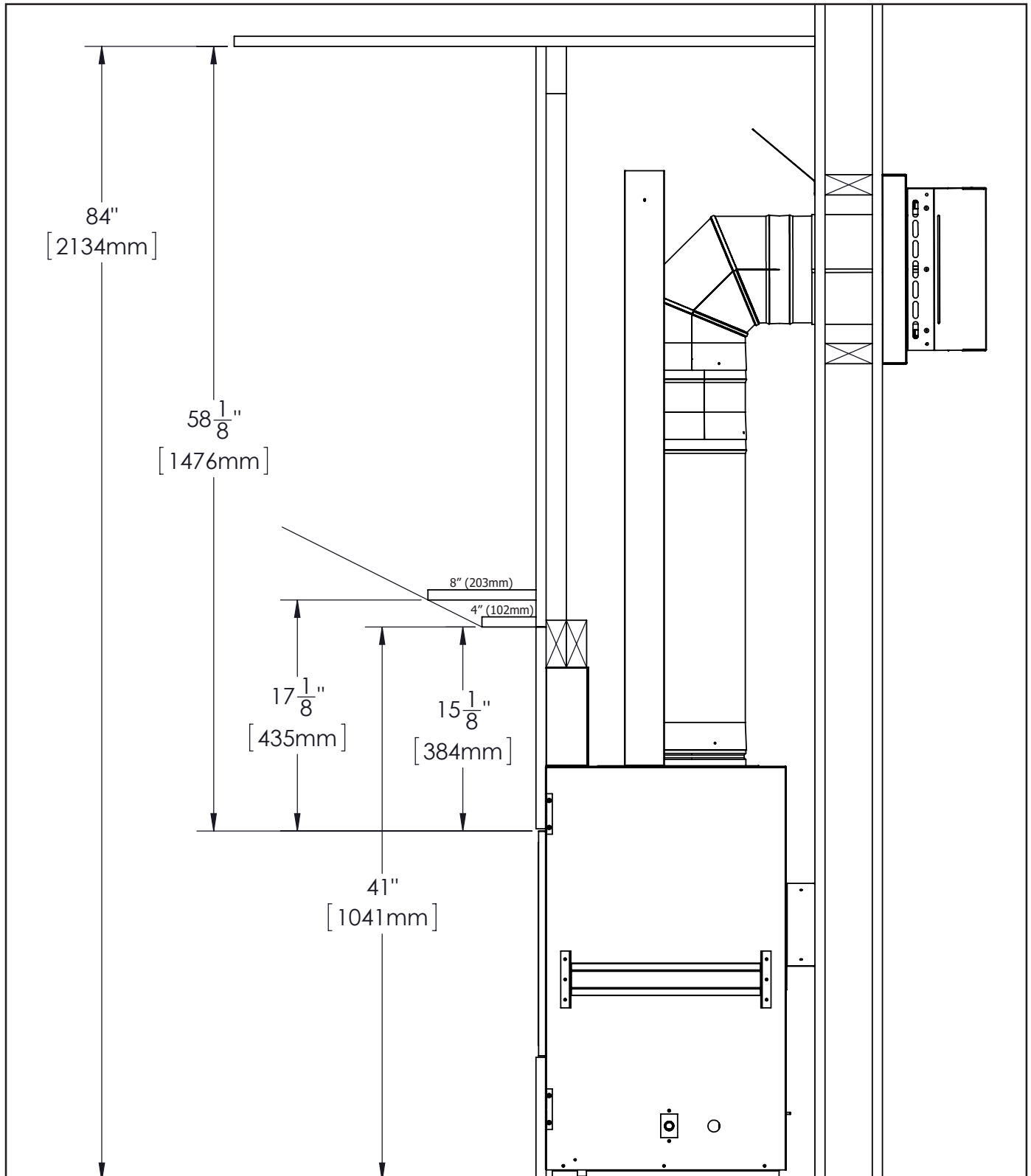
Figure 35(c): Install Dimensions with Mantel
