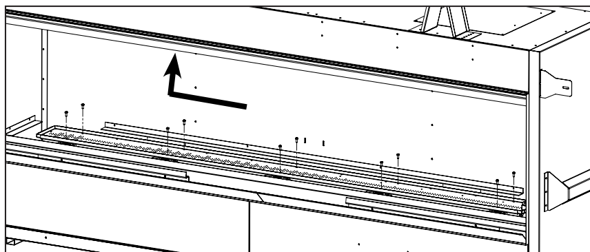
Figure 6. Removing Burner
