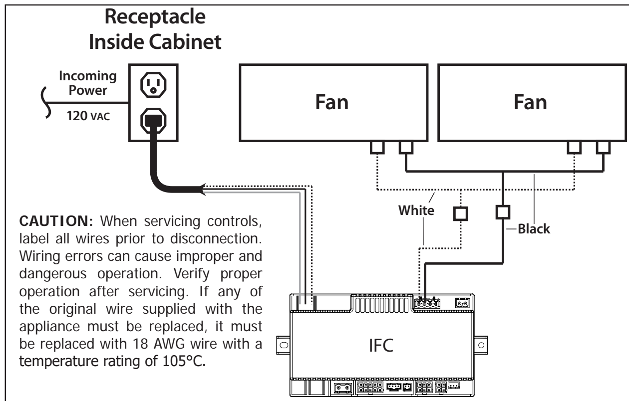
Figure 58: Fan Kit Wiring Diagram
