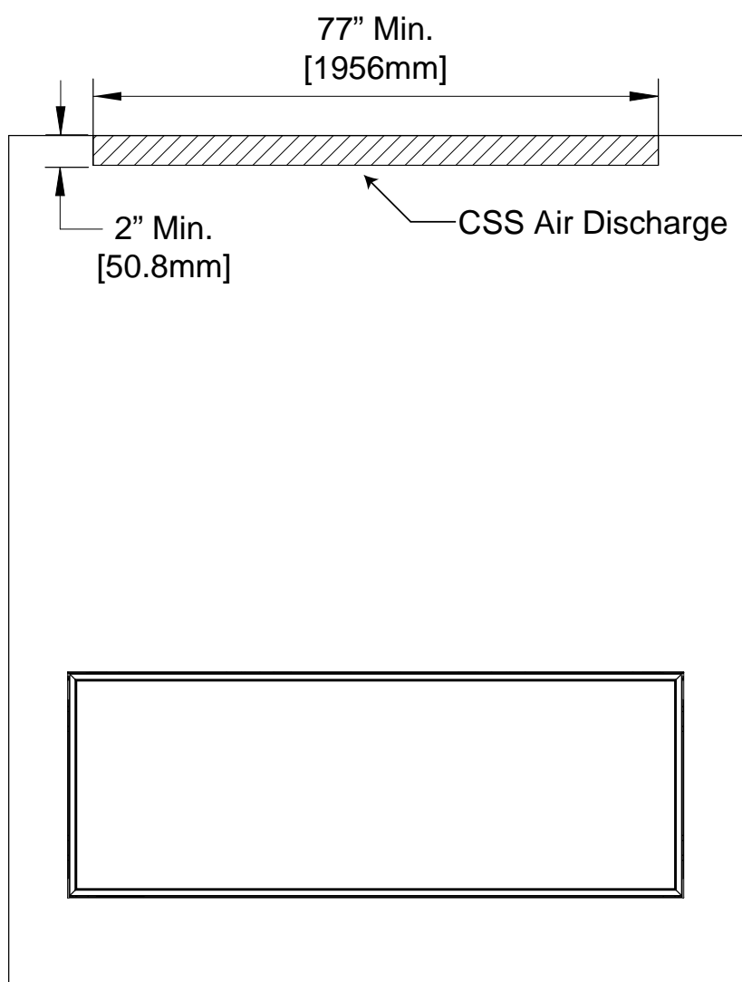
Figure 24 CSS Outlet
