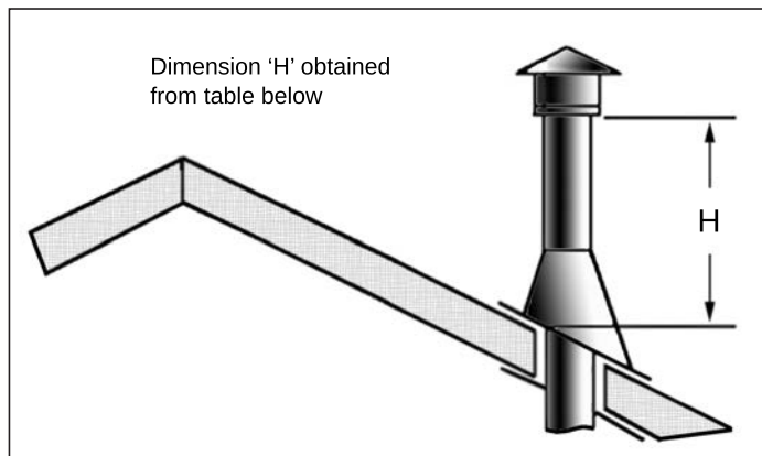
Figure 50(b): Height of Vertical Termination; Reference Table 8
