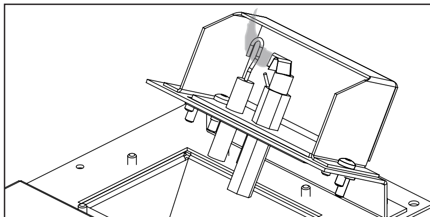
Figure 12: Flame Sensor Coverage
