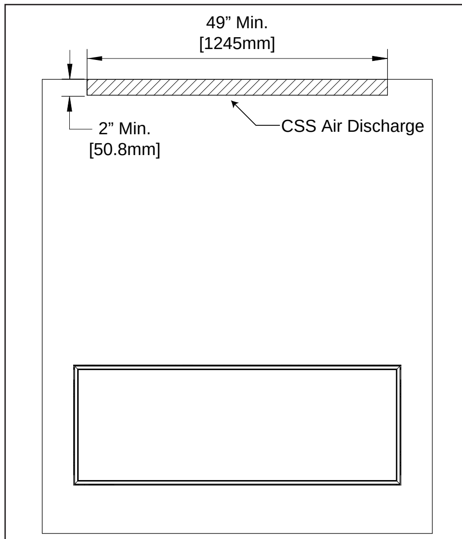
Figure 24 CSS Outlet
