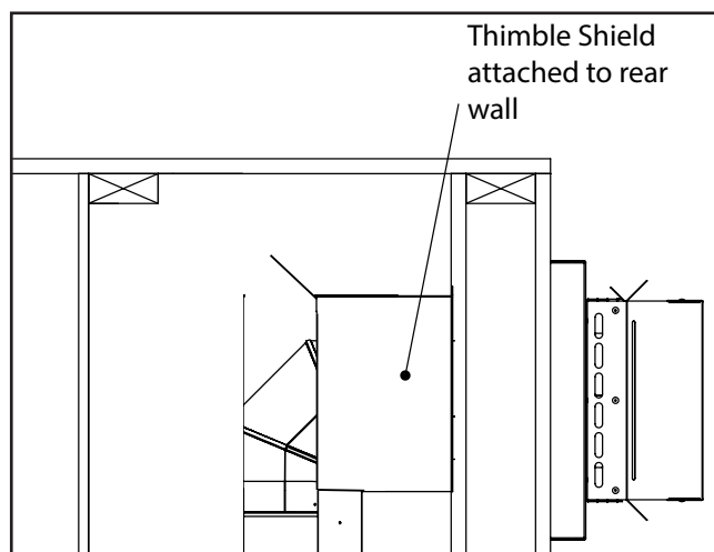
Figure 30: CSS Heat Shield
