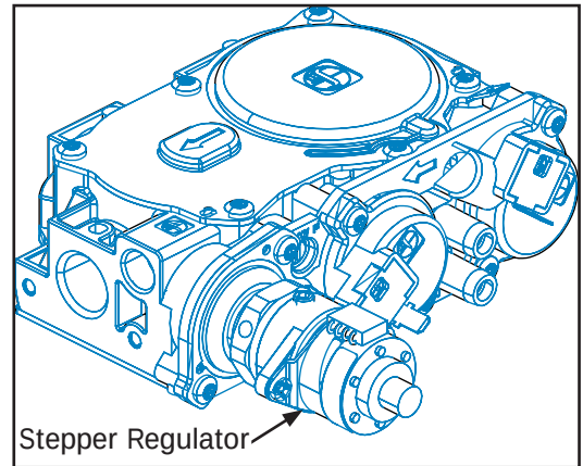
Figure 11: 885 Gas Valve
