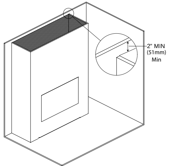
Figure 29: Open Chase Iso View
