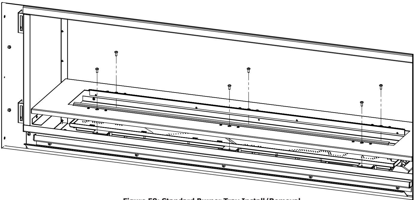
Figure 58: Standard Burner Tray Install/Removal
