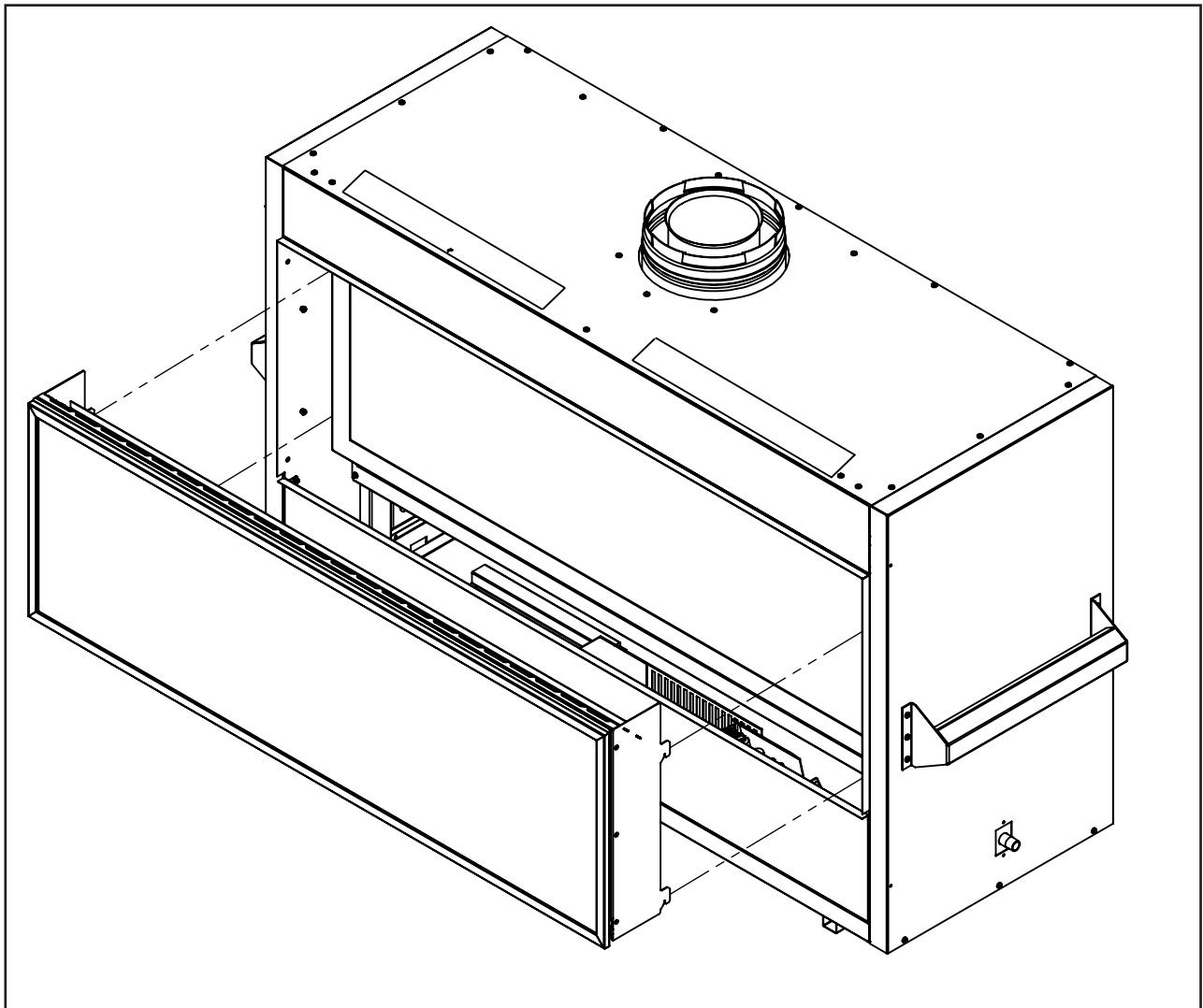
Figure 4: Safety Screen Removal
