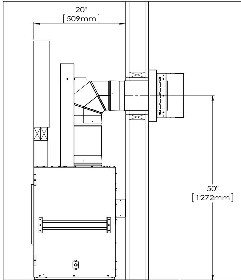
Figure 34: Minimum Horizontal Venting
