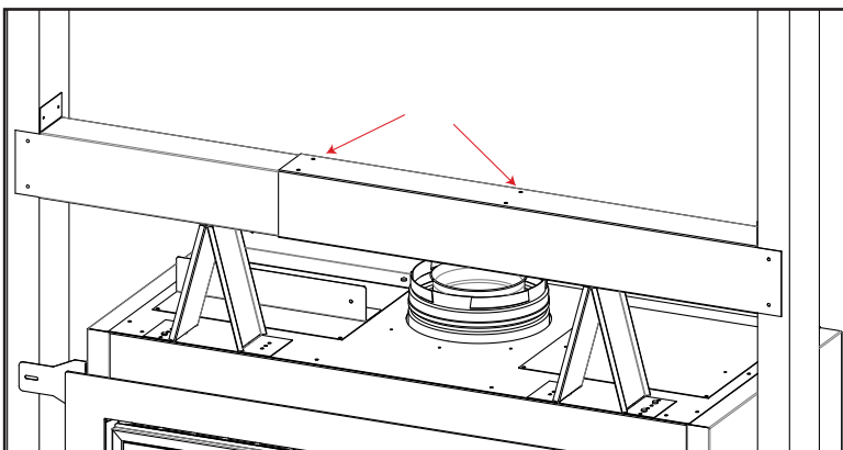
Figure 16: Steel Stud Installation
