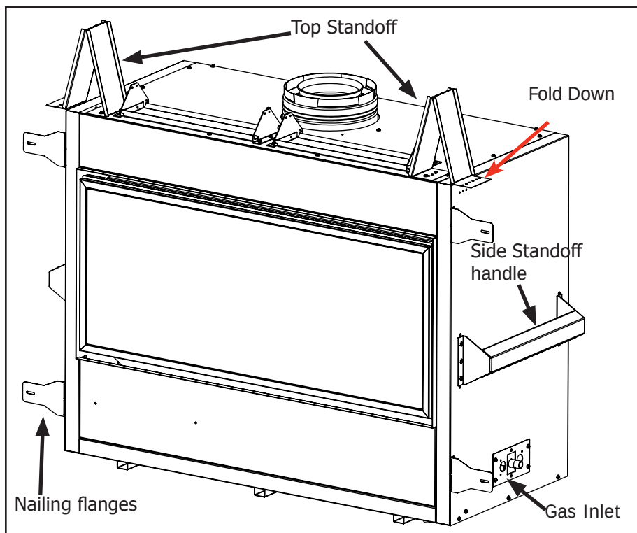
Figure 13: Fireplace Install Prep
