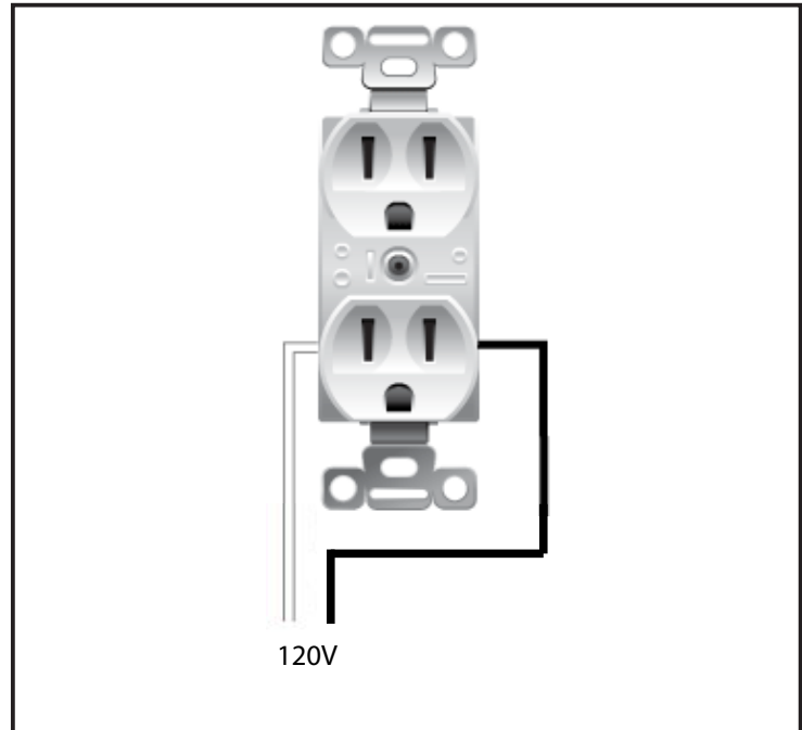
Figure 55: C44I Receptacle Wiring
