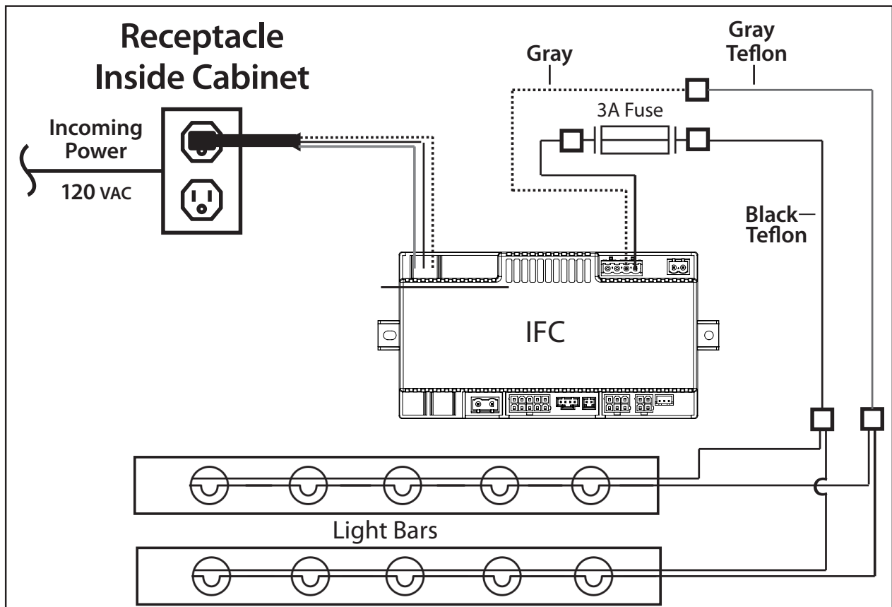
Figure 57: Light Kit Wiring Diagram
