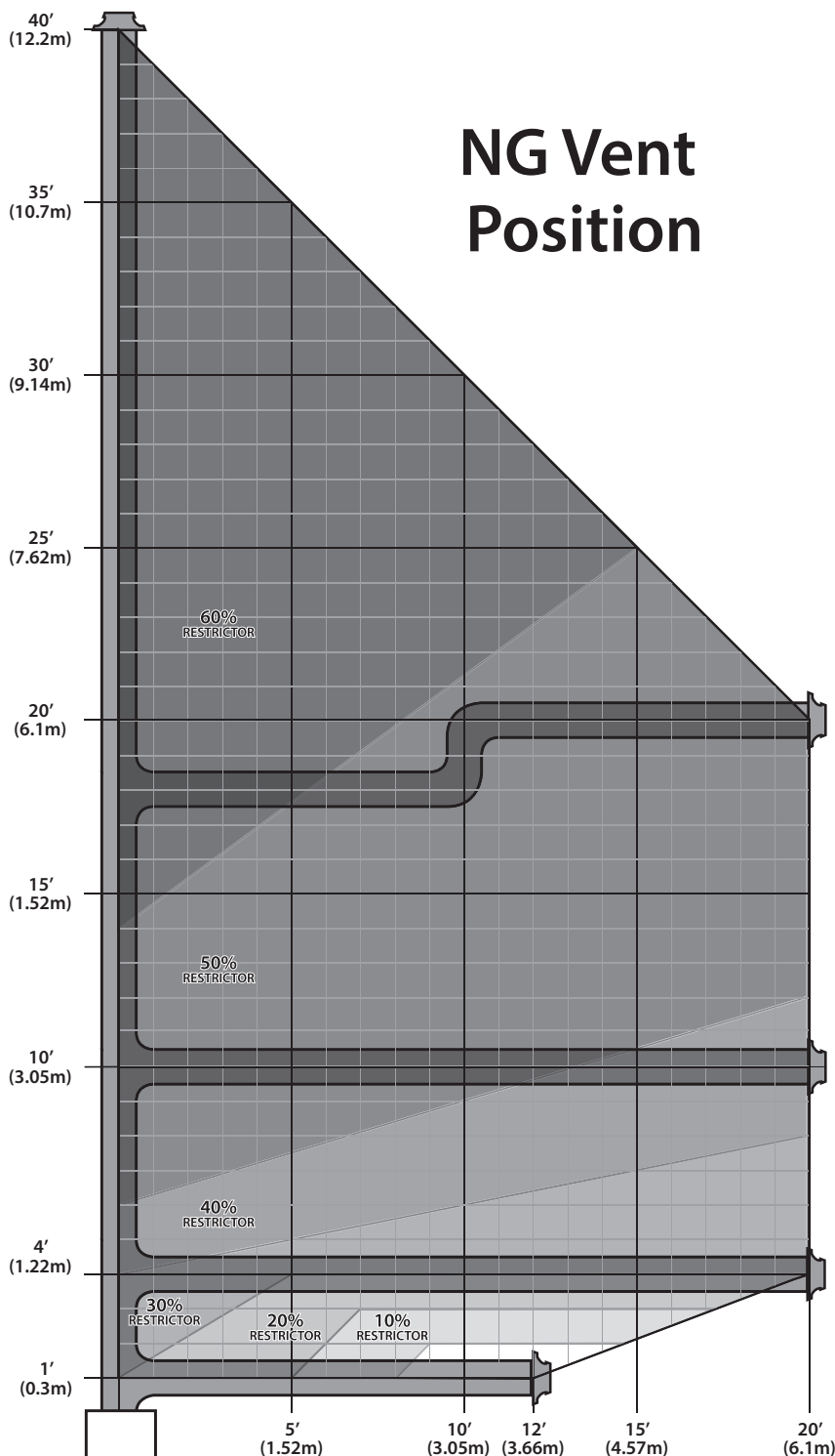
Figure 45. Natural Gas Vent Graph **Vertical vent height does not account for elbows
