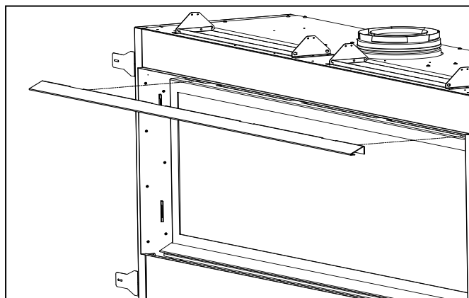
Figure 20 Discharge Accelerator removal
