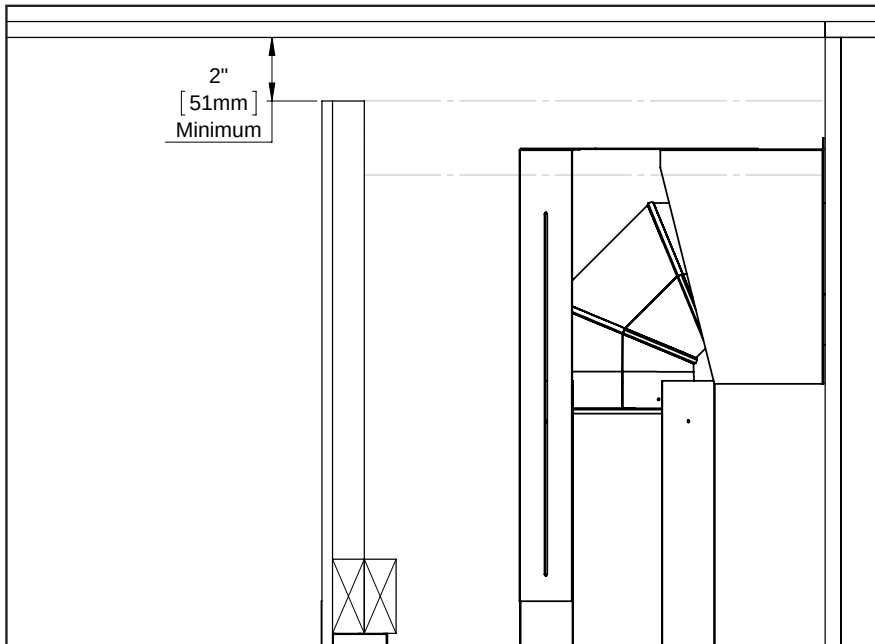
Figure 28: Open Chase
