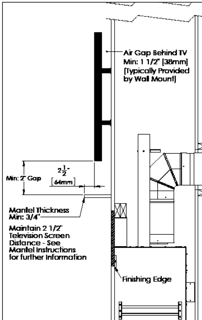
Figure 41. Minimum TV Install Clearances
