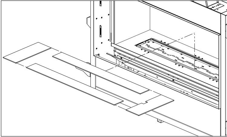
Figure 59: Burner Bezel Placement
