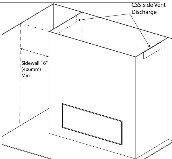
Figure 25 CSS Side Vent
