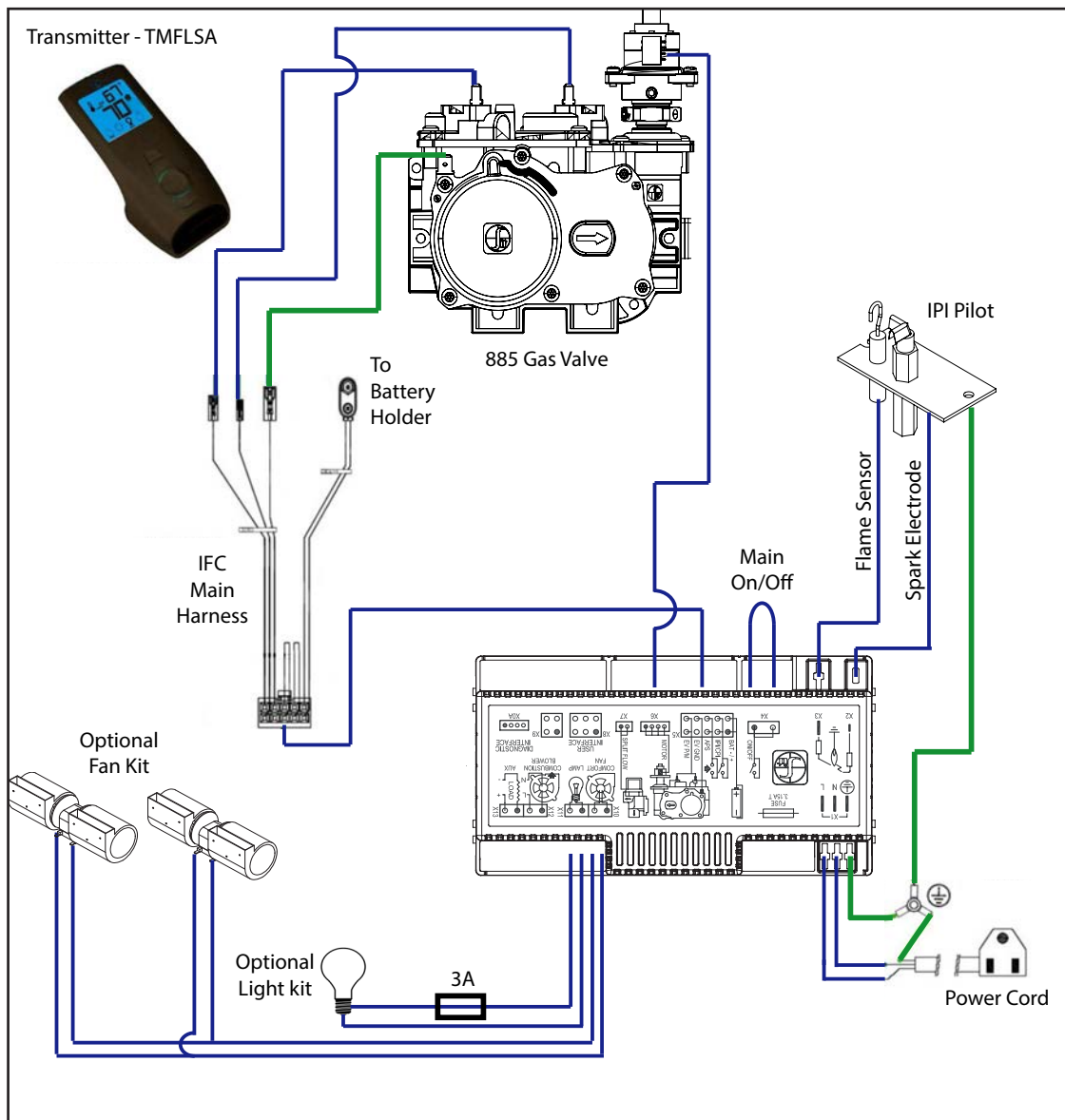
Figure 54: C44I Wiring Diagram
