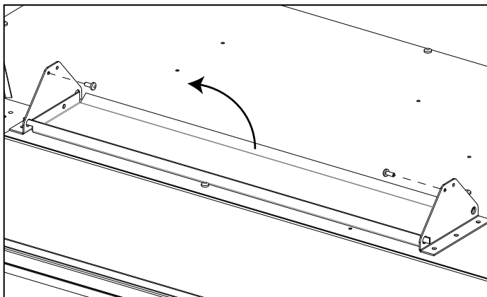
Figure 22 CSS flaps
