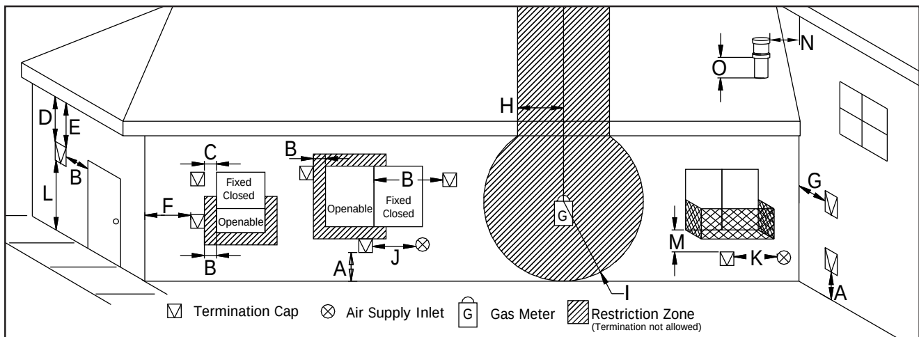
Figure 43. Vent Termination Restrictions, refer to Table 3
