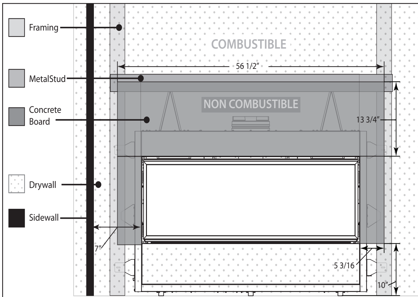
Figure 19. Finishing Non-Combustible Zone
