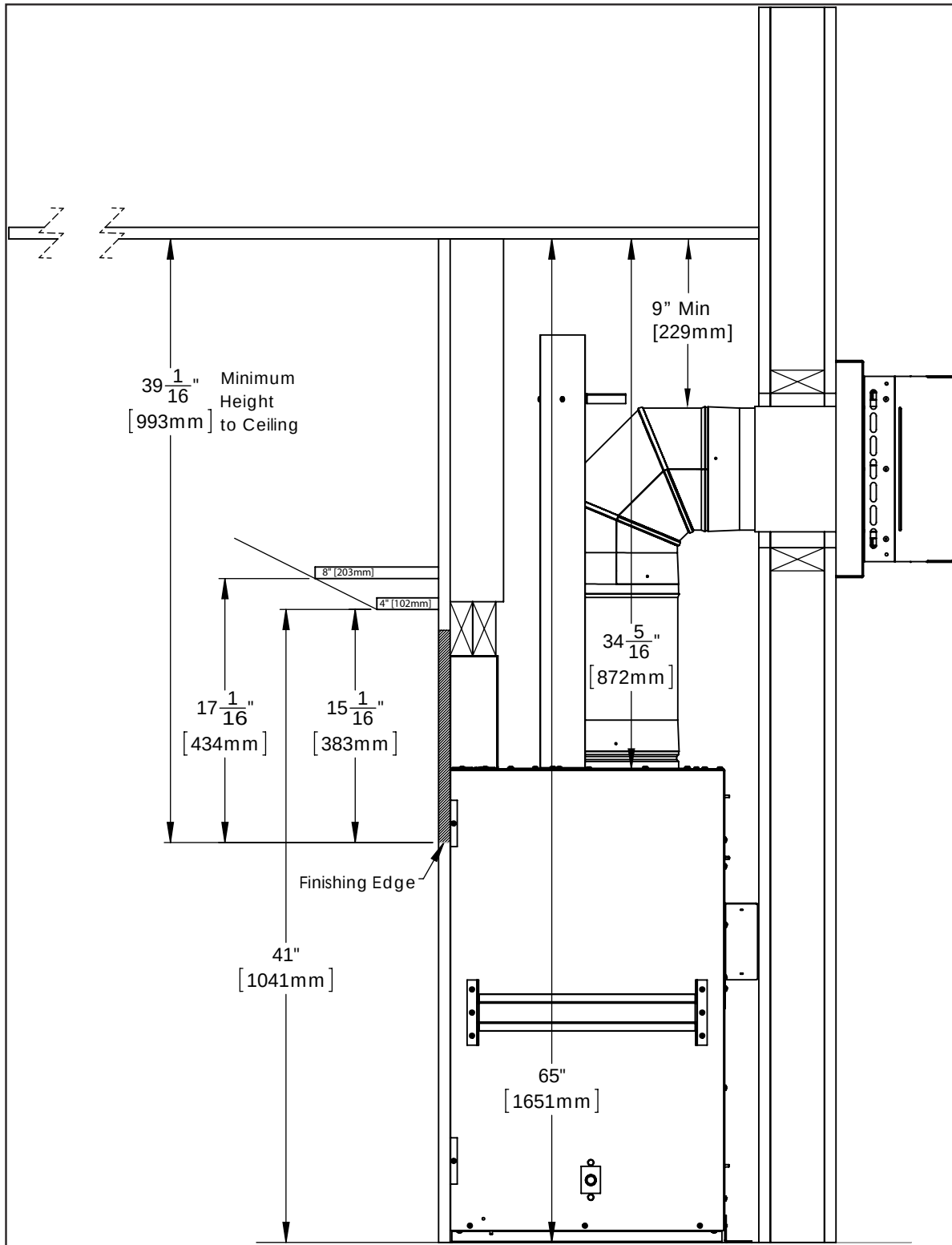
Figure 35(c): Install Dimensions with Mantel
