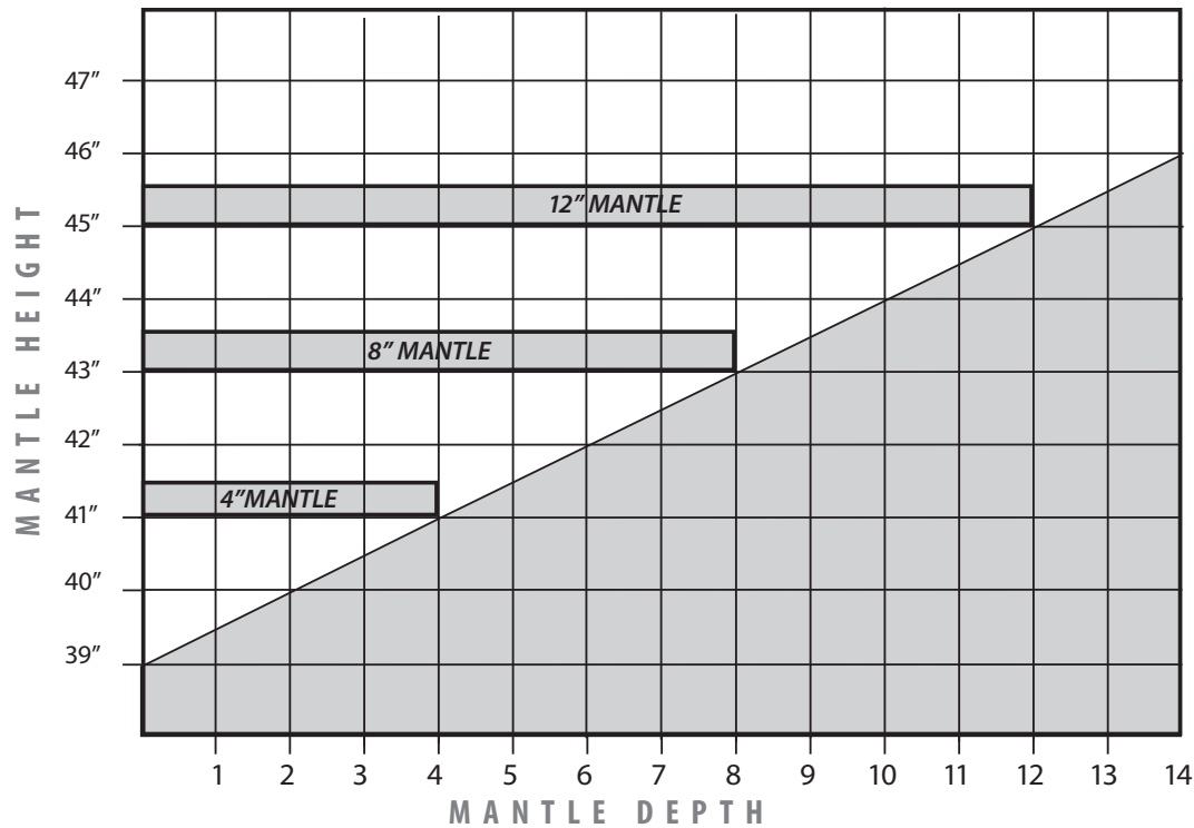
Figure 35(a): Minimum Mantel Height
