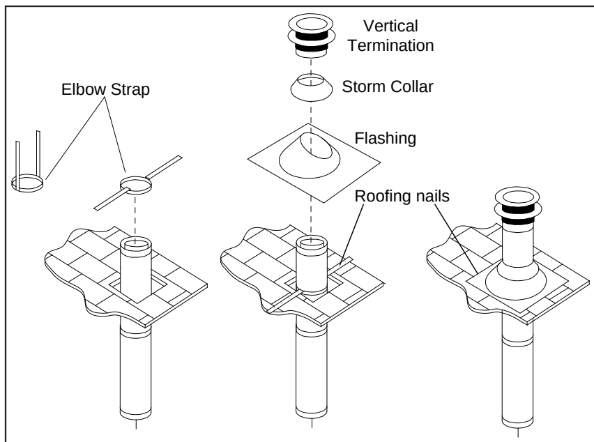
Figure 50(a). Vertical Vent Termination
