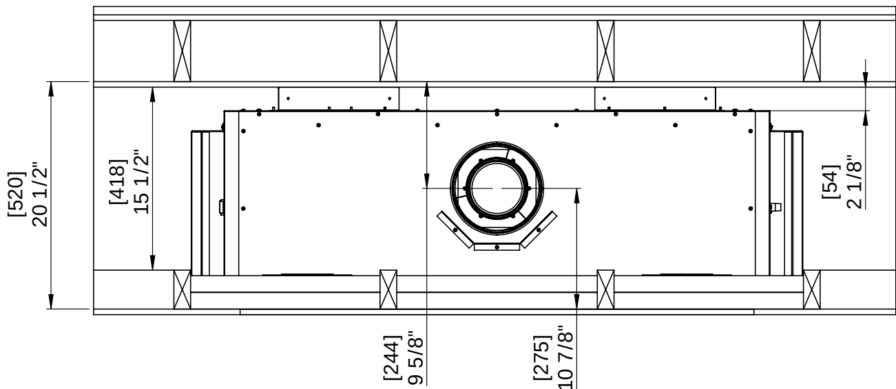
Figure 39(b). Dimensions for a Vertical Installation
