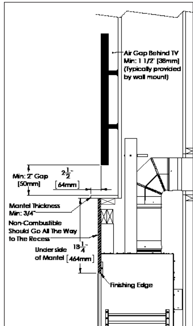
Figure 42. Recess Minimum TV Install Clearances
