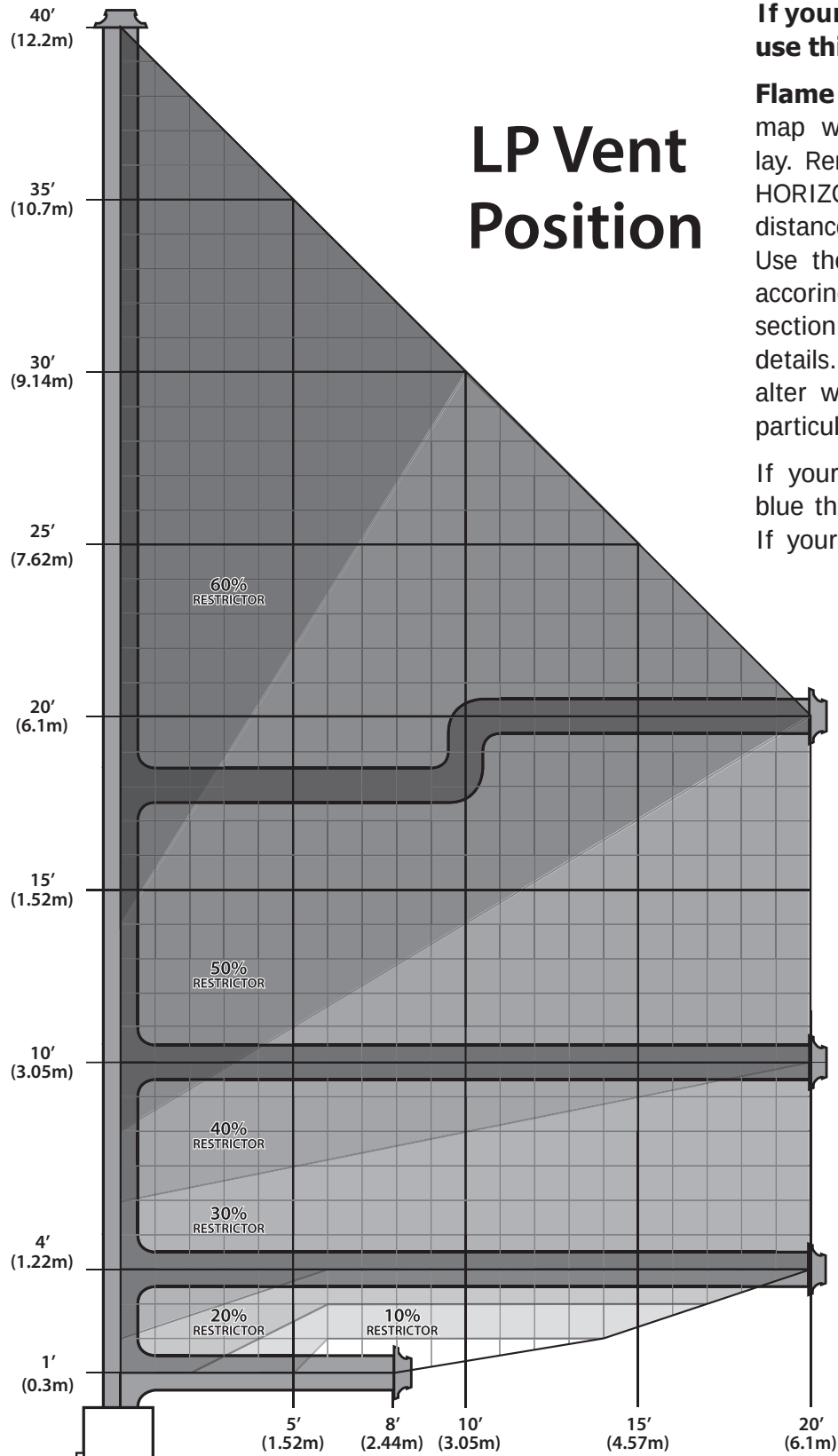
Figure 46. LP Vent Graph
