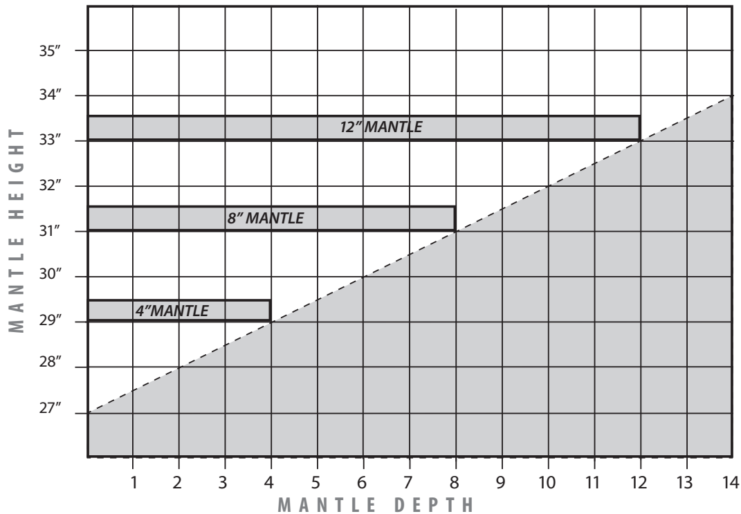
Figure 35(b): Minimum Mantel Height -- CSS Activated
