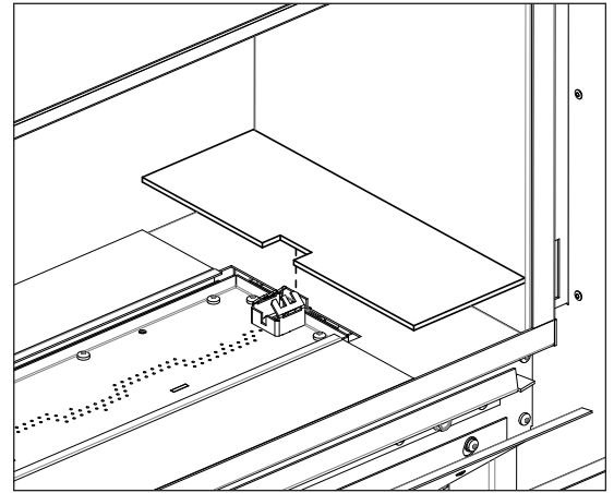
Figure 60: Bezel Placement Around Pilot
