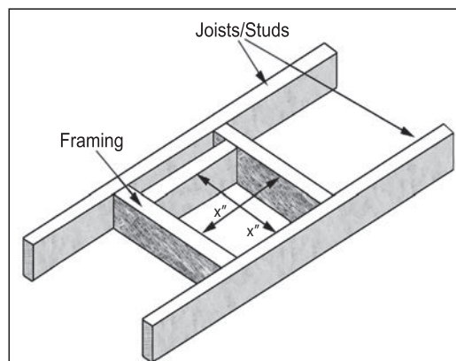
Figure 44. Vent Framing For Wall or Ceiling
