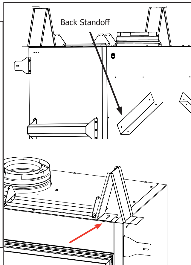
Figure 13: Fireplace Install Prep
