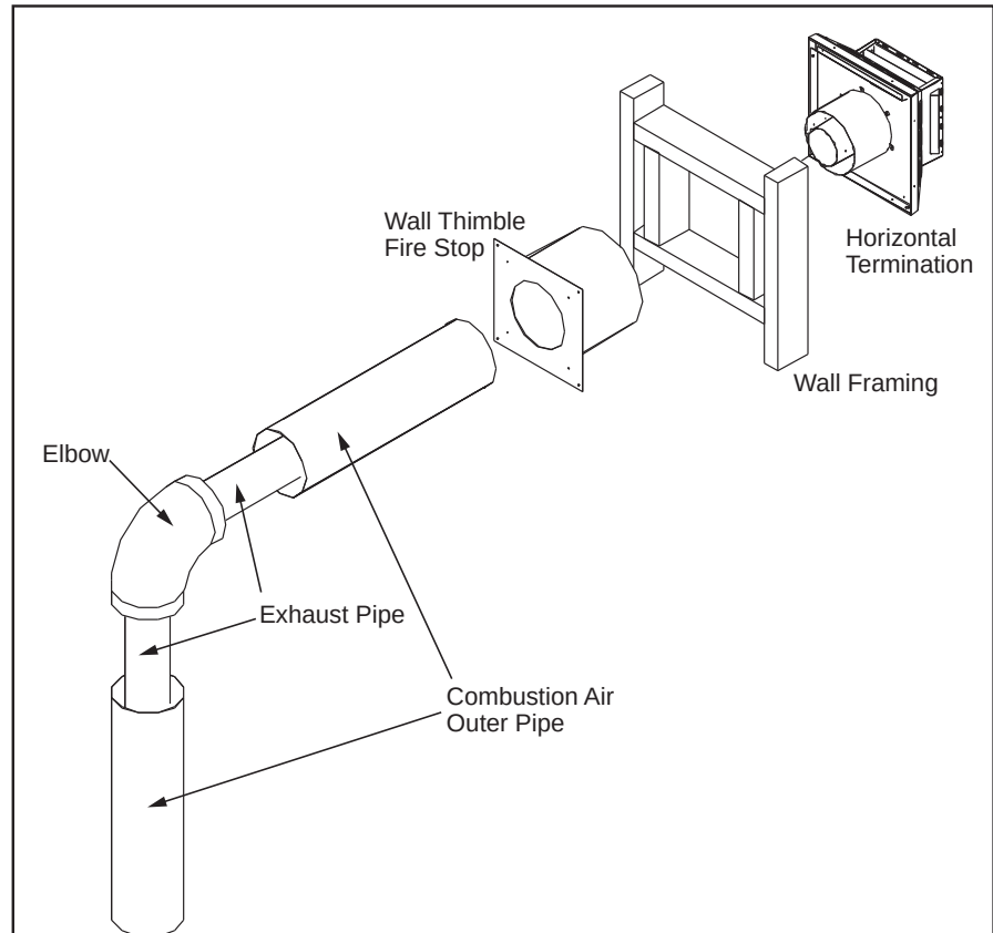
Figure 49. Horizontal Vent Termination
