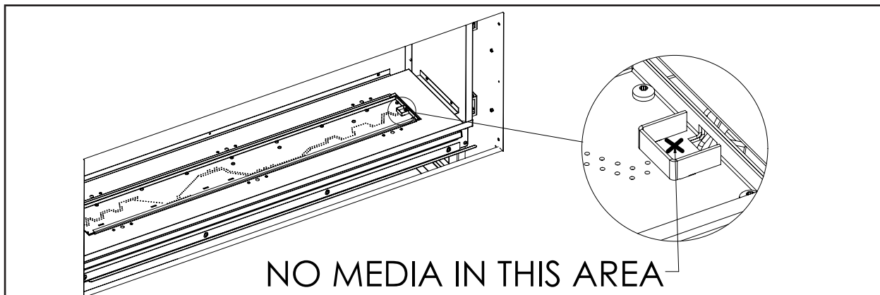
Figure 59: Protected Pilot Area
