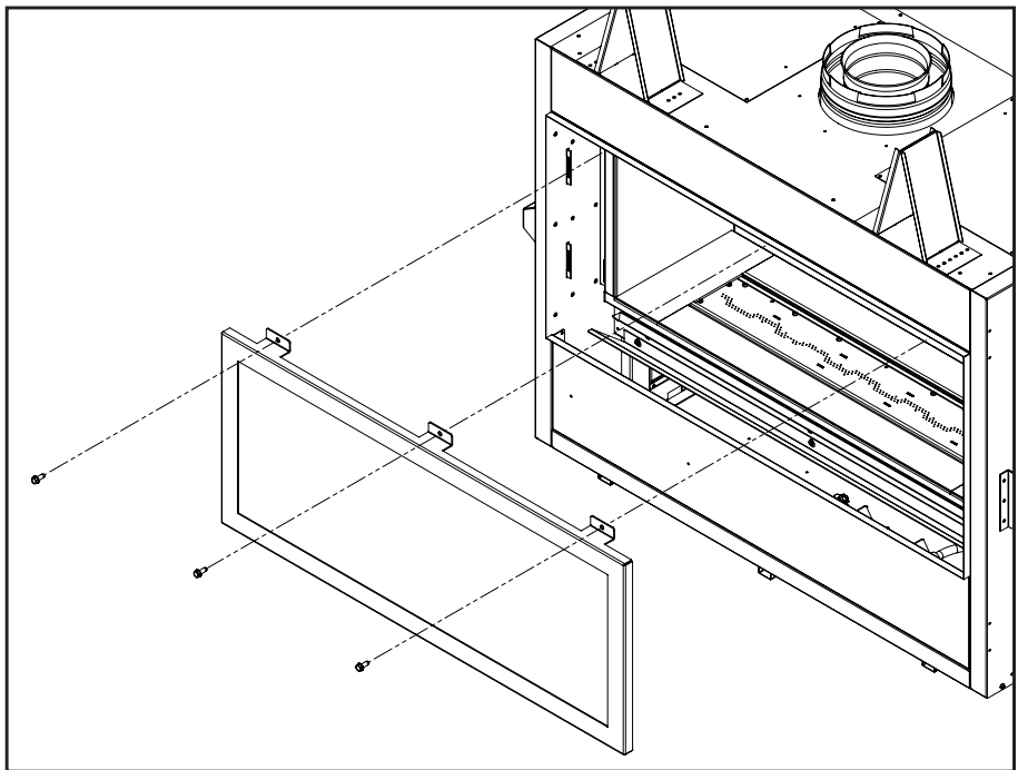
Figure 5. Door Removal Motion
