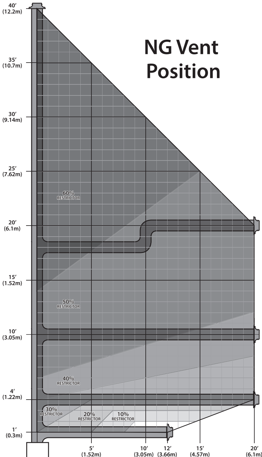
Figure 44. Natural Gas Vent Graph
