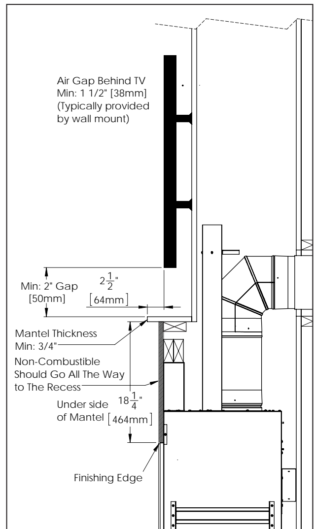
Figure 41. Recess Minimum TV Install Clearances
