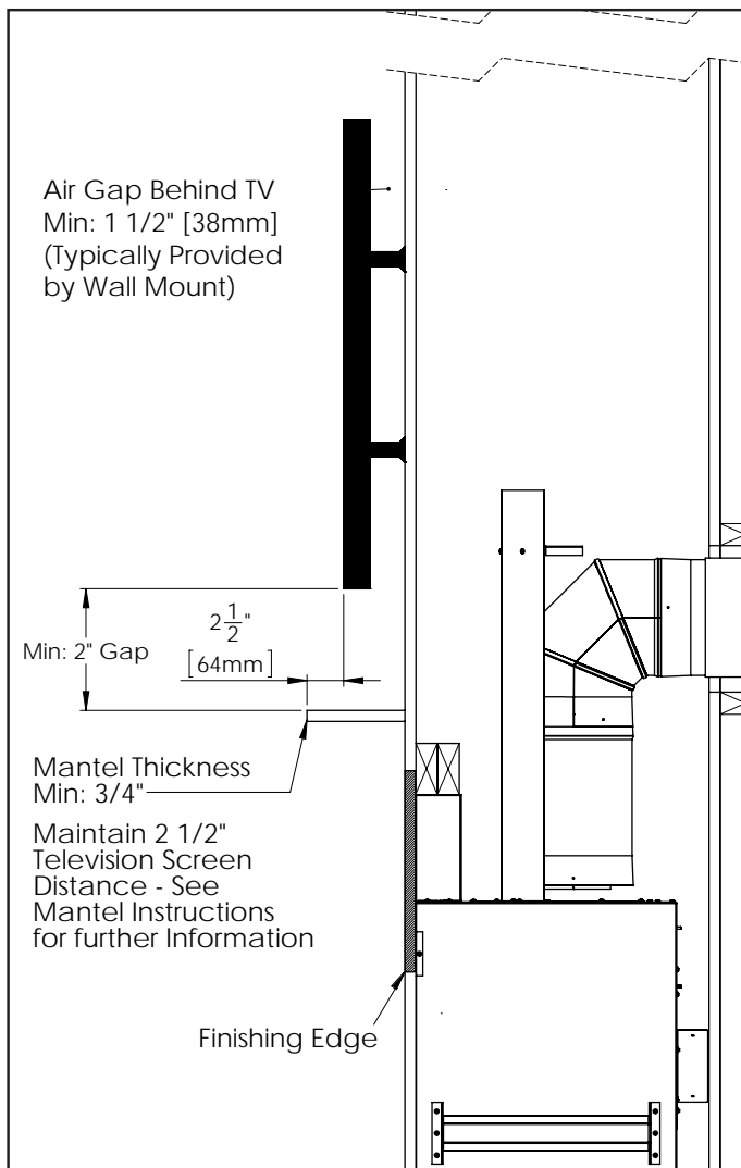
Figure 40. Minimum TV Install Clearances
