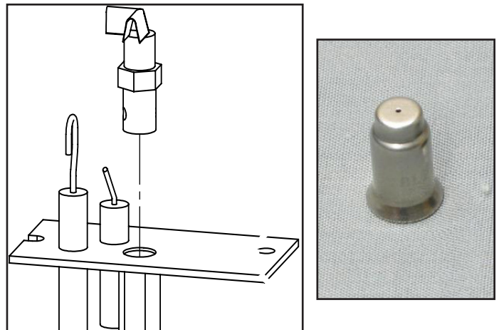
Figure 9. Pilot Orifice
