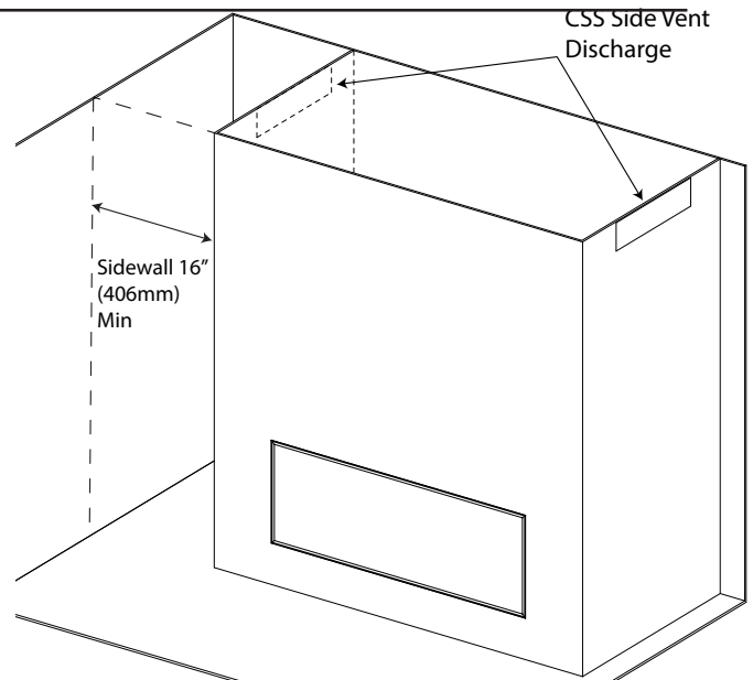
Figure 25 CSS Side Vent
