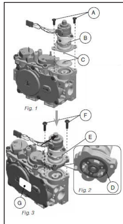
Figure 11: 885 Gas Valve
