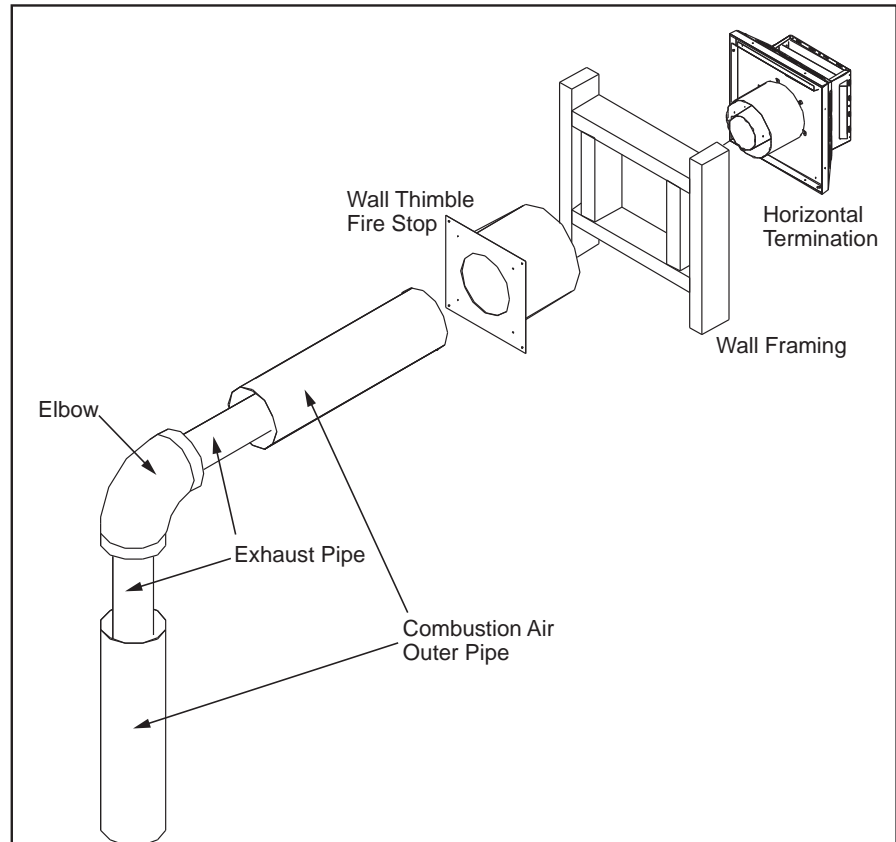
Figure 48. Horizontal Vent Termination
