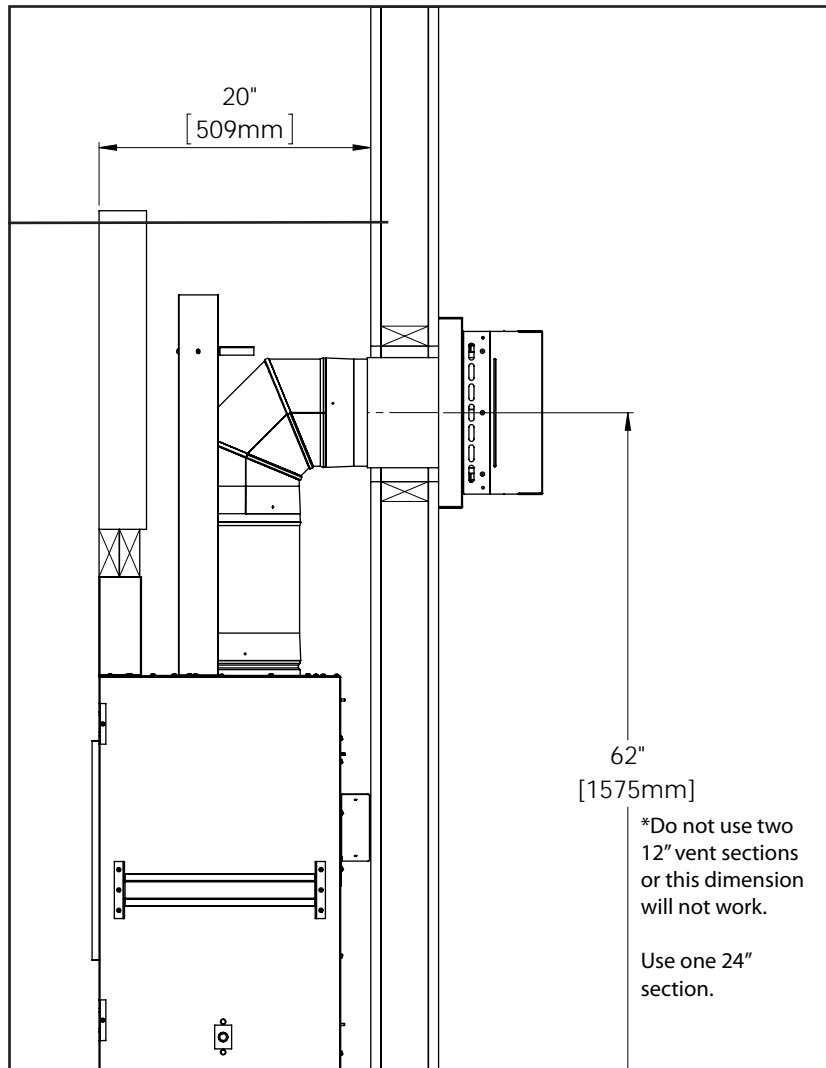
Figure 34 Minimum Horizontal Venting
