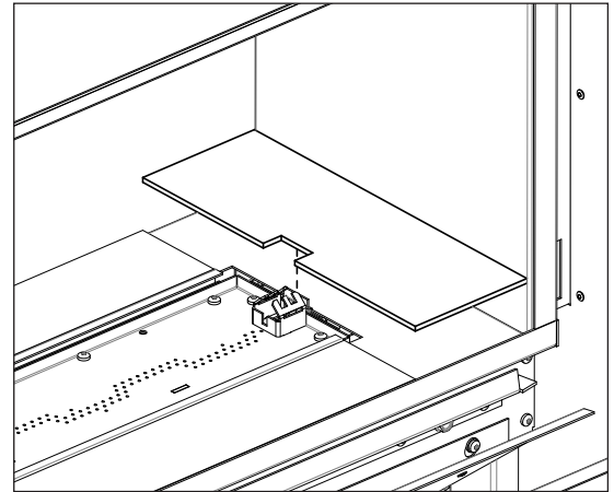
Figure 62 Bezel Placement Around Pilot
