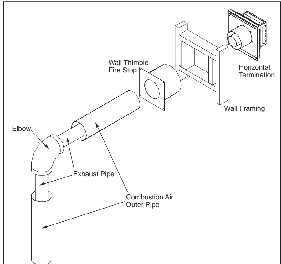
Figure 50 Horizontal Vent Termination
