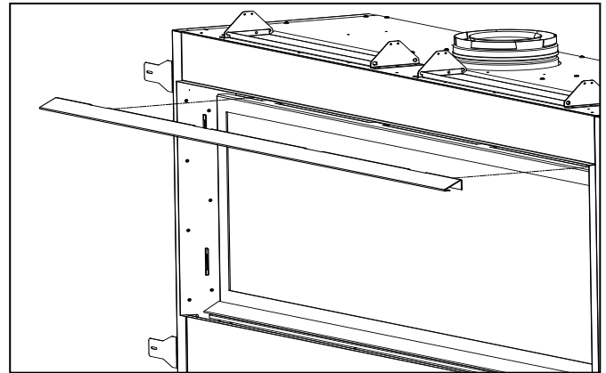
Figure 20 Discharge Accelerator removal
