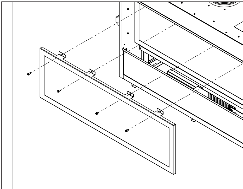
Figure 5: Door Removal Motion
