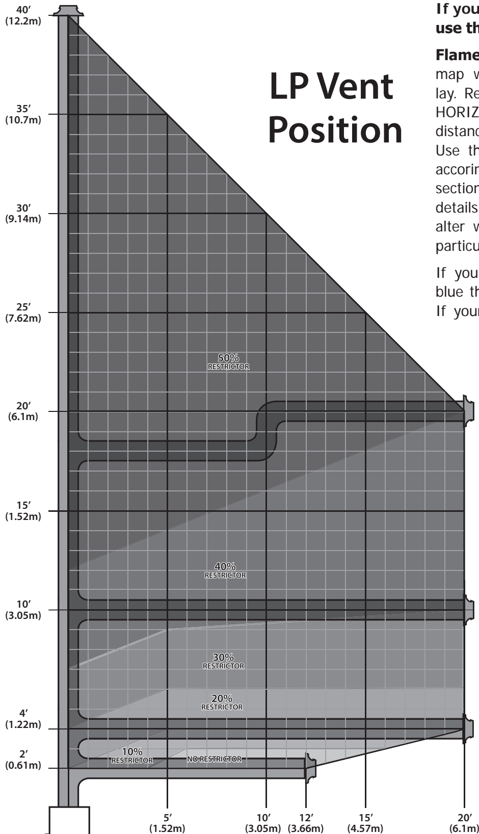
Figure 47 LP Vent Graph
