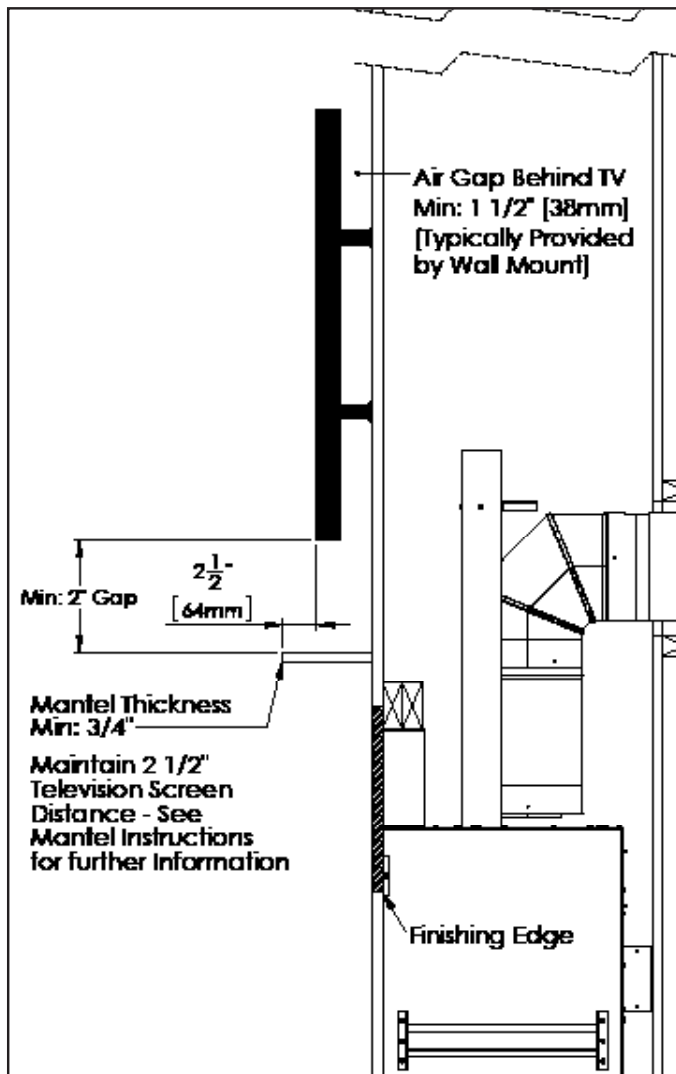
Figure 42 Minimum TV Install Clearances
