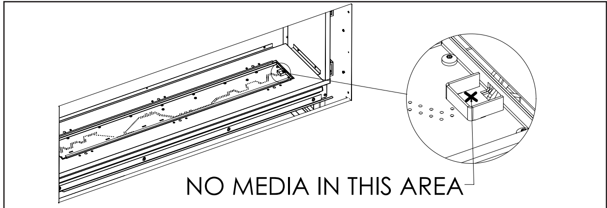
Figure 63 Protected Pilot Area
