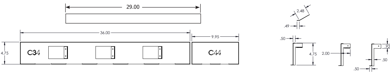
C44 CSS Combustible Facing Kit Dimensions
