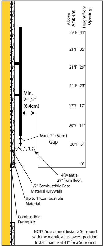
CSS - TV Clearances with Mantle
