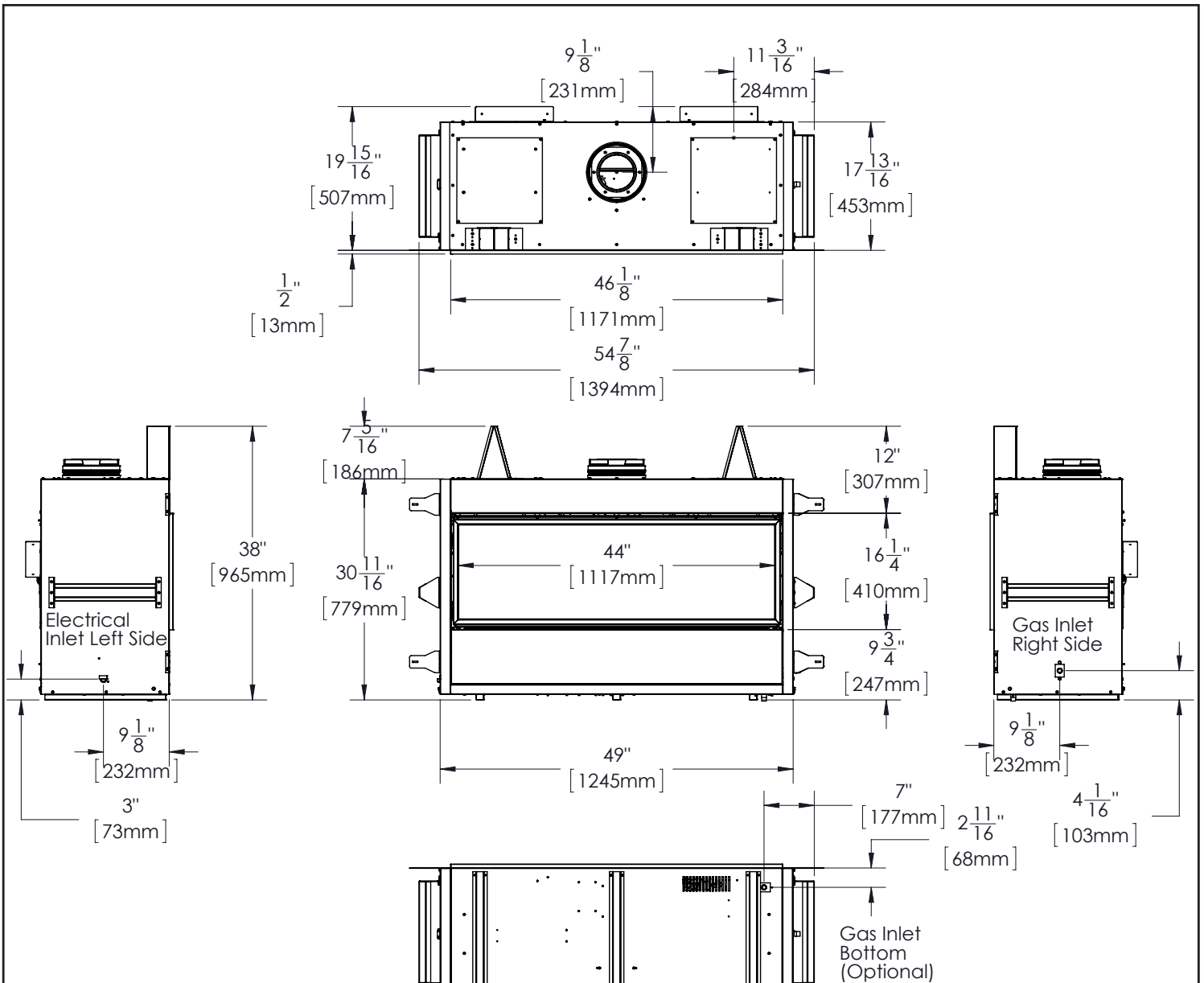
Figure 1: Unit Dimensions
