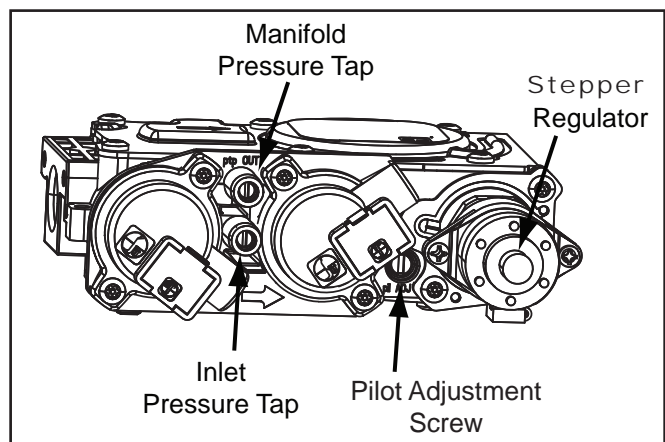
Figure 57: Fully Labeled Gas Valve. See Dexen User Manual for C34ID valve details
