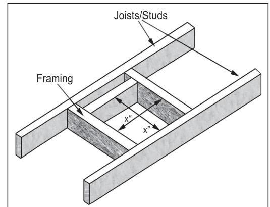
Figure 55: Vent Framing - Wall or Ceiling
