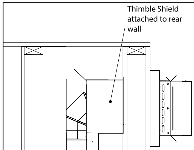
Figure 38: CSS Heat Shield
