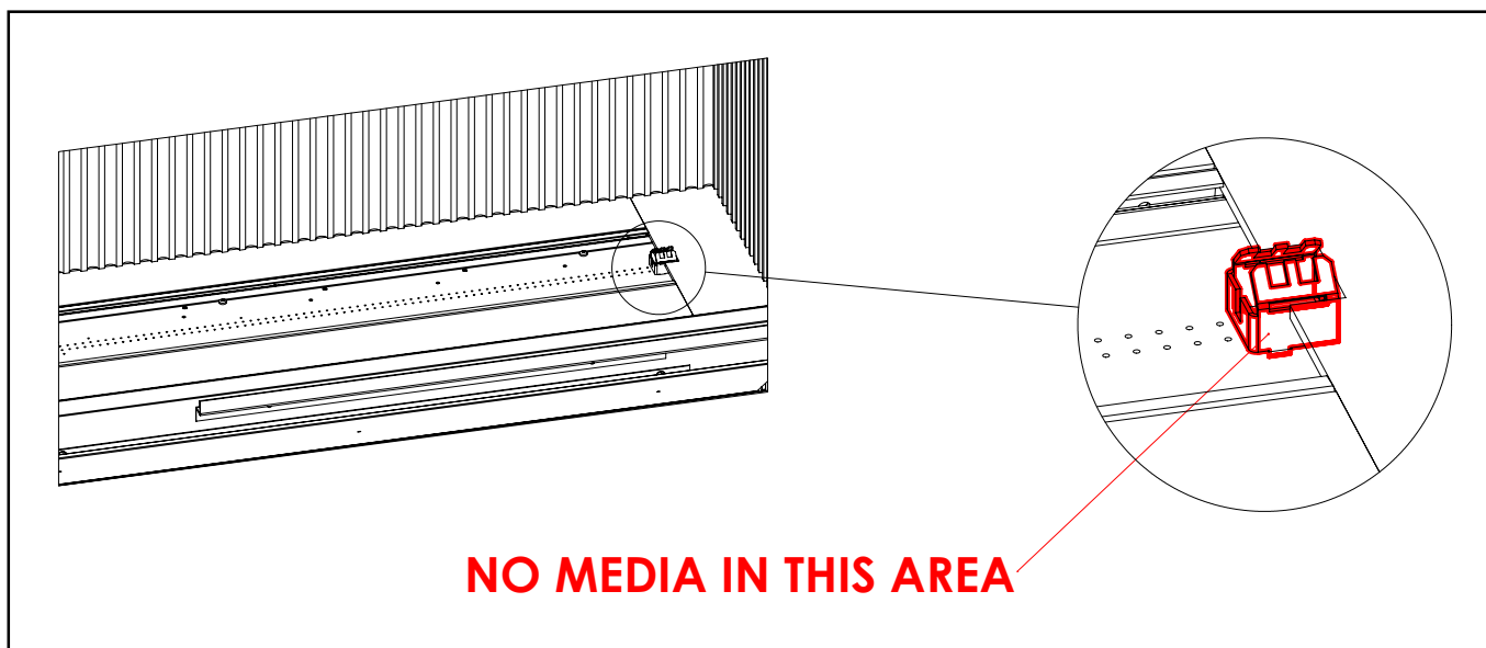
Figure 74: Protected Pilot Area
