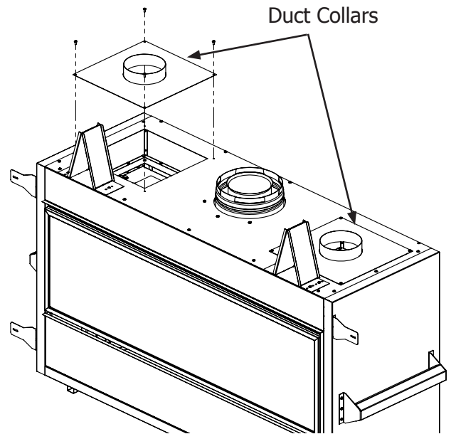
Figure 28: CSS Duct Collar Plates
