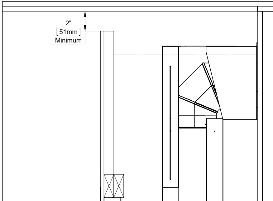
Figure 36: Open Chase
