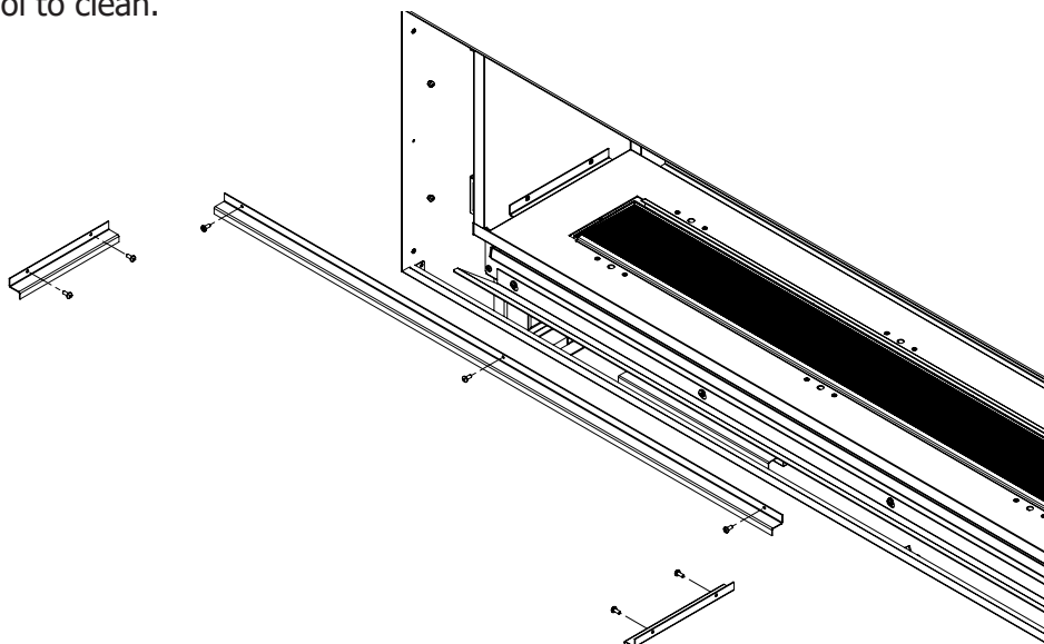
Figure 76: Panel Retainer Installation
