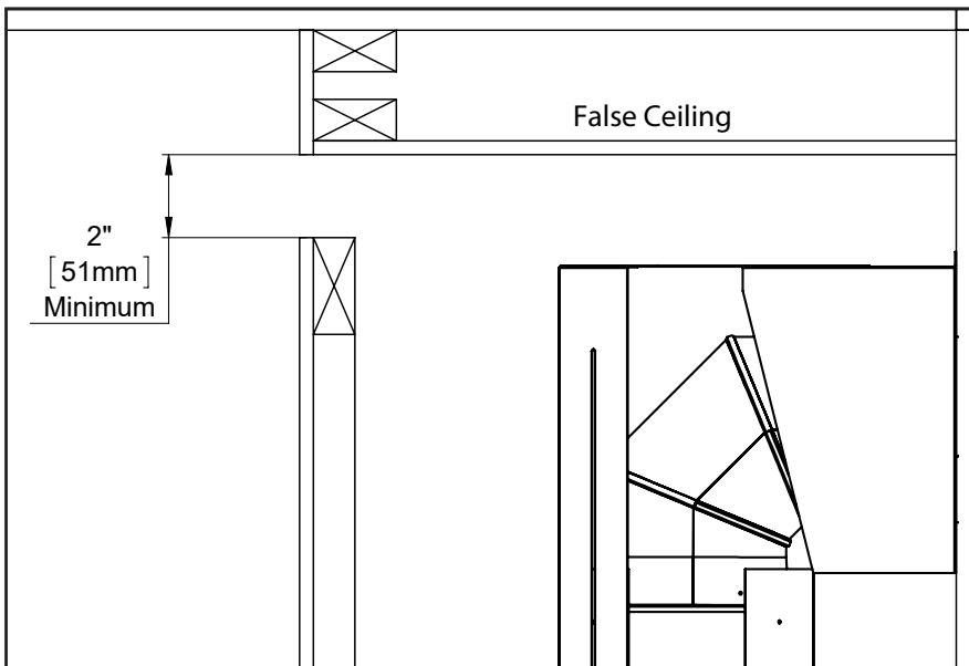
Figure 34: False Ceiling
