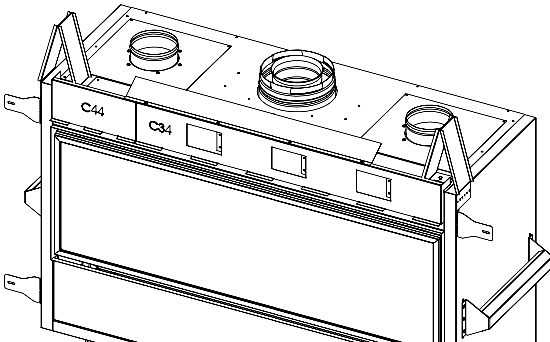
Figure 29: CSS Combustible Facing Kit
