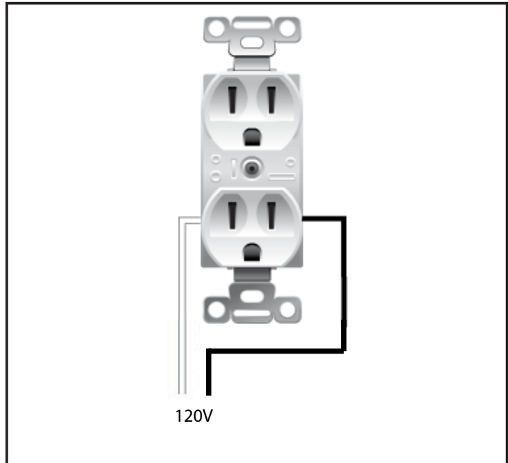
Figure 68: C44I Receptacle Wiring
