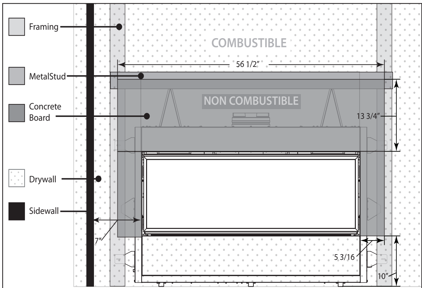
Figure 30: Non-Combustible Zones
