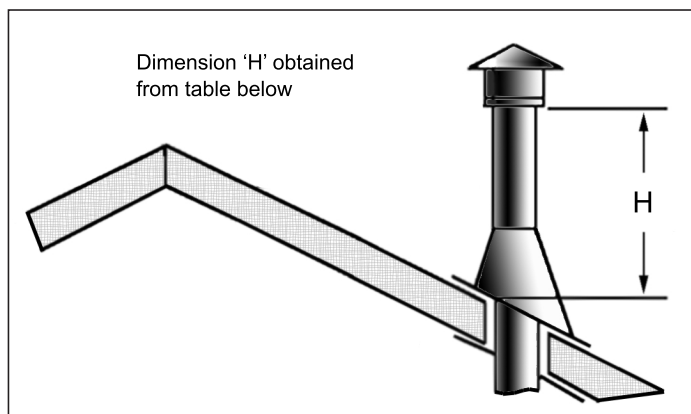
Figure 63: Height of Vertical Vent Termination; Reference Table 7
