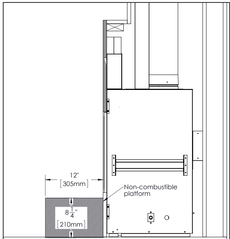
Figure 43: Non-Combustible Platform
