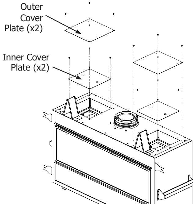
Figure 27: CSS Duct Cover Plates
