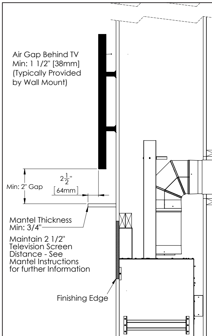
Figure 52: Minimum TV Clearance - Mantel
