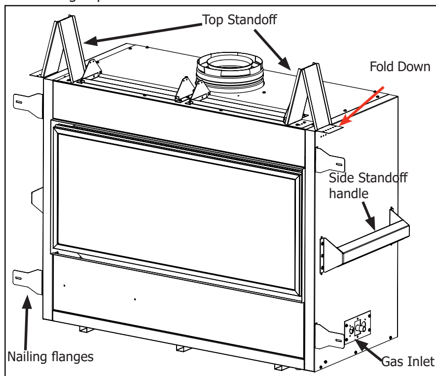
Figure 13: Fireplace Install Preparation - 1
