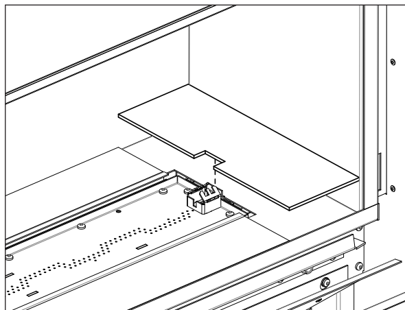
Figure 73: Burner Bezel Placement Around Pilot
