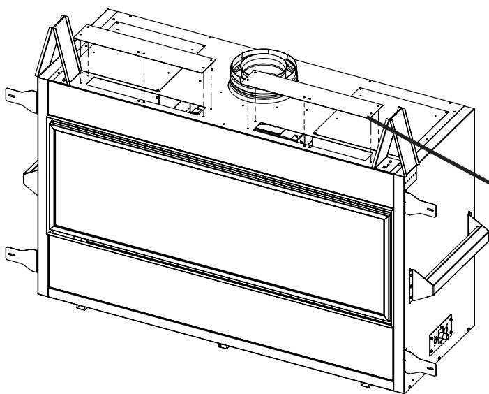
Figure 26: CSS Top Cover Plates
