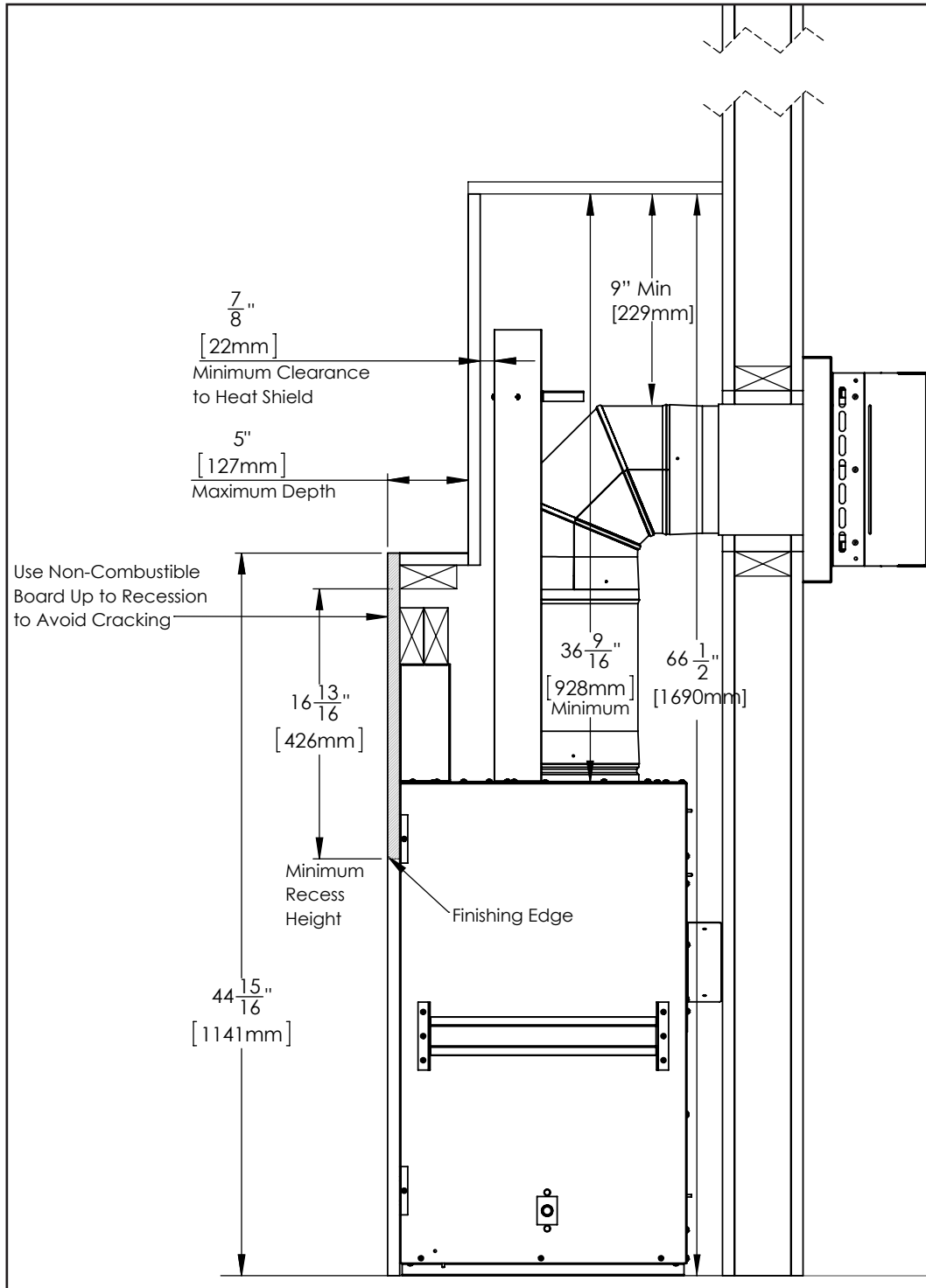
Figure 47: Install Dimensions with Recess
