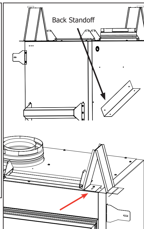
Figure 14: Fireplace Install Preparation - 2
