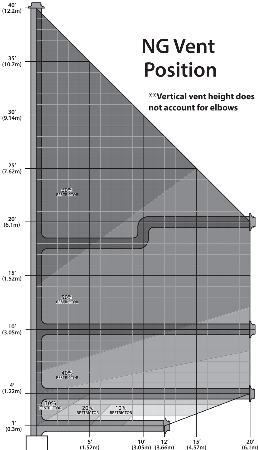
Figure 57: Natural Gas Vent Graph
