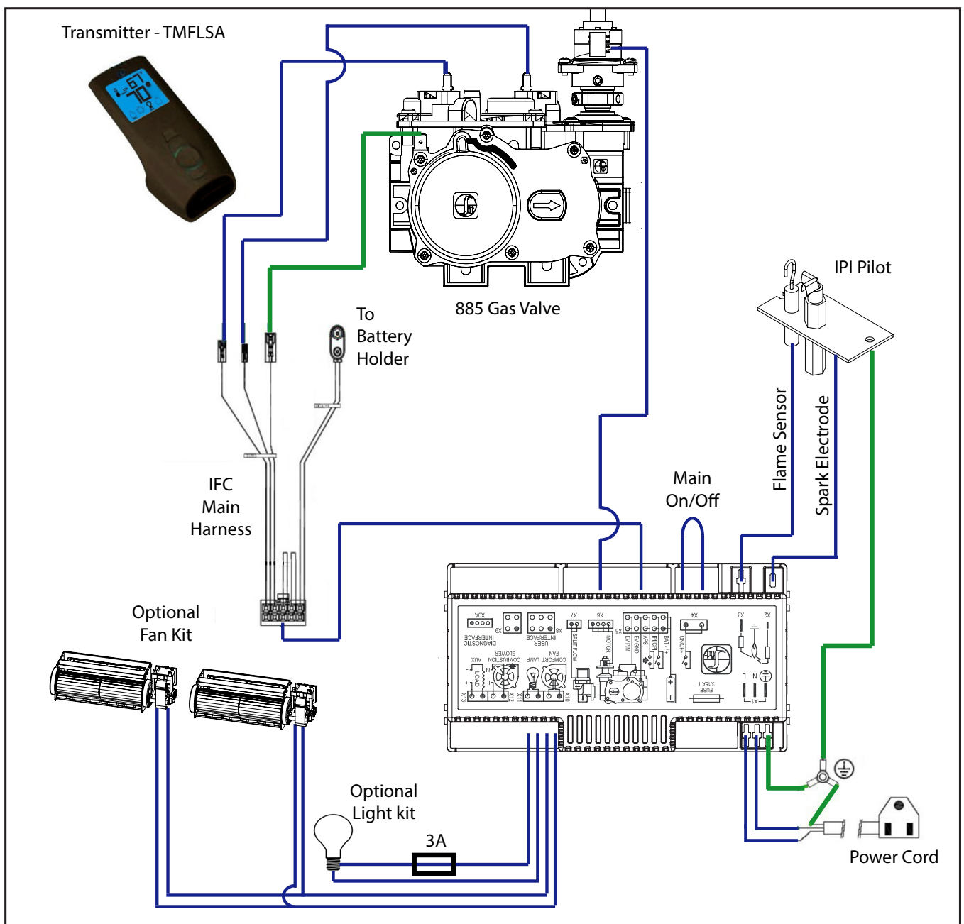
Figure 67: C44I Wiring Diagram
