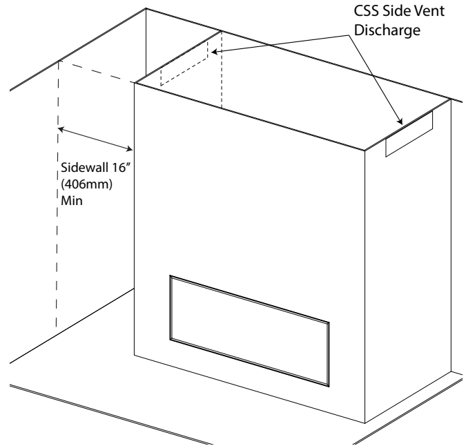
Figure 33: CSS Side Vent
