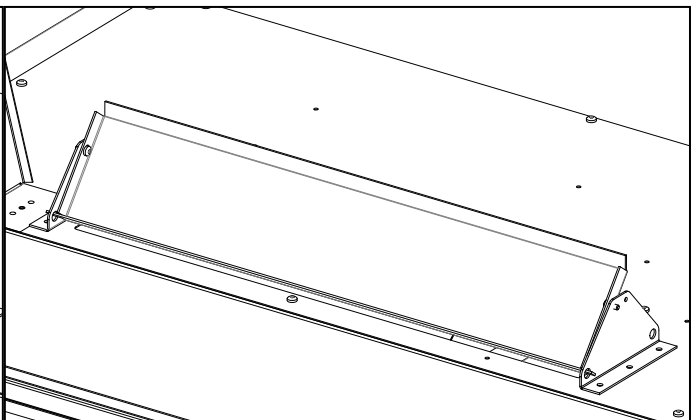
Figure 24: CSS Flaps - Open
