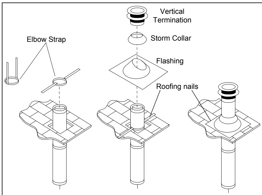
Figure 62: Vertical Vent Termination
