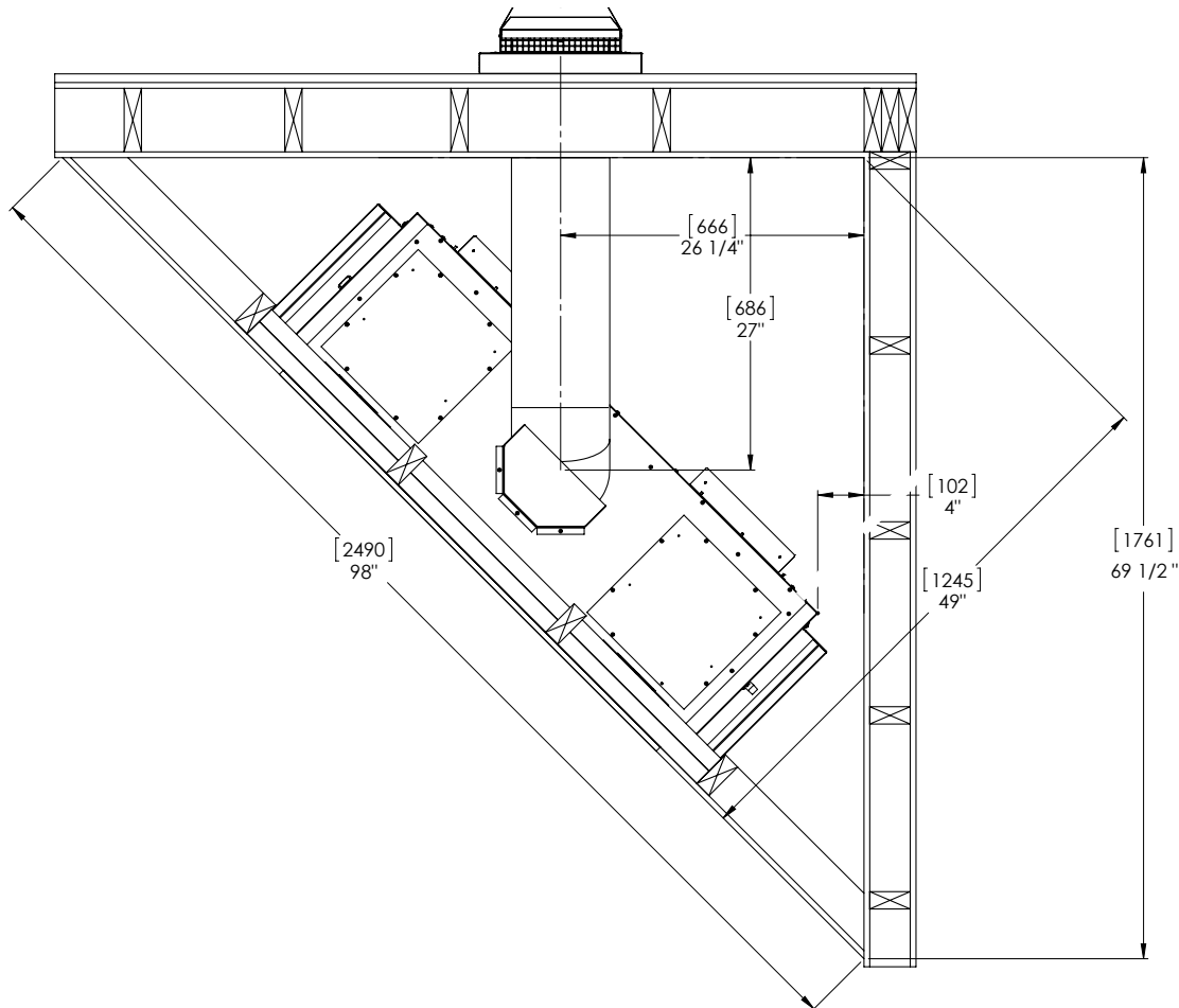
Figure 48: Corner Installation Dimensions
