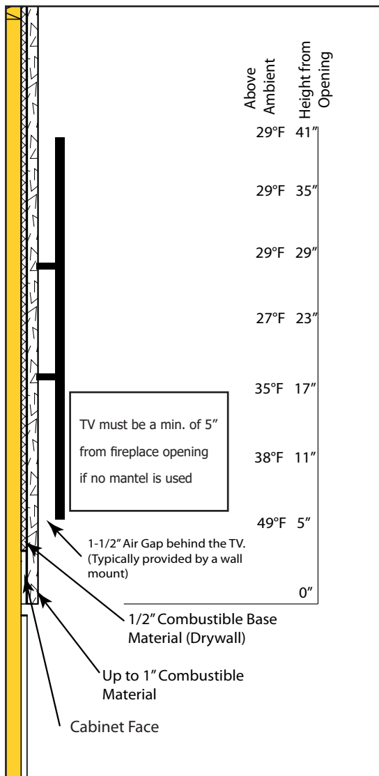
Figure 39: CSS TV Clearances - Flat Wall
