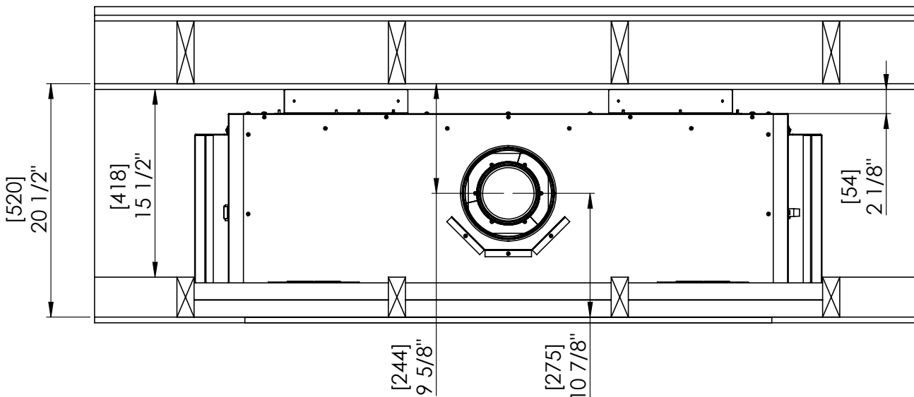
Figure 51: Vertical Vent Installation Dimensions
