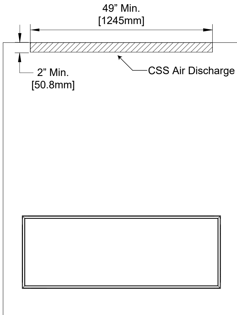
Figure 32: CSS Front Outlet
