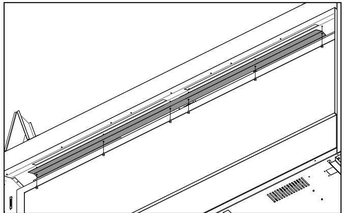
Figure 22: CSS Cover Removal
