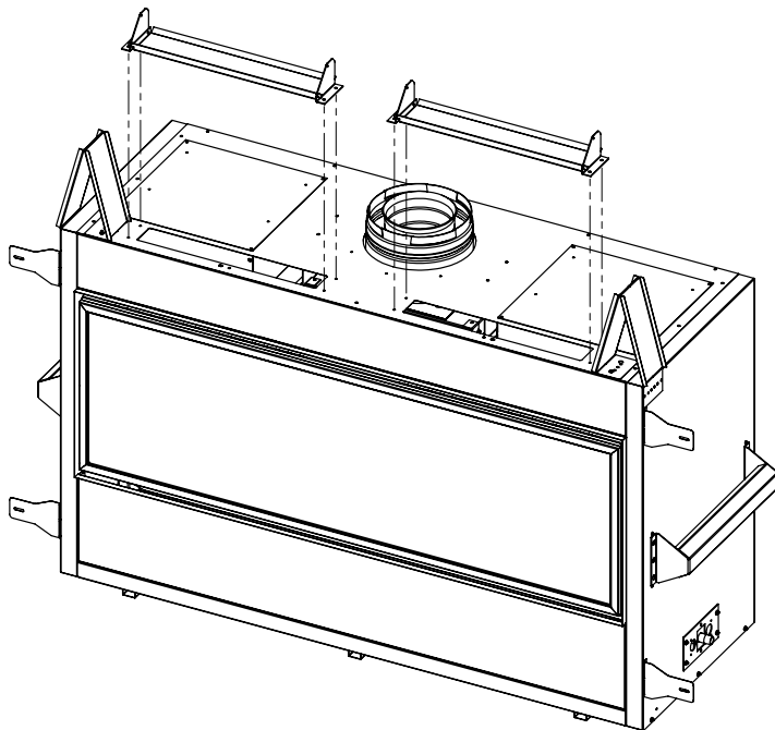
Figure 25: CSS Flaps - Removal
