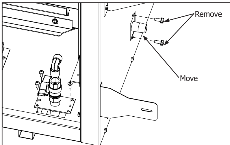
Figure 41: Alternate Gas Inlet Location
