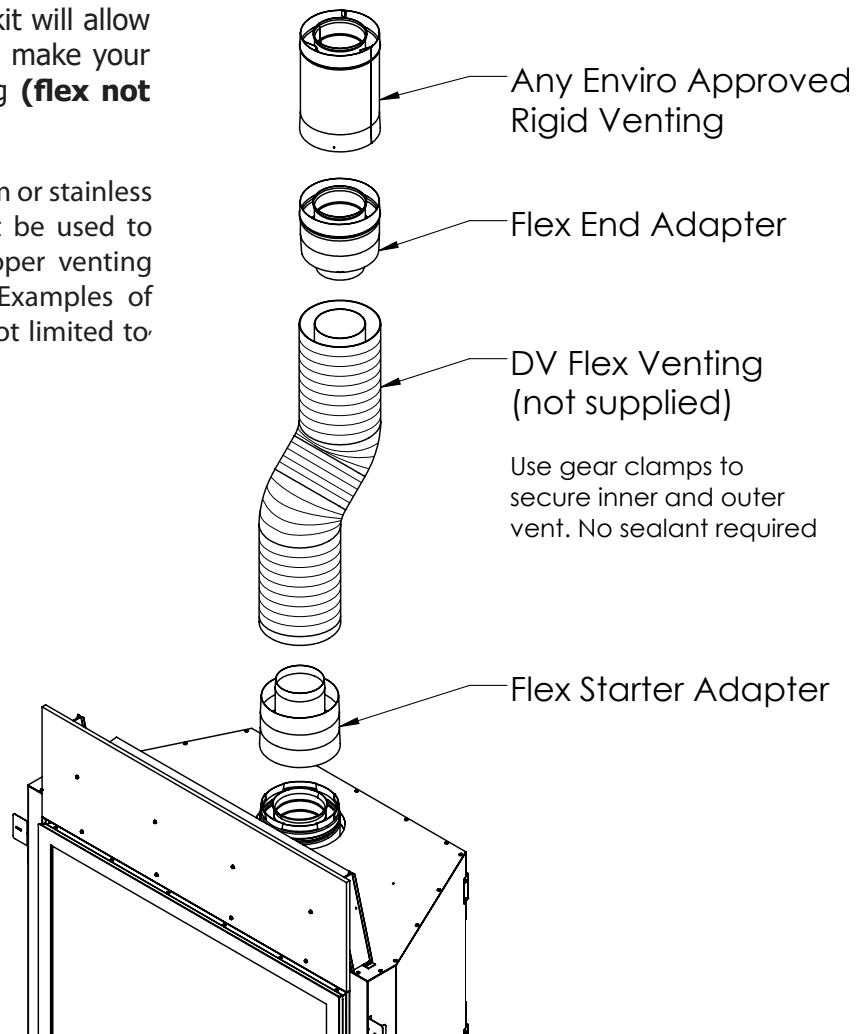
Figure 56: Flex Vent Adaptor Kit
