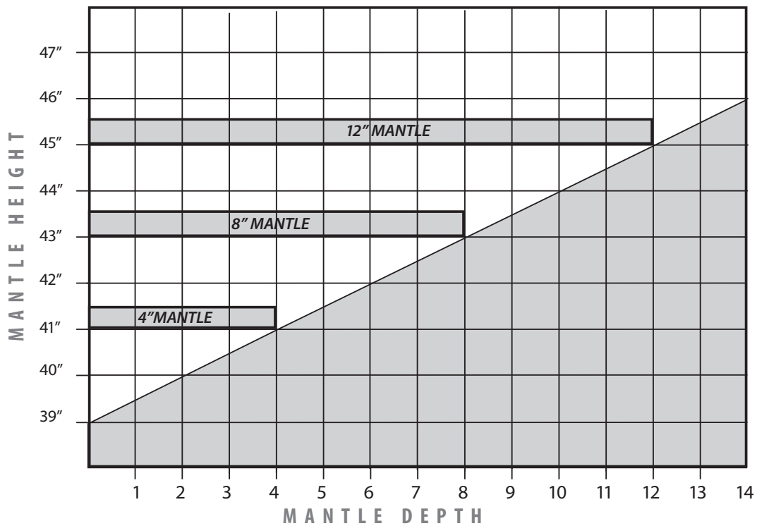
Figure 44: Minimum Mantel Height - Non CSS
