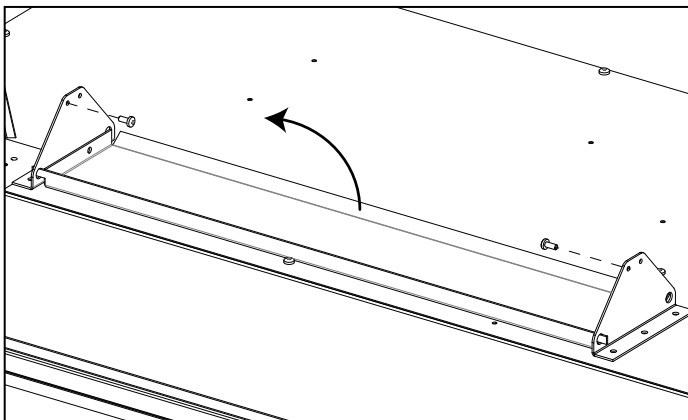
Figure 23: CSS Flaps - Closed
