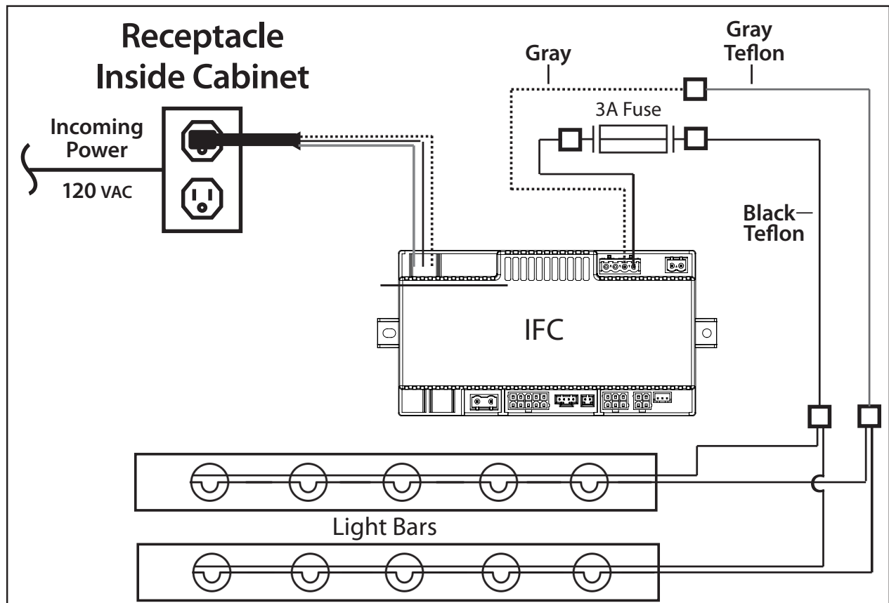
Figure 70: Light Kit Wiring Diagram
