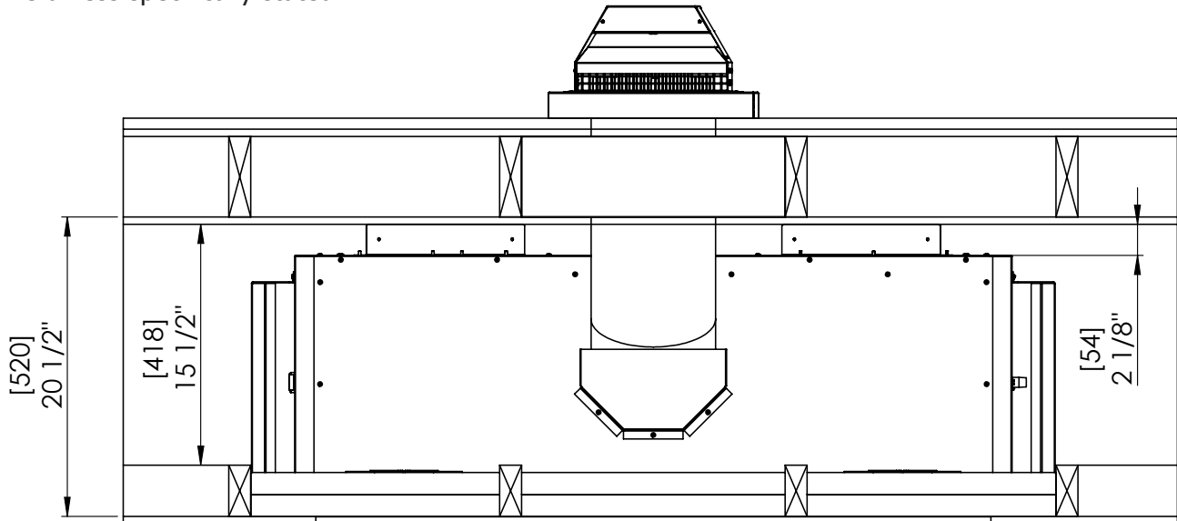
Figure 50: Horizontal Vent Installation Dimensions
