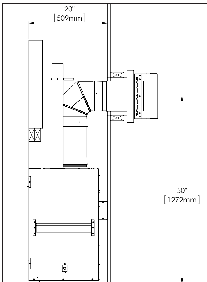
Figure 42: Minimum Horizontal Venting
