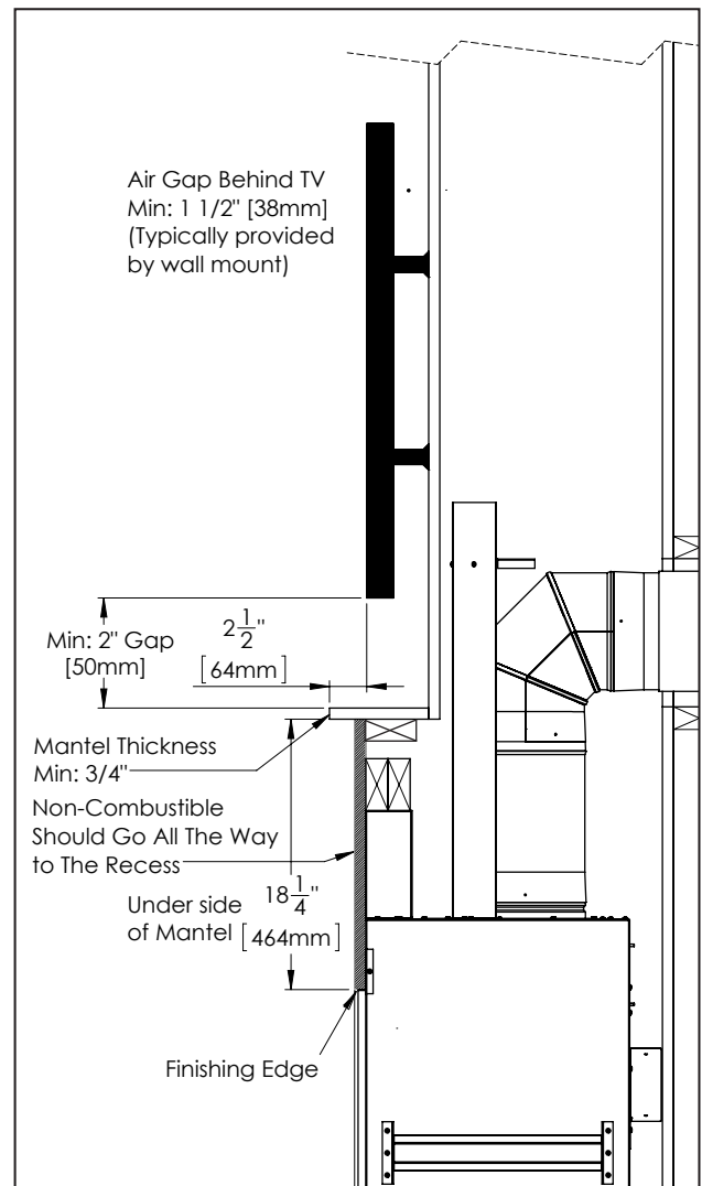
Figure 53: Minimum TV Clearance - Recess
