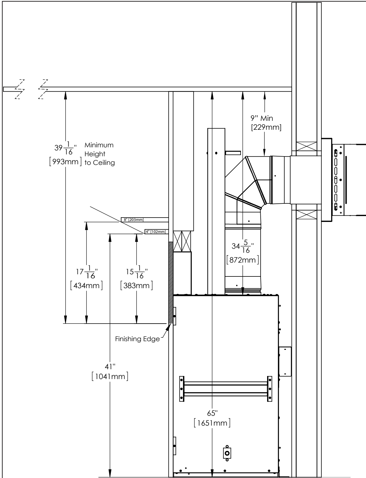
Figure 46: Install Dimensions - Minimum Mantel
