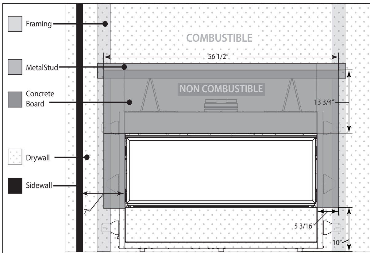
Figure 20: Finishing Non-Combustible Zones
