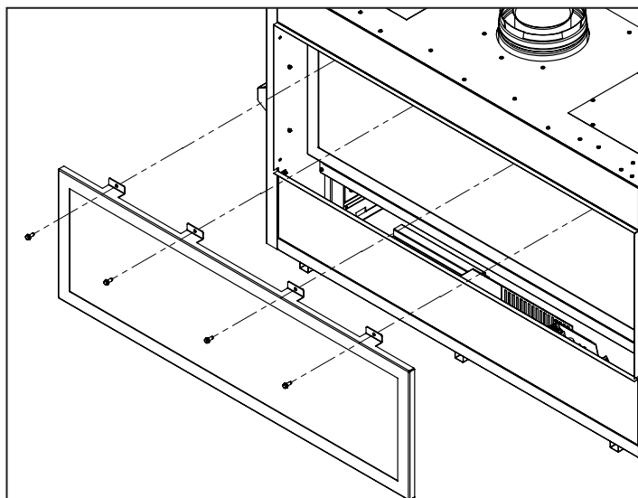
Figure 5: Door Removal Motion
