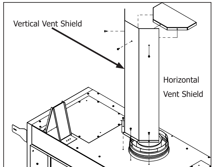
Figure 49: Vent Shielding Install
