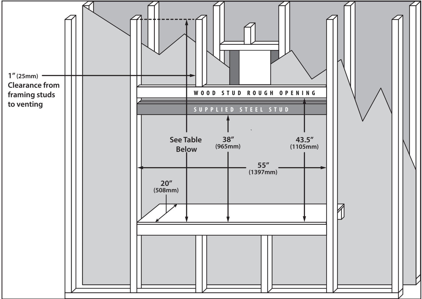
Figure 19: Construction Framing Dimensions
