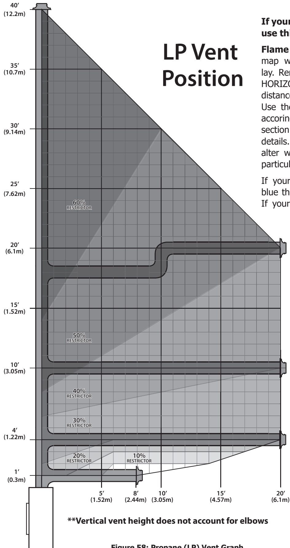
Figure 58: Propane (LP) Vent Graph
