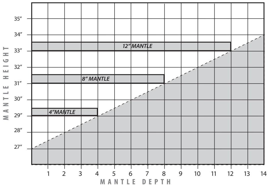
Figure 45: Minimum Mantel Height - CSS
