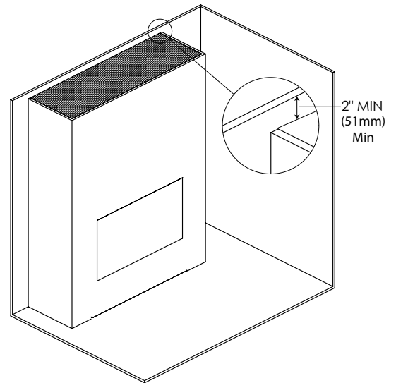
Figure 37: Open Chase - Iso View
