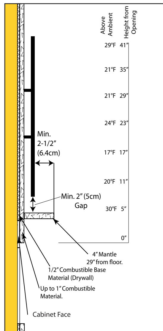
Figure 40: CSS TV Clearances - Mantel
