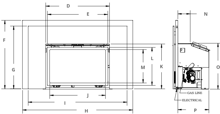
Figure 1.5 Unit dimensions (Tolerance \pm 1/8" ) [1.25 mm]
