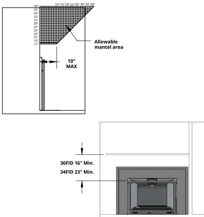
Figure 2.2 Install clearances
