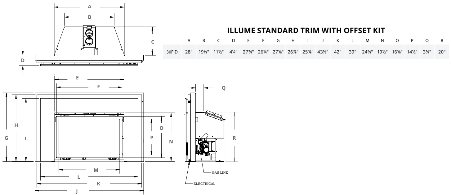
Figure 1.4 Unit dimensions (Tolerance ± 1/8") [1.25 mm]
