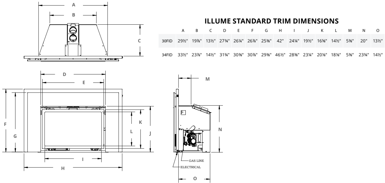
Figure 1.3 Unit dimensions (Tolerance ± 1/8") [1.25 mm]
