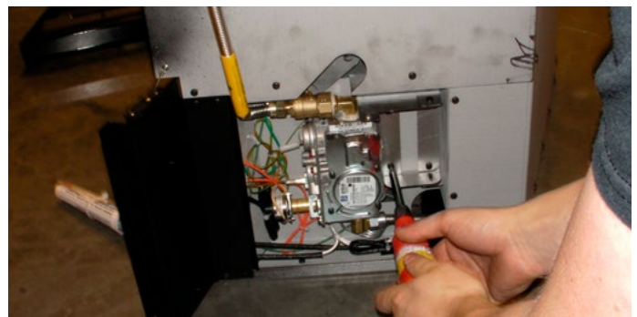
Figure 4.2 Propane conversion kit showing pilot orifice, main burner orifice,
