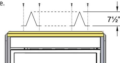
Figure 4.b Installing standoffs
