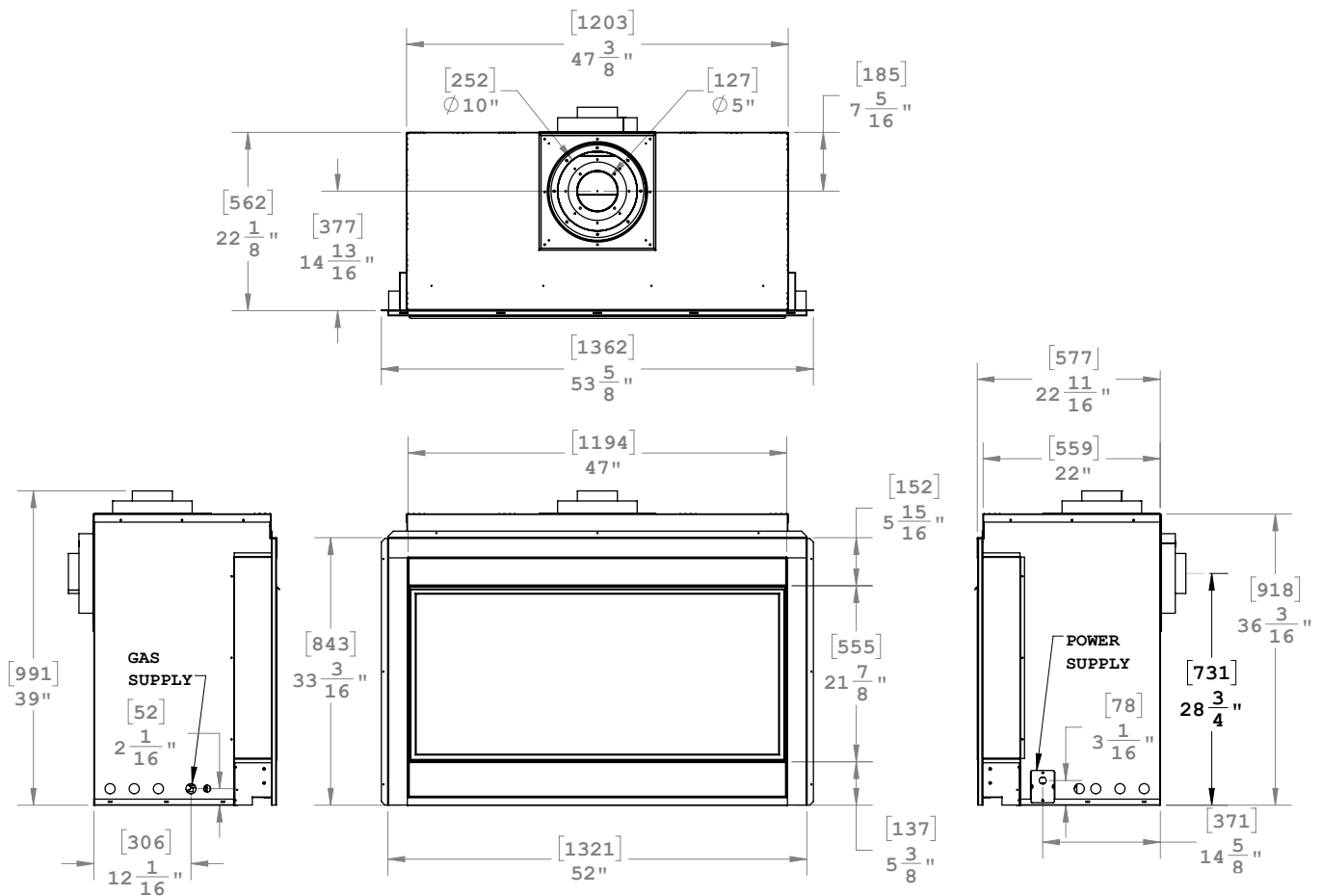
Figure 2. Fireplace dimensions (Tolerance \pm \frac{1}{16} ").
