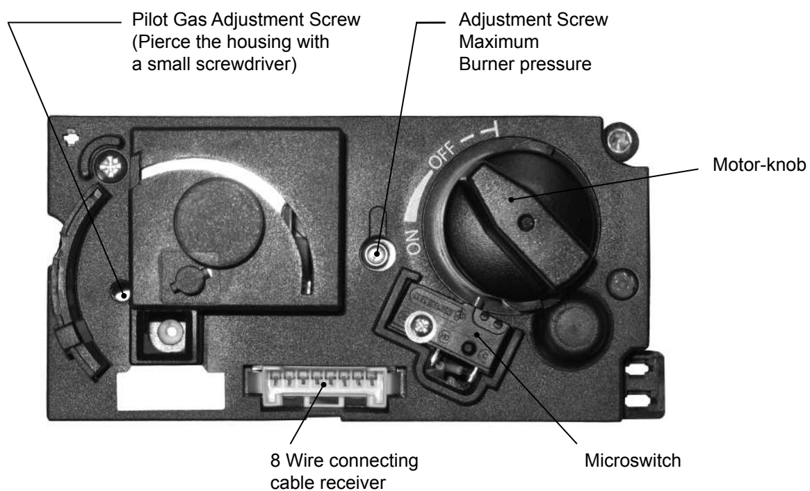
Figure 17: Gas regulator block - Front
