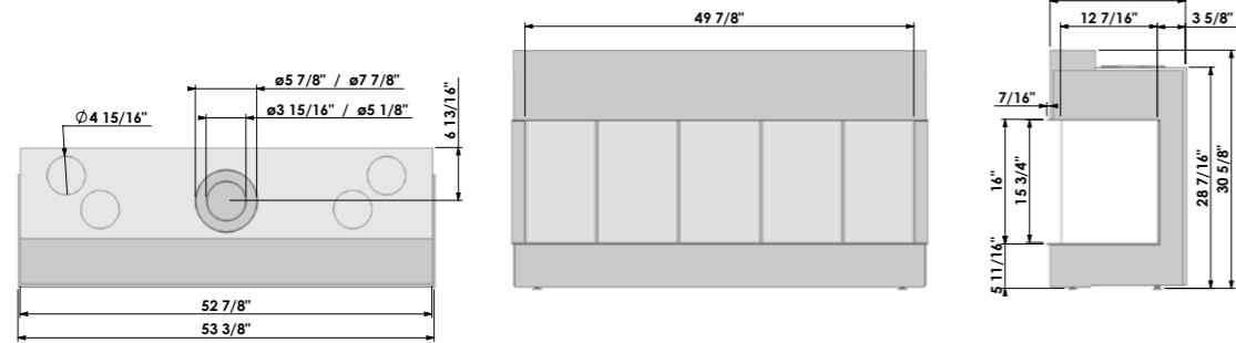
View Bell Large 3 - hidden door
