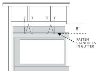
Figure 4.b Installing standoffs
