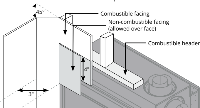
Figure 21.d Combustible facing materials.
