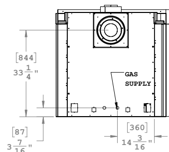
Figure 18.b Gas Inlet Supply location
