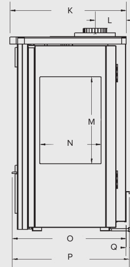
FDV451N Free Standing Direct Vent Stove – Natural Gas, F450FBL Door Front – Charcoal with Black Posts, F451SDFBL Side Doors – Flame Panel Charcoal – with Black Frame, MQG5C Bronze Glass (x3), RBCB1 Cannonballs, F45LG Log Grate, F45FK Fan Kit.
