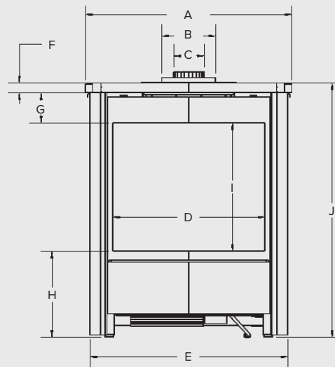
FDV451N Free Standing Stove – Natural Gas, F450FBL Door Front – Charcoal with Black Posts, F451SDSBL Side Doors – Solid Charcoal Panel with Black Frame, MQG5C Bronze Glass (x3), MQROCK3 Rock Set – Multi-Colored, F451RLT Traditional Brick Liner, F45FK Fan Kit.
