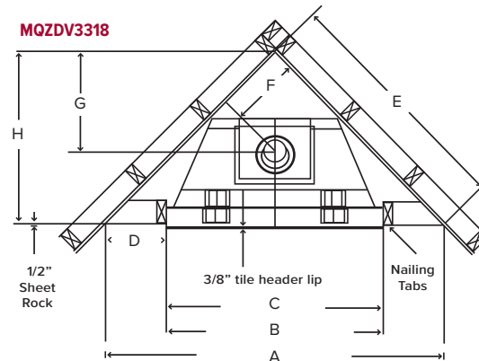
1: MQZDV3318N Zero Clearance Direct Vent Natural Gas Fireplace, MQLOGC22 Oak Log Set, V130GBL Black Grill Kit.
