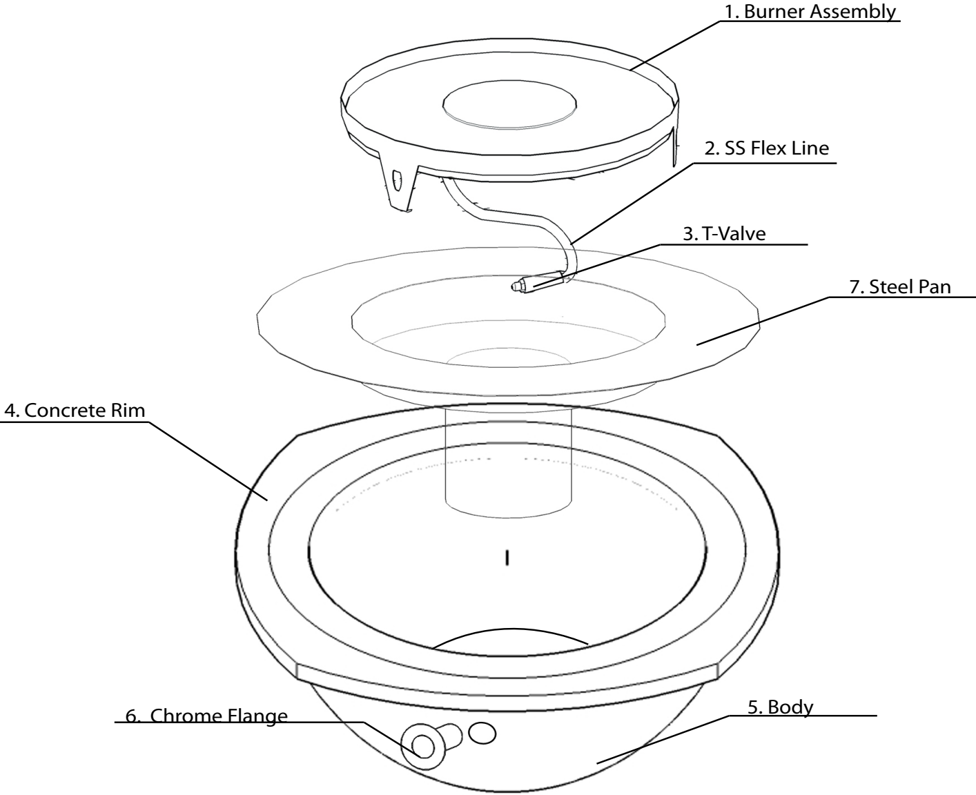
FIG. 2. Firebowl - Exploded
