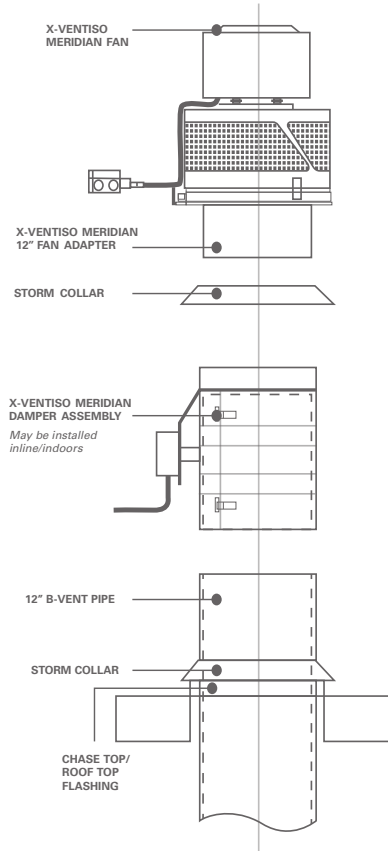
X-Ventiso Meridian system for Maximus Linear shown.
