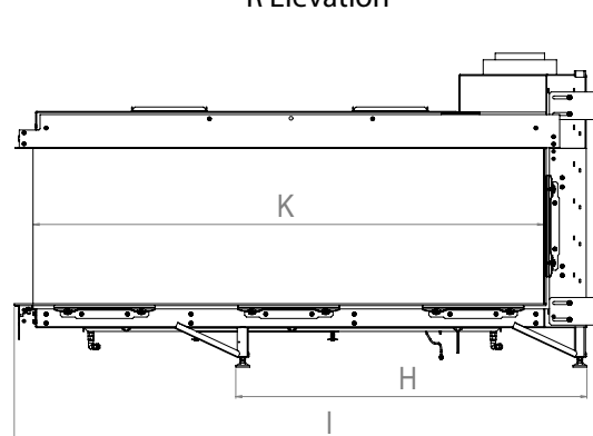
R Elevation
