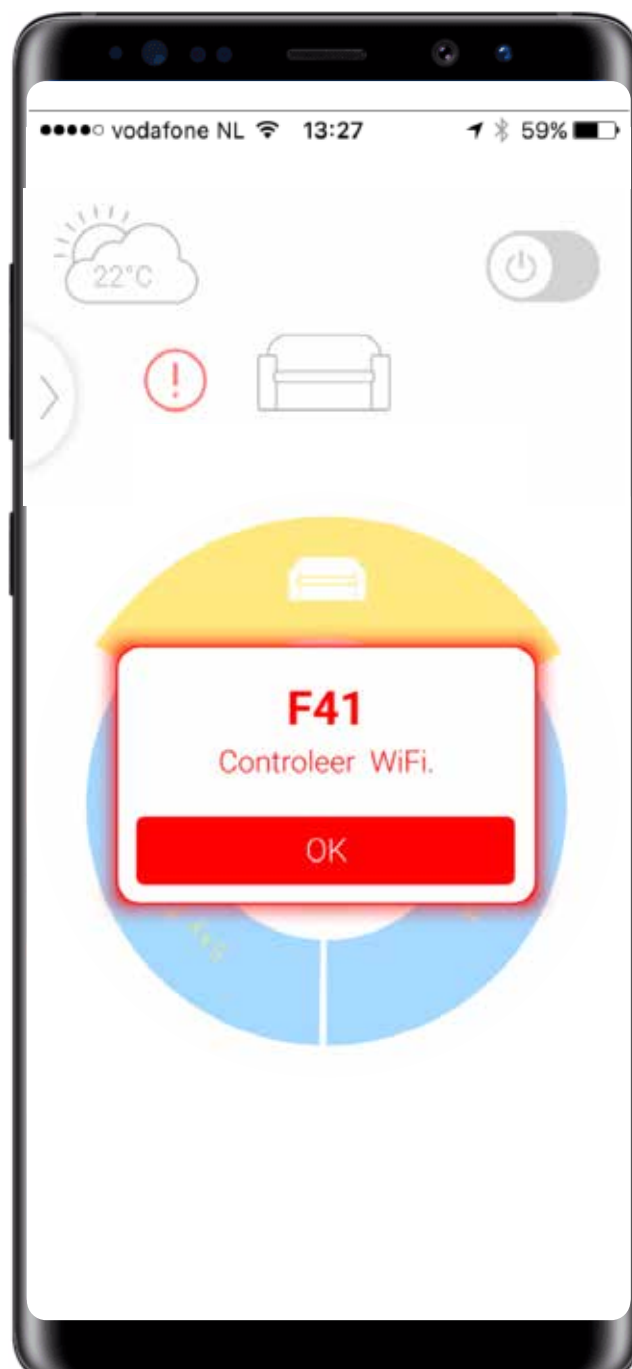
Figure 131: Application screen
