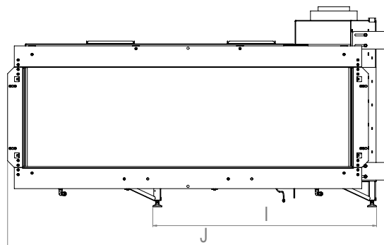
R Elevation
