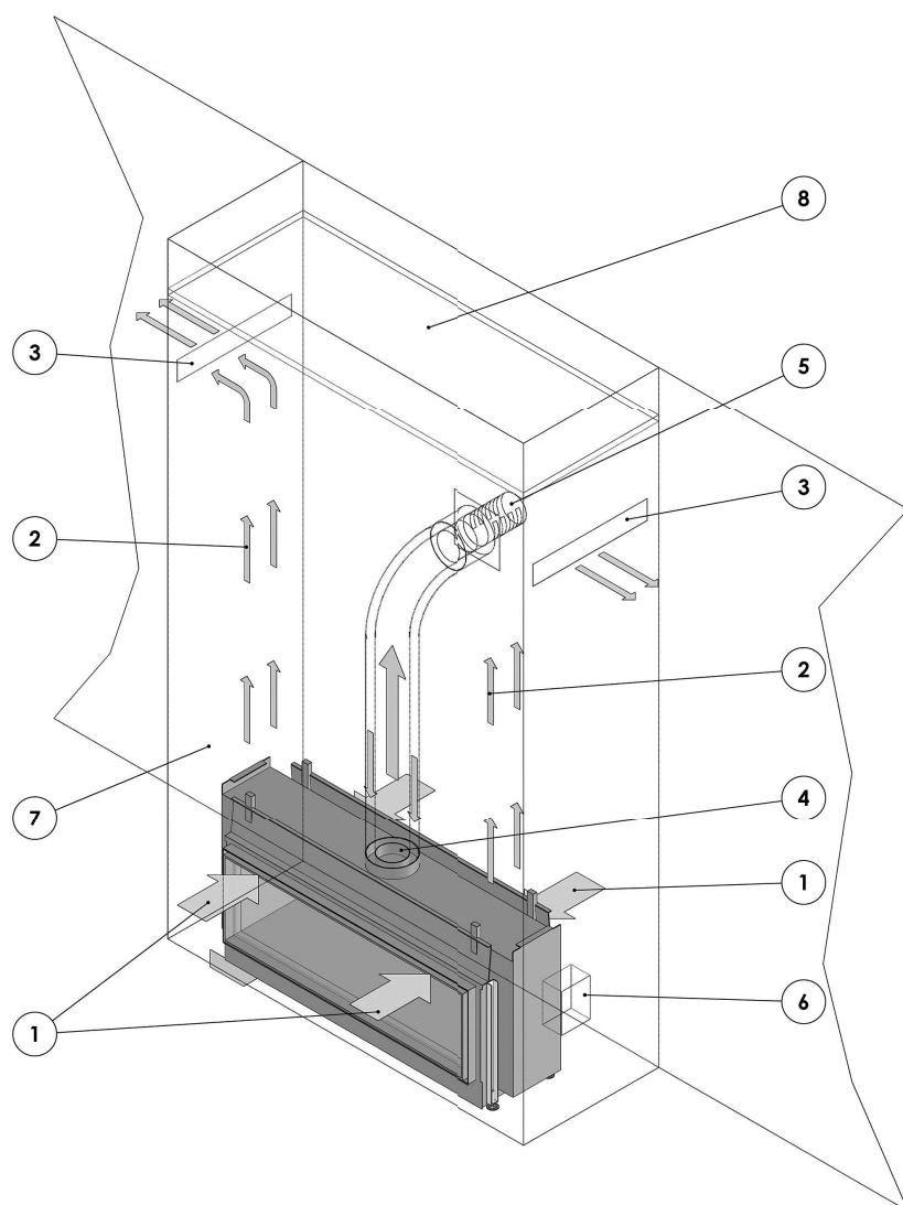
Figure 13: Appliance installed in ventilated chimney breast / Enclosure Horizontal outlet of the flue gas exhaust /combustion air supply via the wall.
