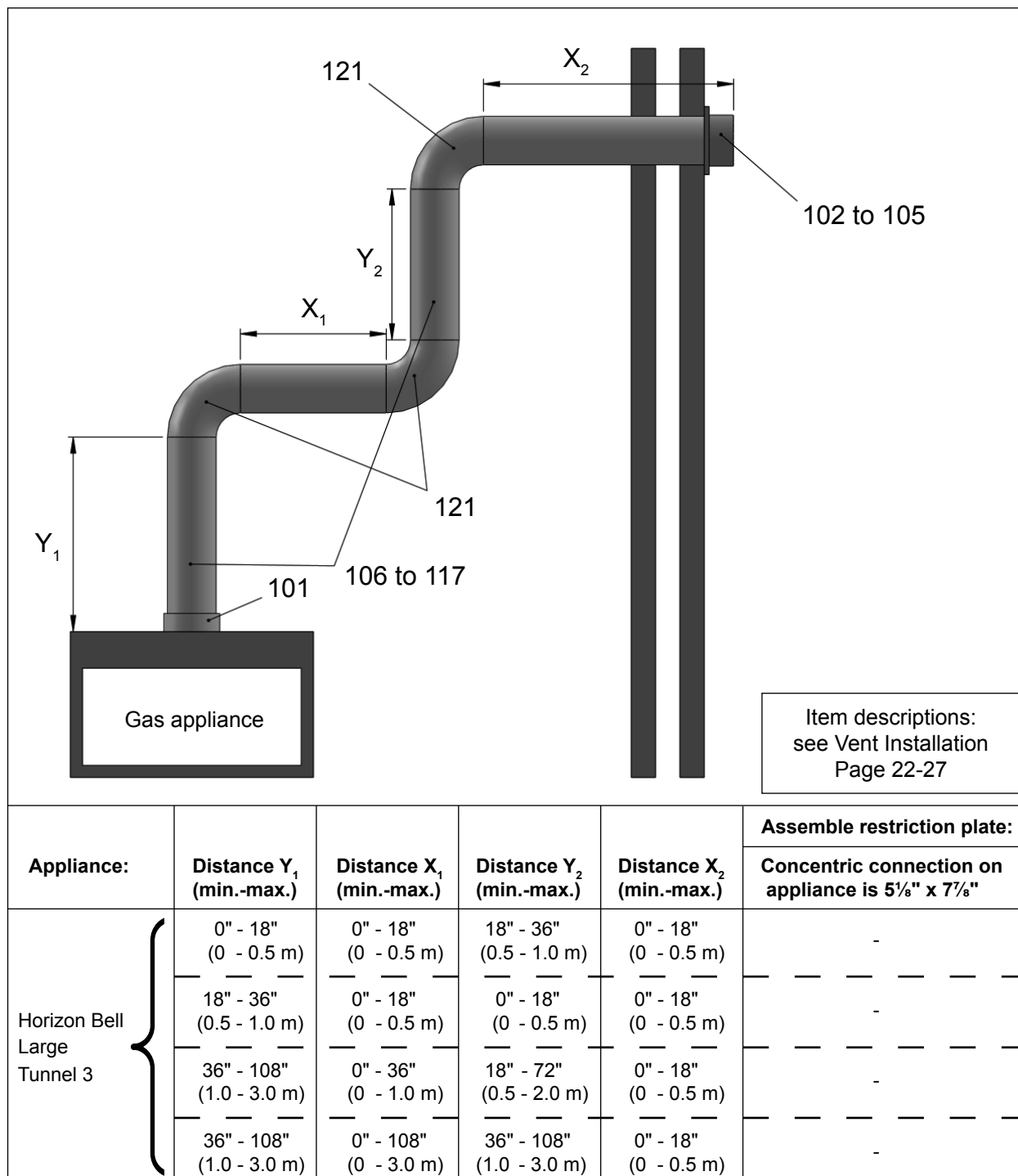
Figure 11: Horizontal wall termination
