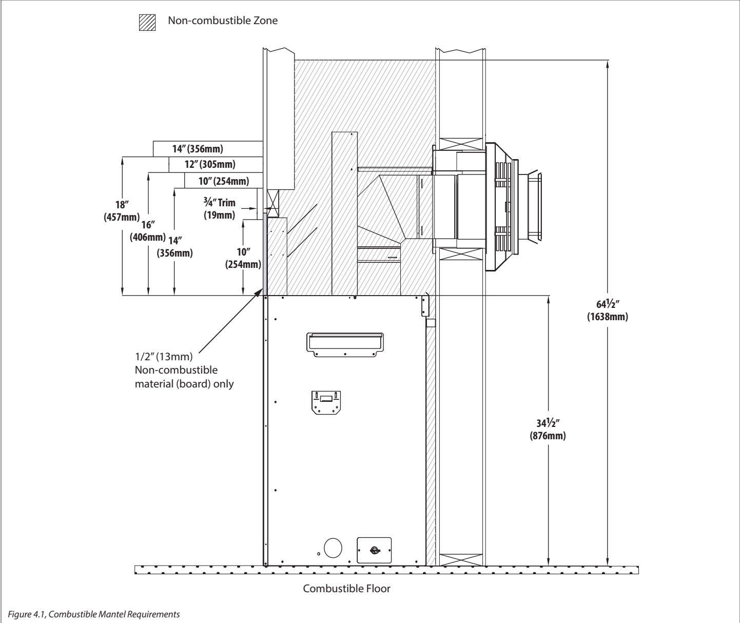
Figure 4.1, Combustible Mantel Requirements
