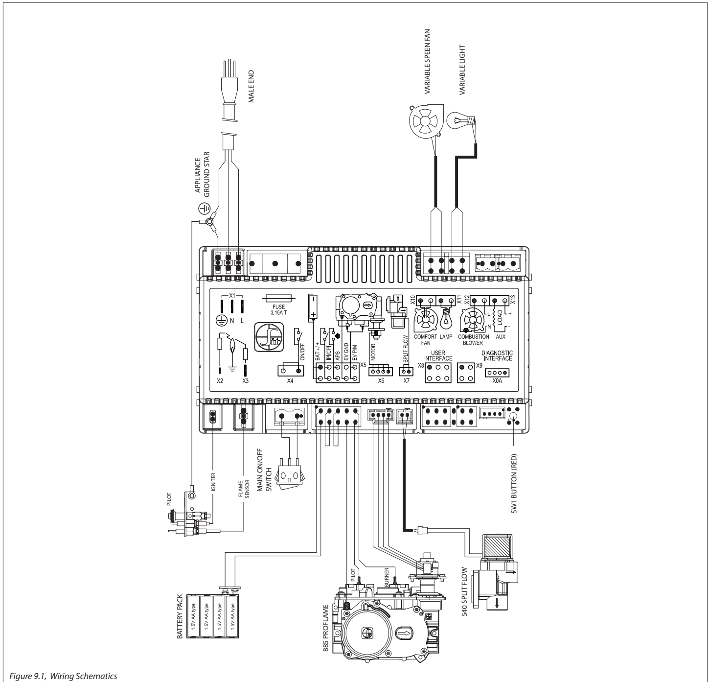
Figure 9.1, Wiring Schematics
