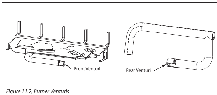
Figure 11.2, Burner Venturis
