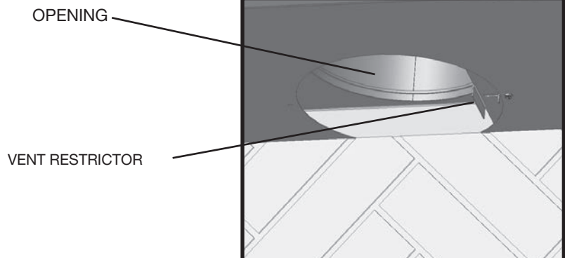
Figure 44: Vent restrictor.
