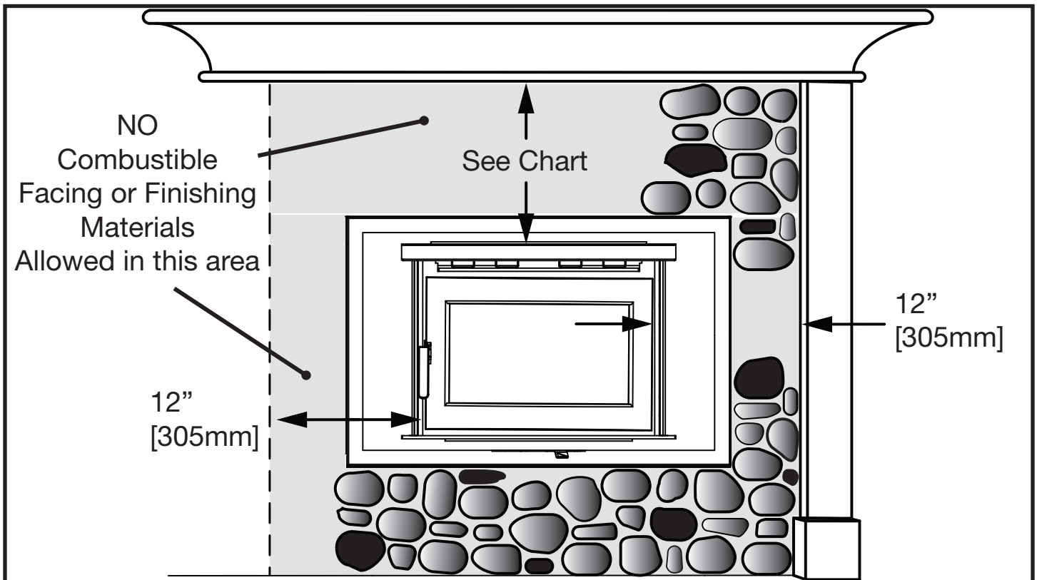
Figure 22: FP16 LE Facing Material Clearances.
