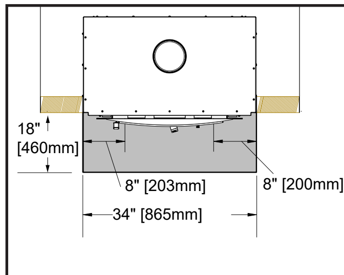
Figure 19: FP16 LE Ember Protection.
