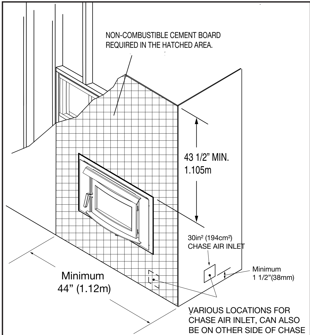
Figure 20: FP16 LE Facing and air inlets..
