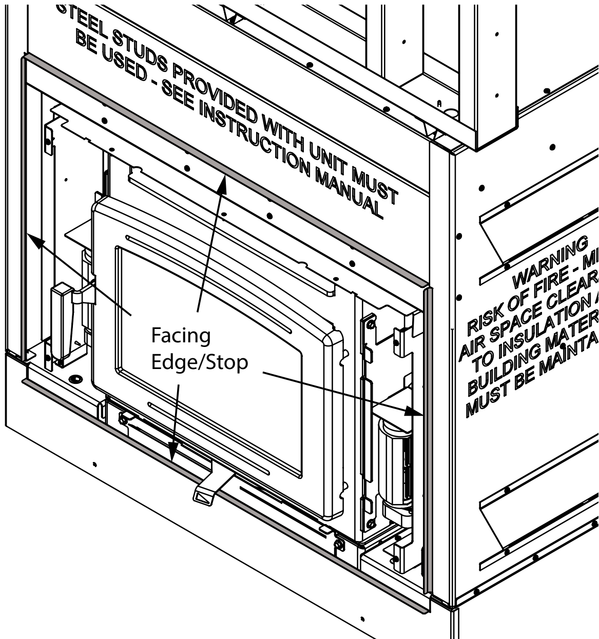
Figure 21: FP16 LE, Facing edge.
