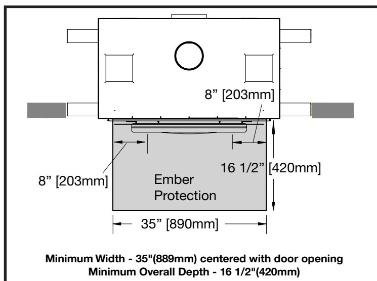
Figure 18: FP25LE Ember protection US.
