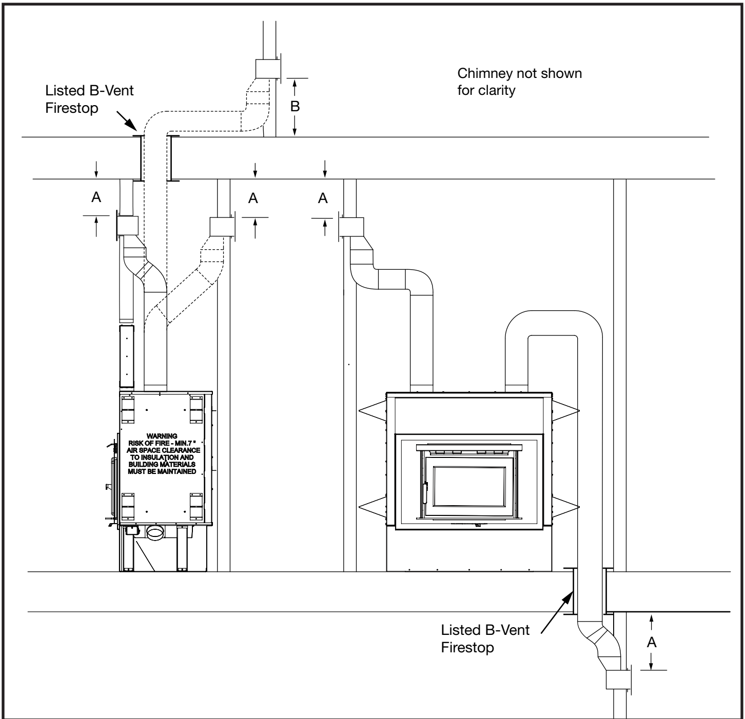
Figure 19: FP25LE Remote heat duct Options.
