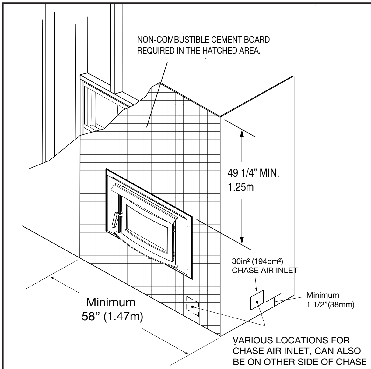
Figure 28: FP25LE Facing and air inlets.
