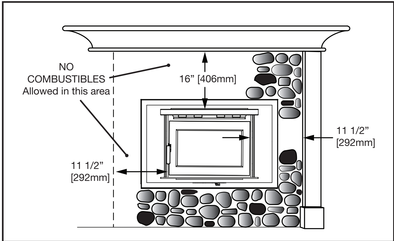
Figure 29: FP25LE Mantle and Pillar.
