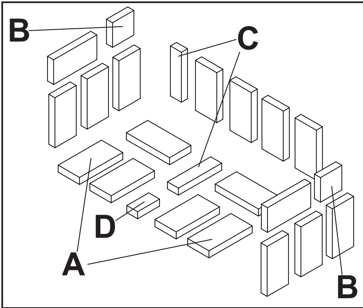
Figure 30: FP25LE Firebrick layout.
