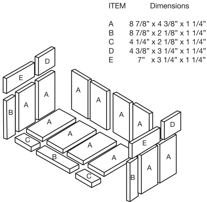
Figure 11: Vista Insert LE - Firebrick layout.
