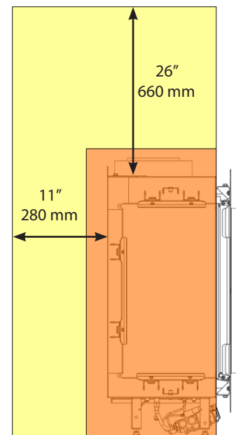
Figure 12 Side Elevation View - Bidore 140
