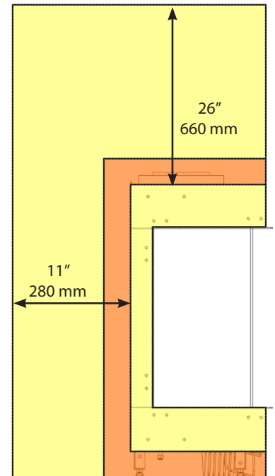
Figure 15 Side Elevation View - Trisore 140
