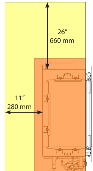
Figure 9 Side Elevation View - Modore 140
