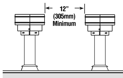
Figure 24 Multiple Termination Clearance
