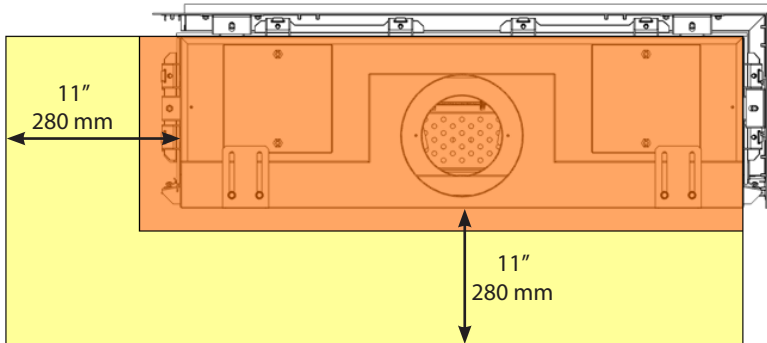
Figure 10 Plan View - Bidore 140
