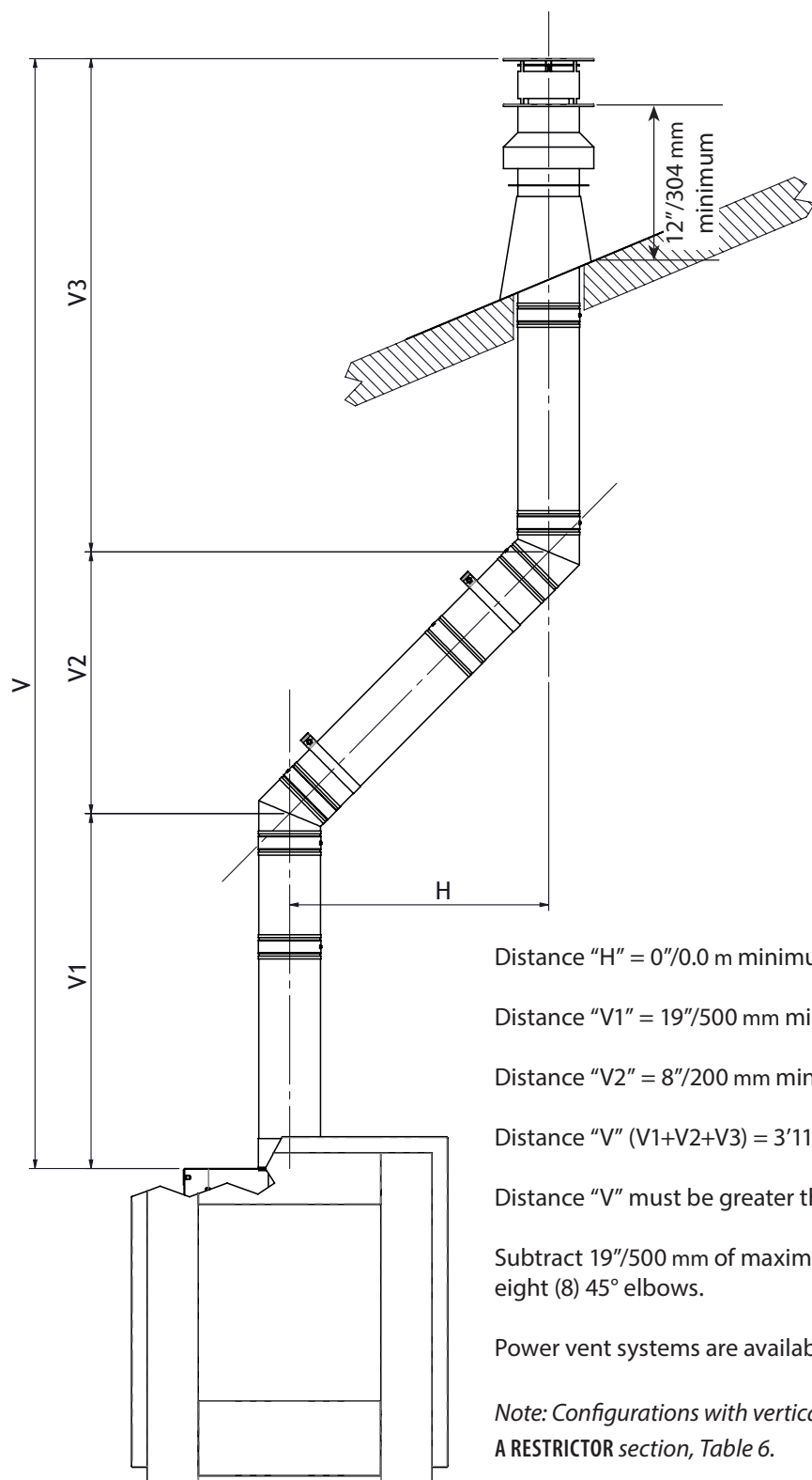
Figure 23 Vertical Terminations with 45° elbows
