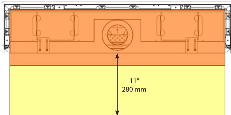
Figure 13 Plan View - Trisore 140
