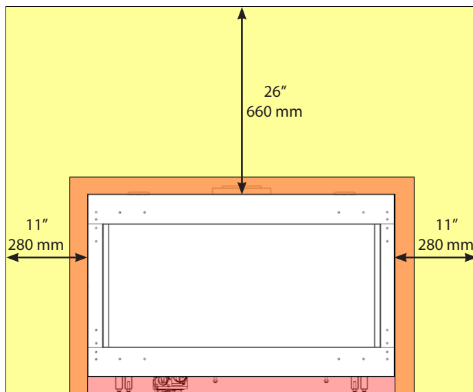
Figure 8 Front Elevation View - Modore 140
