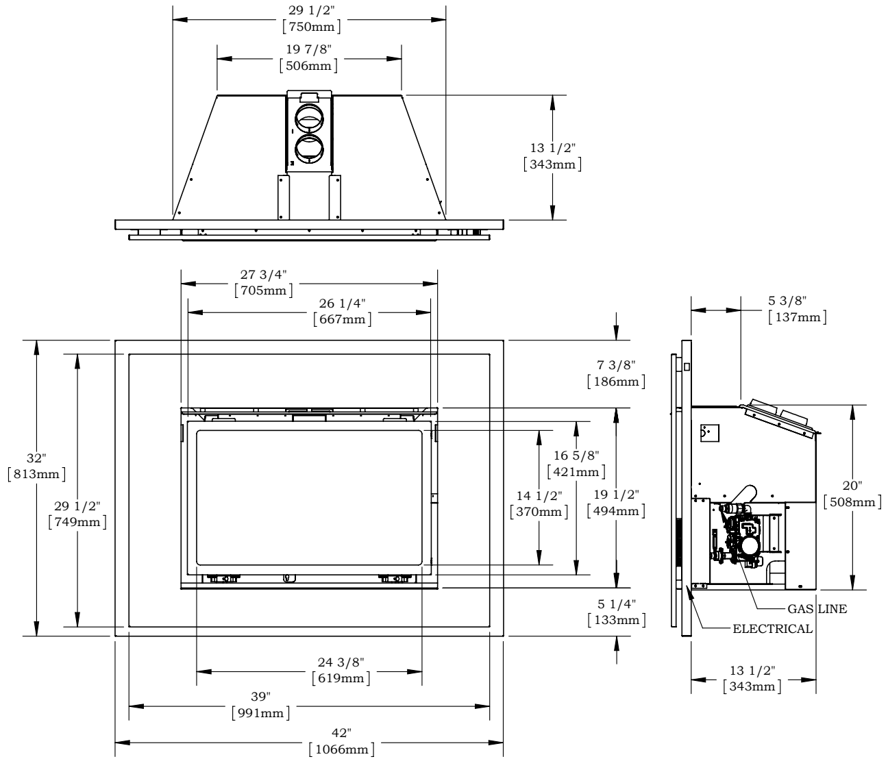
Figure 6 Sec.1 30DFID-S four-sided trim dimensions (Tolerance \pm 1/8" [1.25 mm])
