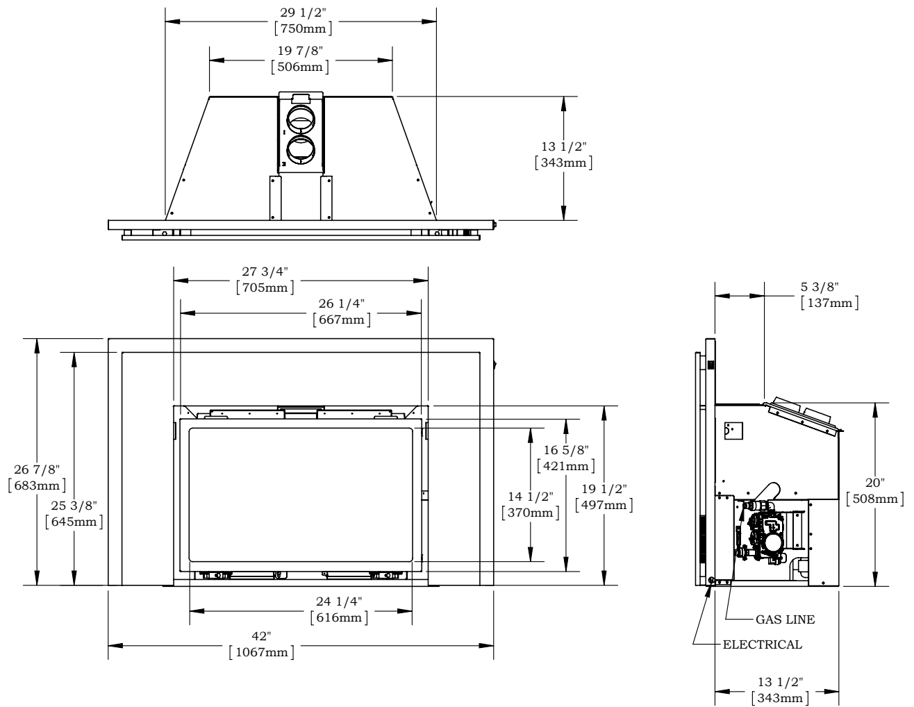
Figure 3 Sec.1 30DFID-S standard trim dimensions (Tolerance \pm 1/8" ) [1.25 mm]
