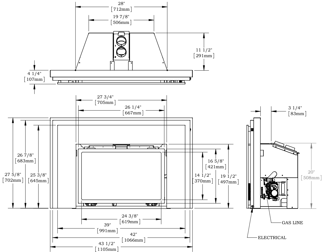
Figure 4 Sec.1 30DFID-S offset trim dimensions (Tolerance \pm 1/8" ) [1.25 mm]
