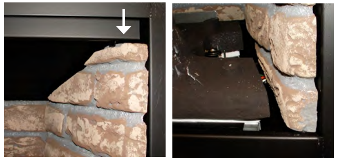
Figure 5 Sec.9 Retainer detail Top and Bottom
