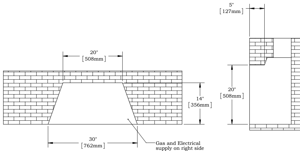
Figure 1 Sec.2 30DFID-S installation dimensions (standard trim)
