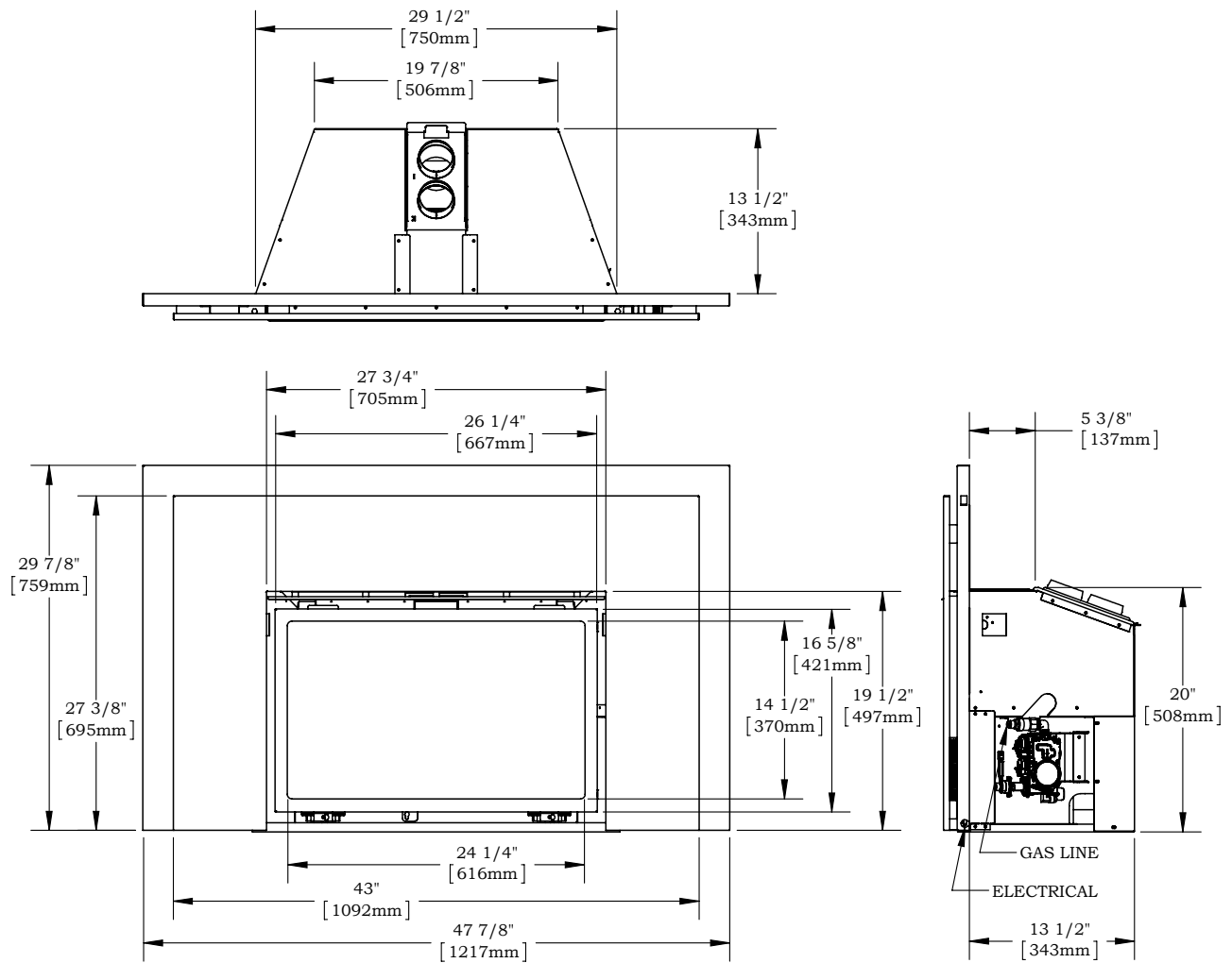
Figure 5 Sec.1 30DFID-S oversized trim dimensions (Tolerance \pm 1/8" ) [1.25 mm]
