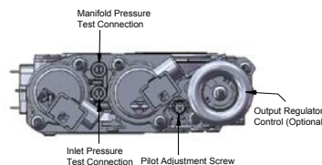
Gas Valve
