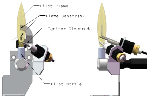
Figure 3 Sec.10 Showing the approximate size of a pilot flame
