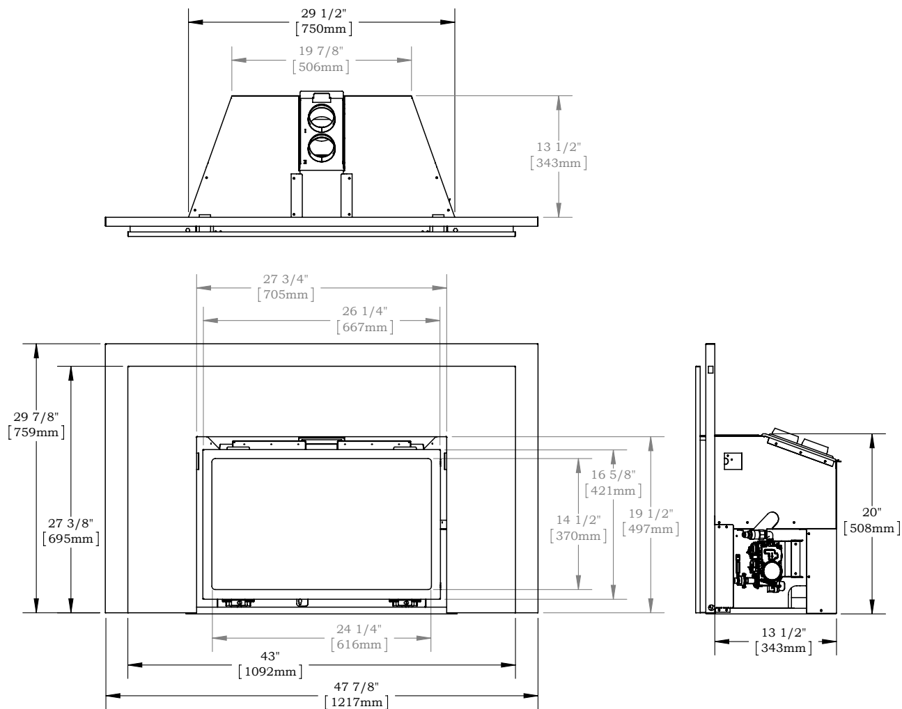
Figure 4 Sec.1 30DFID-L oversized trim dimensions (Tolerance \pm \frac{1}{8} " [1.25 mm])
