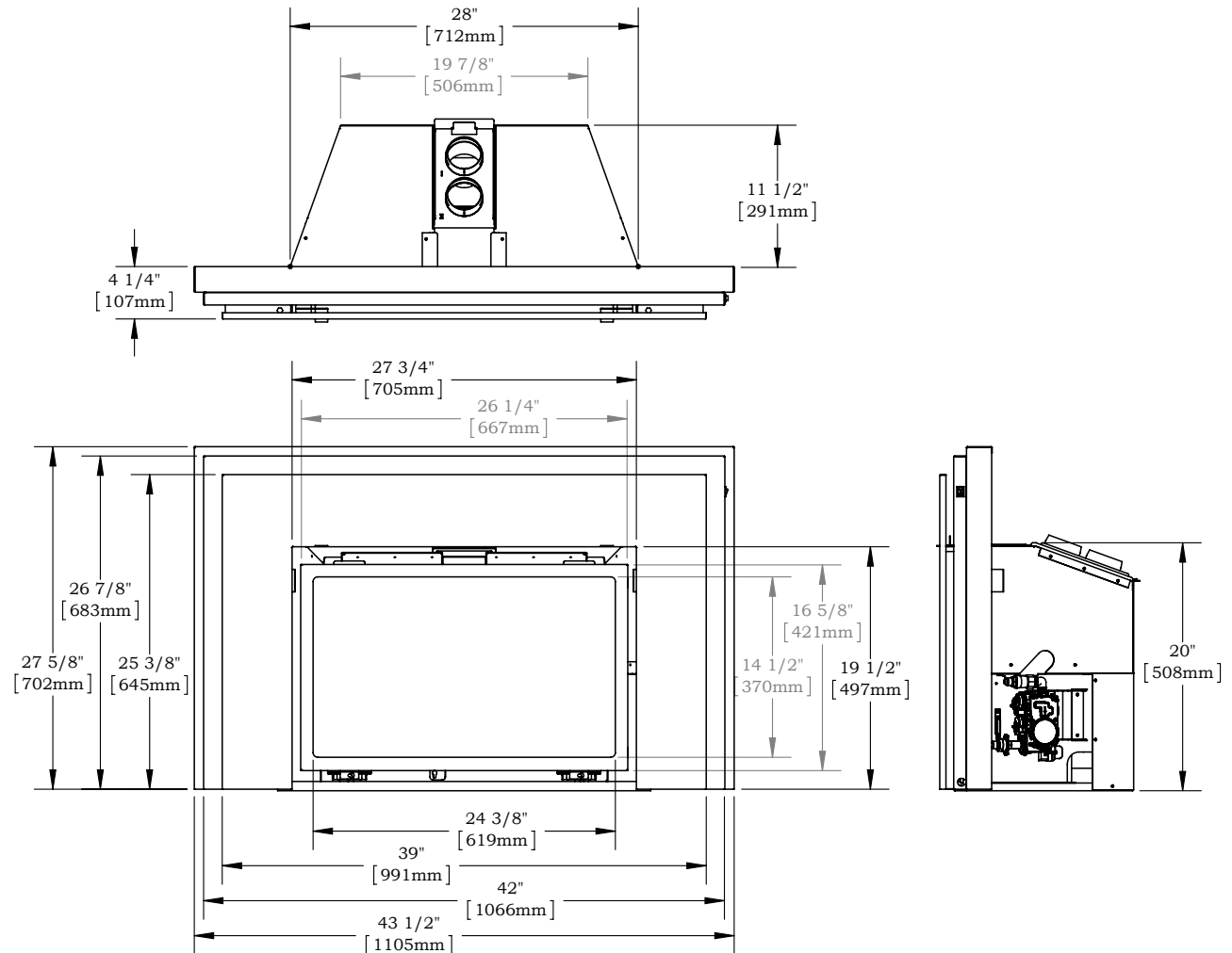
Figure 3 Sec.1 30DFID-L offset trim dimensions (Tolerance \pm \frac{1}{8} " [1.25 mm])
