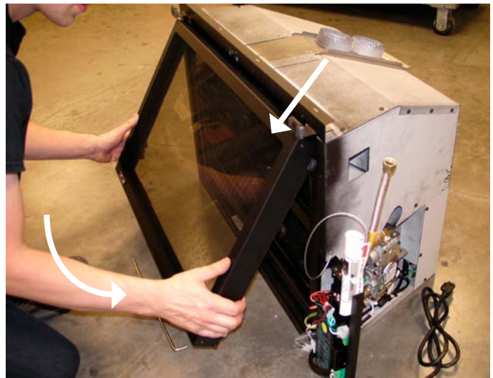
Figure 8 Sec.4 Swing the Door away from the unit, lift over the retaining tabs on top of the firebox. Be careful to not roll the gasket up off the glass when reinstalling the door.
