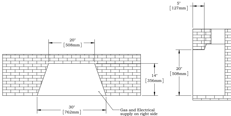
Figure 1 Sec.2 30DFID-L installation dimensions
