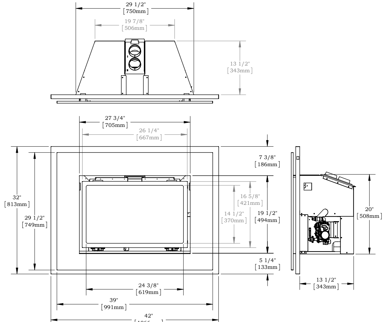
Figure 5 Sec.1 30DFID-L four-sided trim dimensions (Tolerance \pm \frac{1}{16} " [1.25 mm])
