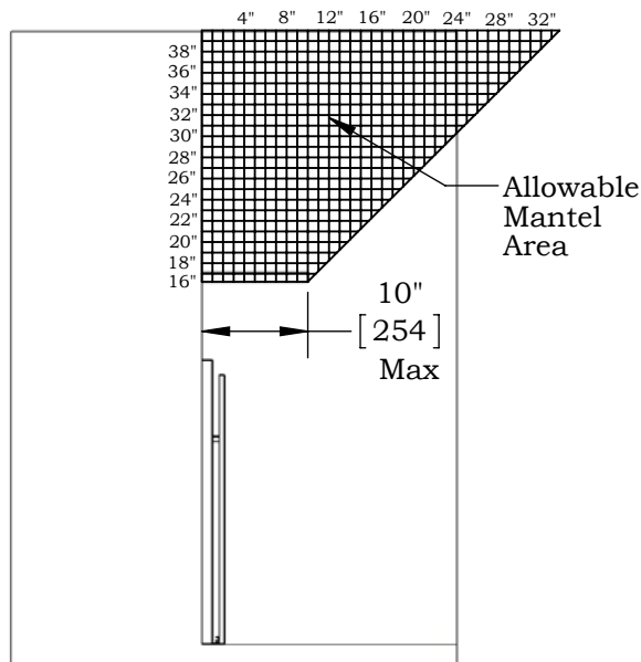
Figure 3 Sec.2 30DFID-L mantel clearances
