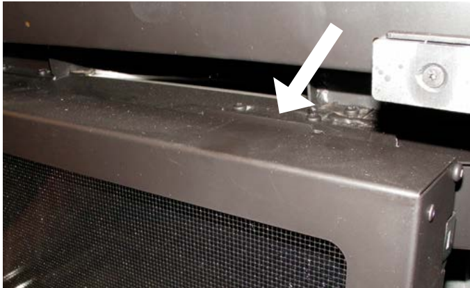
Figure 9 Sec.4 Location of Door retainer tabs
