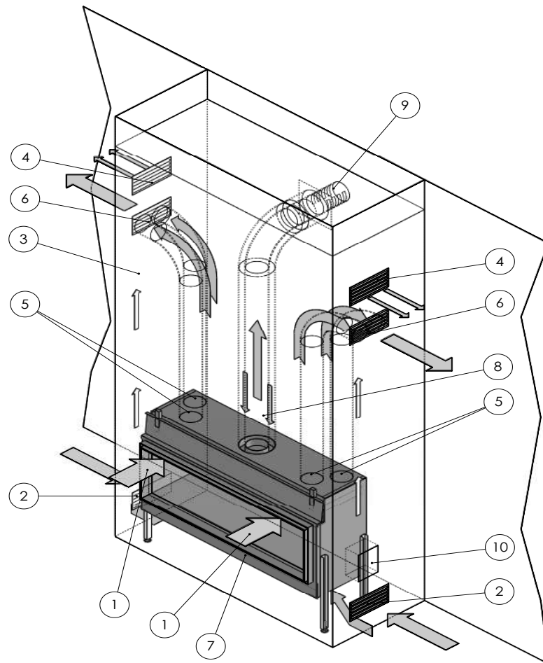
Figure 12: Appliance installed in ventilated chimney breast Horizontal outlet of the flue gas exhaust /combustion air supply via the wall. Fitted with the options / accessories: • convection package (= convection casing and 1x convection set) • 1x extra convection set • high adjustable feet
