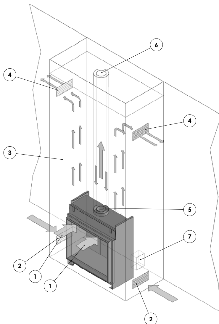
Figure 13: Appliance installed in ventilated chimney breast Vertical outlet of the flue gas exhaust / combustion air supply via the roof. Fitted without convection package
