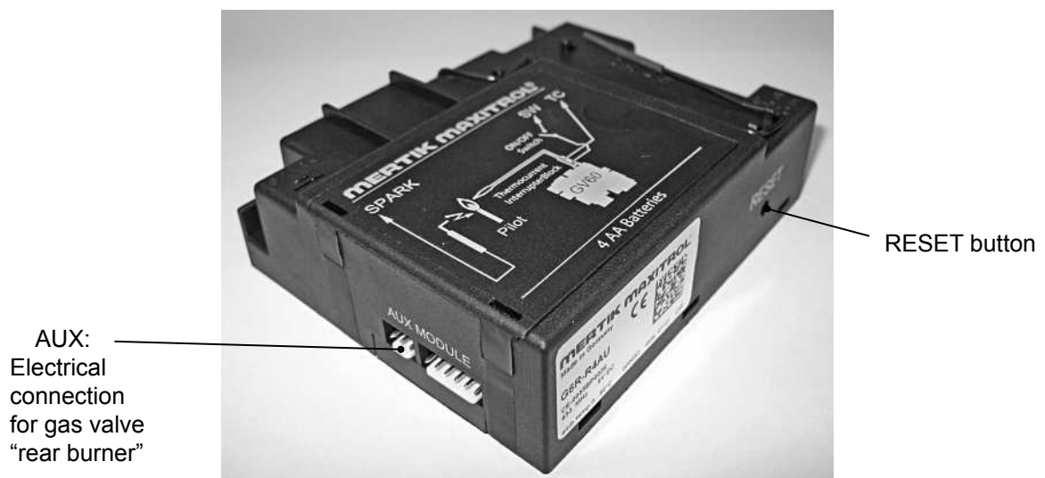
Figure 19: Receiver - AUX connection - RESET button
