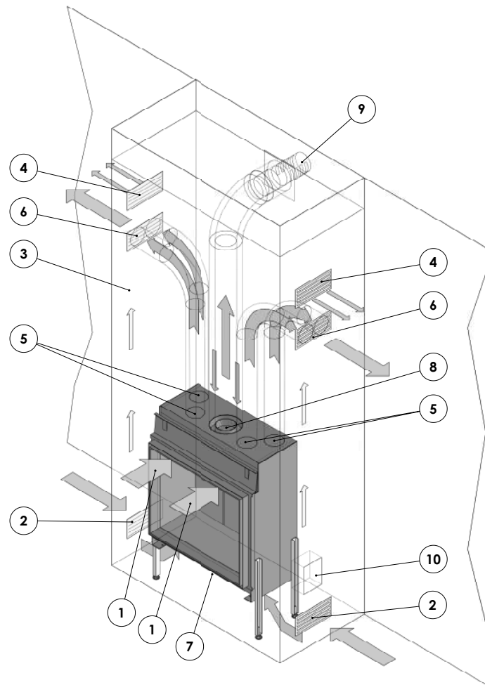
Figure 12: Appliance installed in ventilated chimney breast Horizontal outlet of the flue gas exhaust /combustion air supply via the wall. Fitted with the options / accessories: • convection package (= convection casing and 1x convection set) • 1x extra convection set • high adjustable feet
