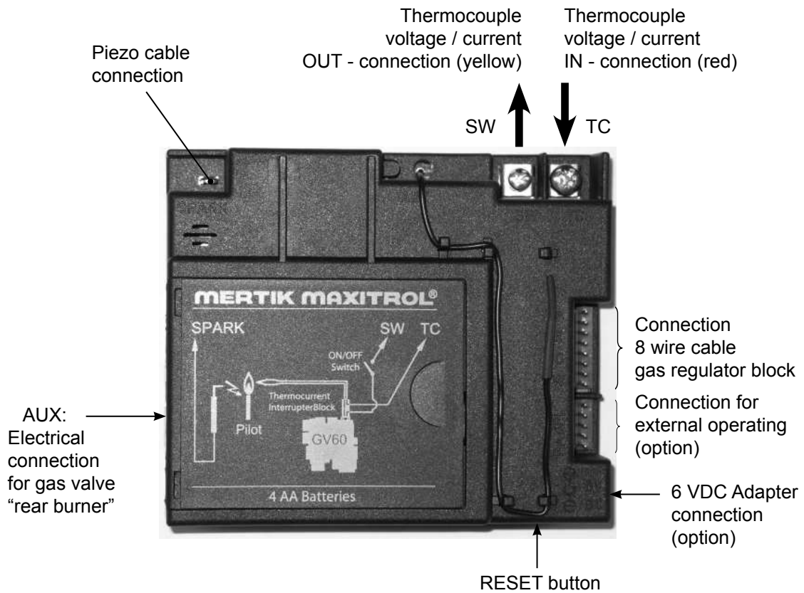
Figure 18: Receiver - Top
