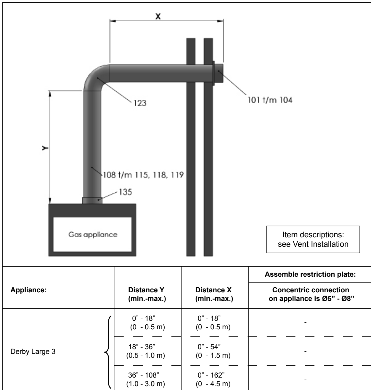
Figure 11: Horizontal wall termination
