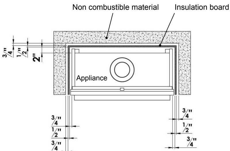
Figure 2: Clearances to non-combustible material
