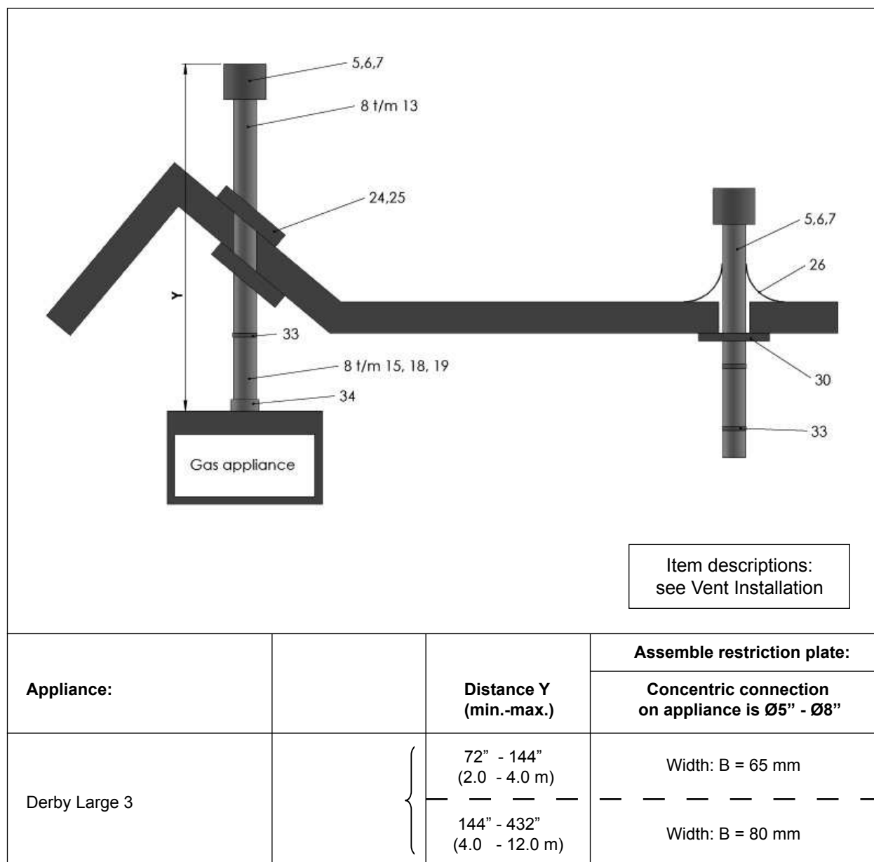
Figure 6: Vertical roof-mounted outlet without bend
